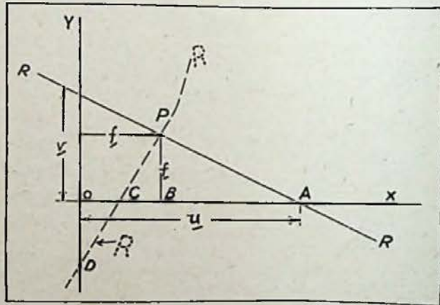
Fig. 4.—Another graphic method of solving lens problems.
