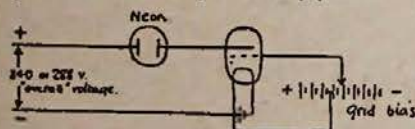
Fig 5. Circuit diagram for Valve amplification.
