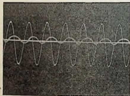
Fig. 6.—Oscilloscope record of plate current and oscillatory circuit current when coupling is tight.
