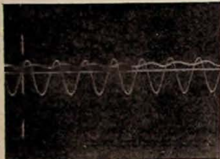
Fig. 5.—Oscilloscope record of plate current and oscillatory circuit current when valve is just oscillating.
