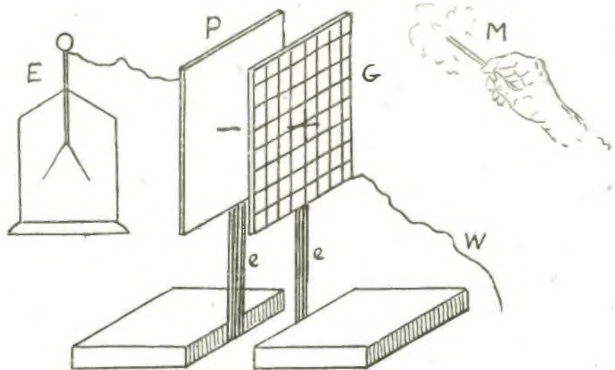
Fig. 1. An experiment illustrating the photo-electric effect. P, zinc or magnesium plate; G, wire grid; E, electroscopes; W, earth wire; M, magnesium wire burnt to produce ultra-violet; ee, ebonite pillars.
