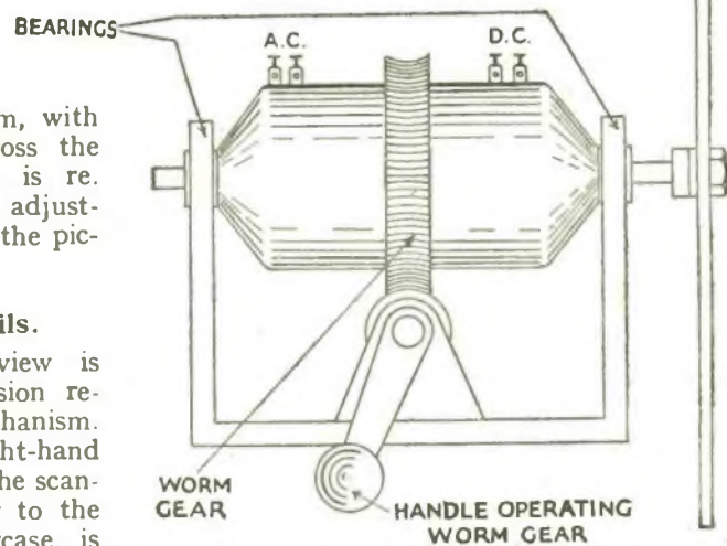
Fig. 4. Showing the operation of the worm gear for rotating the carcass of the receiver driving motor and its associated synchronous motor.
