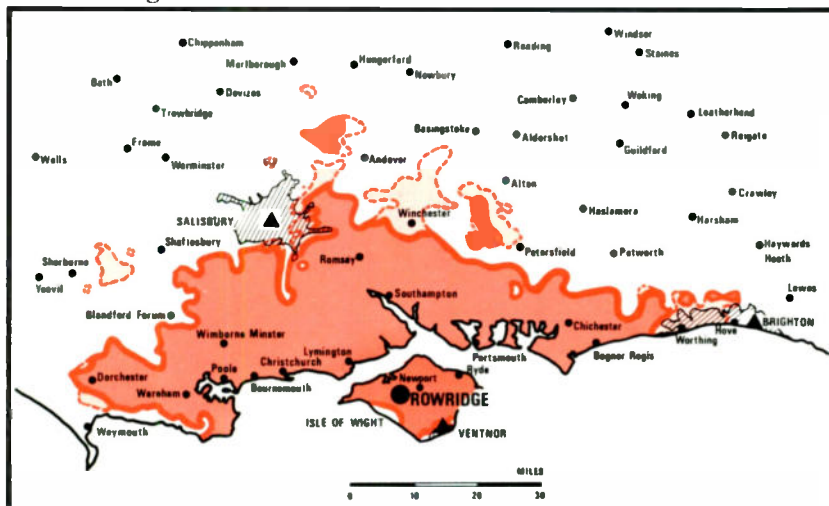
108 Rowridge UHF Main Station Ch27
