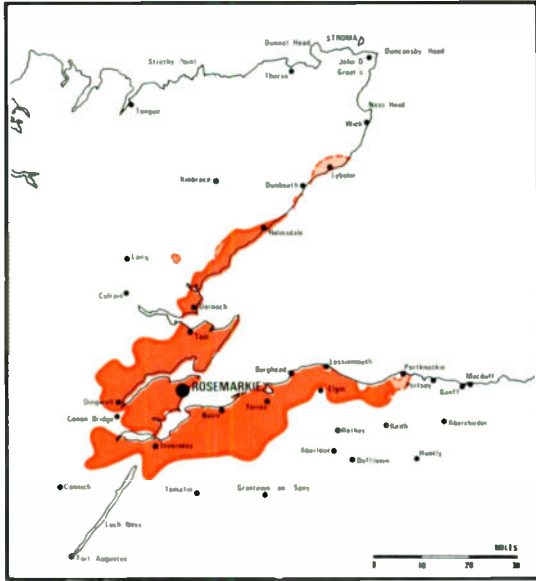
156 Rosemarkie UHF Main Station Ch49
