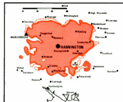
126 Hannington UHF Main Station Ch42*
