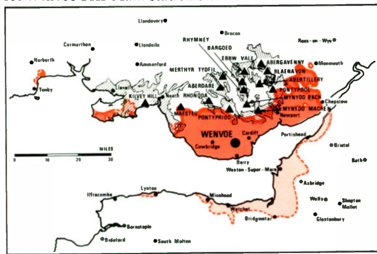
106 Wenvoe UHF Main Station Ch41
