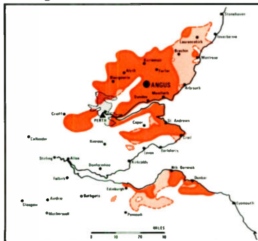
123 Angus UHF Main Station Ch60
