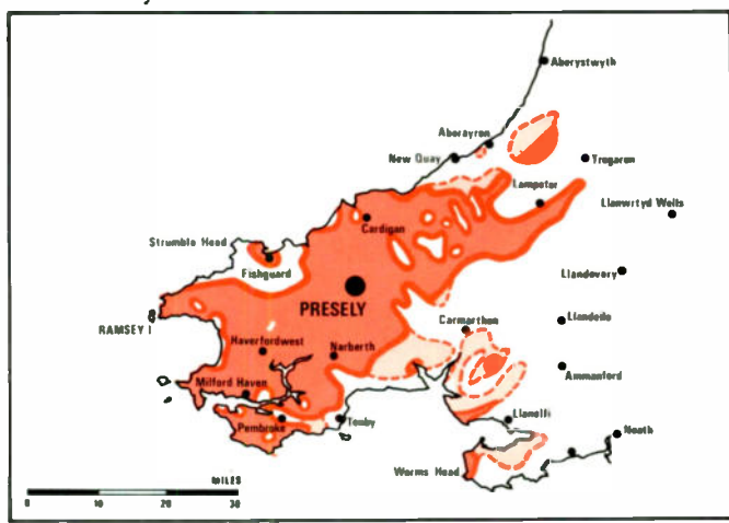
129 Presely UHF Main Station Ch43*
