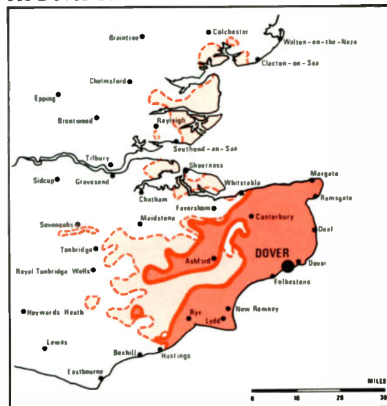
113 Dover UHF Main Station Ch66
