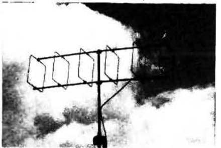
The Halbar six-element quad initially used by the author on the 144MHz band. The ribbon at the top corner of the reflector, right, shows wind direction so that the beam may be turned into wind during gales and the like. A nine-over-nine element Tonna has since replaced the quad
