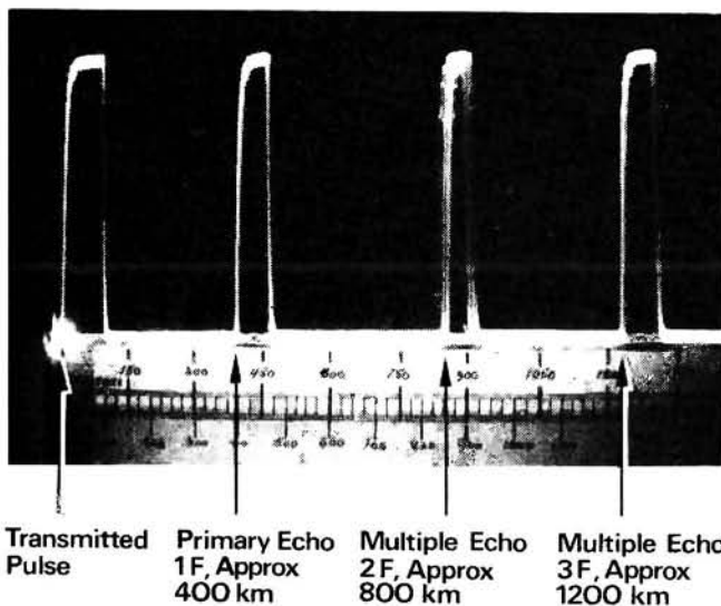
Fig. 1.6: Echoes received from the F layer using modern equipment and a c.r.t. display. Note: scale shown not aligned owing to camera angle
