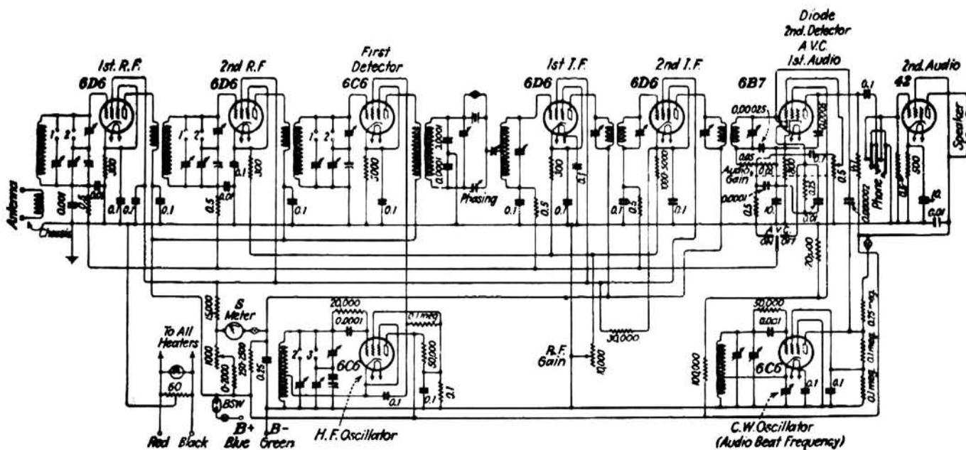
Fig. 1: Schematic diagram of the HRO receiver
