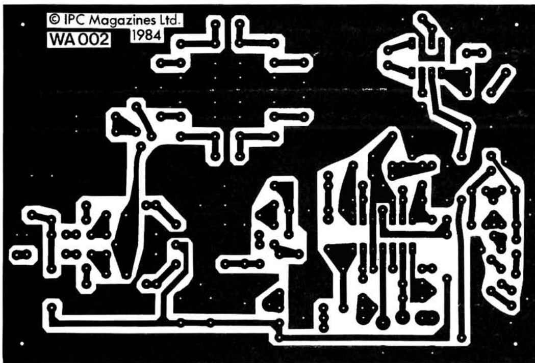
Fig. 3.3.: Full size p.c.b. track pattern and component layout for Module 3, the Receiver
