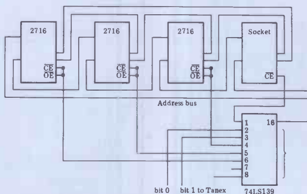
6k ROMboard circuit diagram
