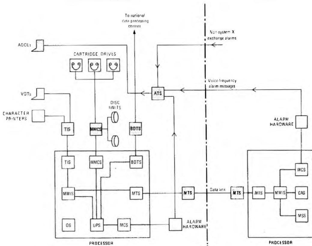
FIG. 1—Block diagram of local administration centre
