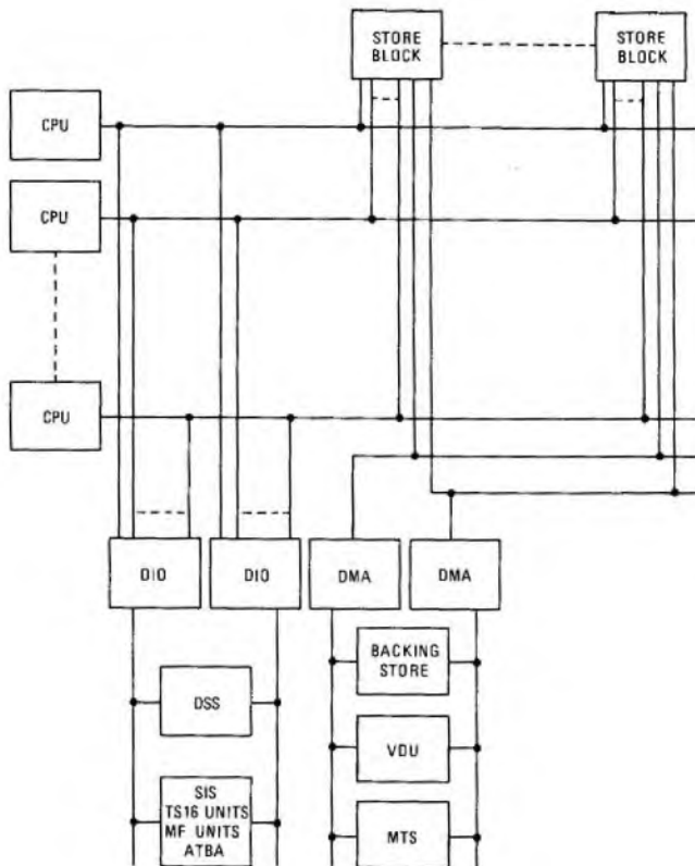
FIG. 7—Block diagram of processor
