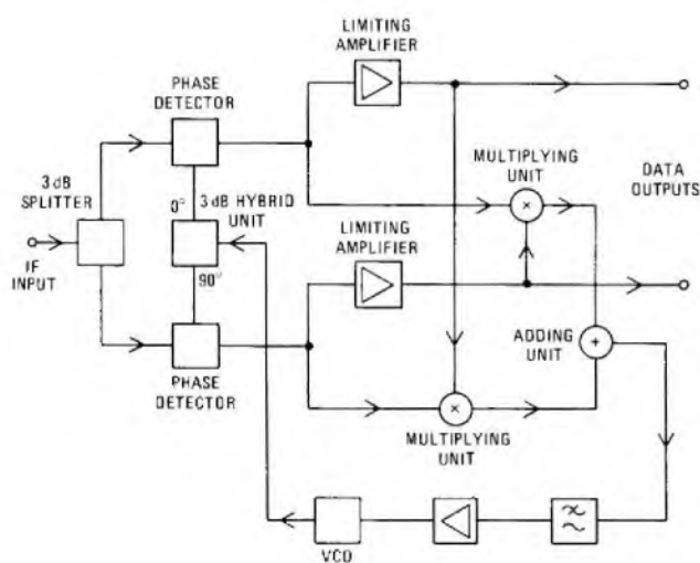
Fig. 11—Block diagram of a baseband remodulation-type demodulator
