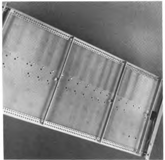
FIG. 10—Rear view of 8-unit shelf showing backplane and stiffeners
