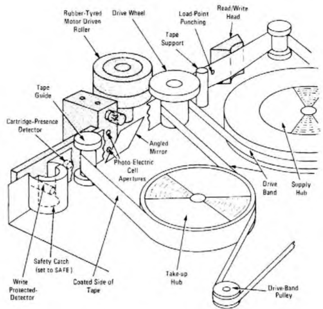
FIG. 4—Cartridge and Recorder Tape No. 3A interface
