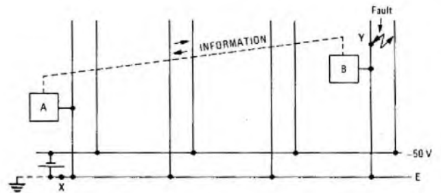
FIG. 6—Voltage-potential disturbance mechanism
