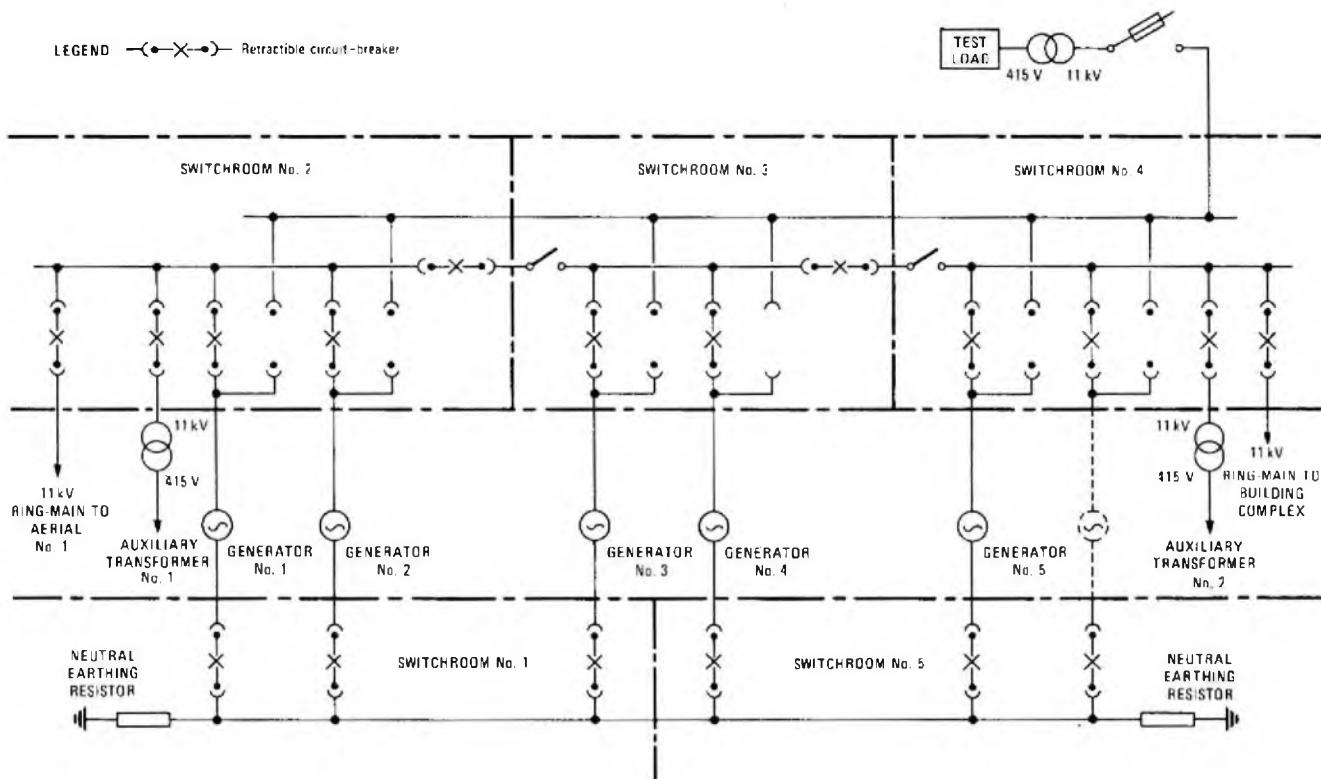
FIG. 6—High-voltage switchboard
