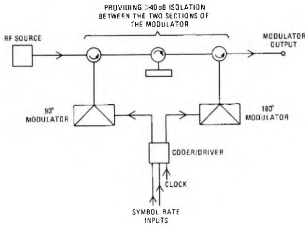
FIG. 9—Block diagram of an RF modulator
