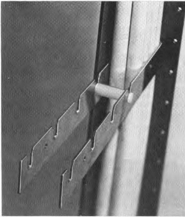
FIG. 5—Cable-compartment fitting
