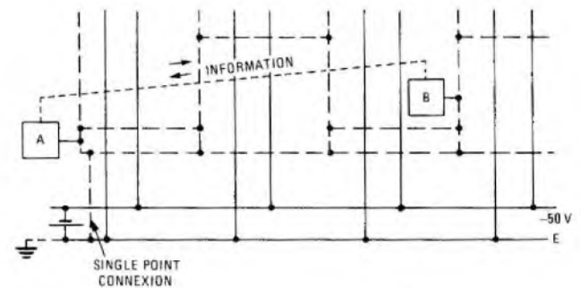
FIG. 7—Electronic-earth circuit configuration
