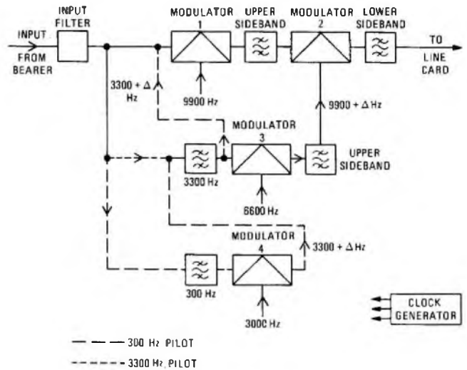
FIG. 9—Block diagram of the GEC Telecommunications Ltd. frequency correction unit
