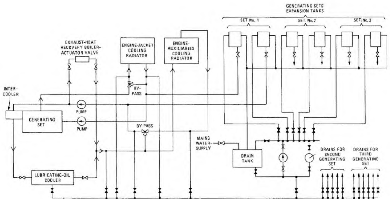
FIG. 4—Water-cooling system
