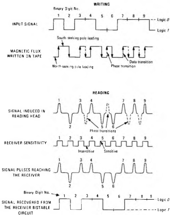
FIG. 1—Phase-encoding format
