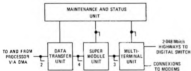
FIG. 6—Block diagram of the message transmission subsystem hardware
