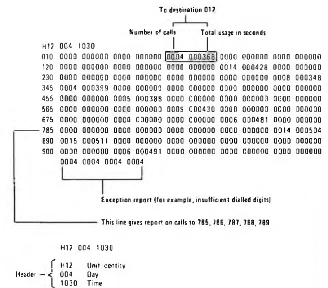
FIG. 4—A typical output of a call-destination analysis program (1000-destination matrix)
