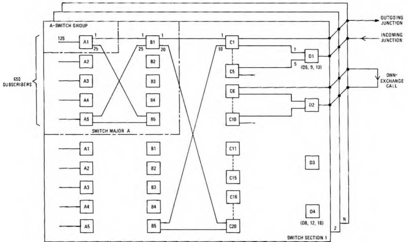
FIG. 4—Switch network, comprising 1-N switch sections (as employed at Werrington, where N = 6 )
