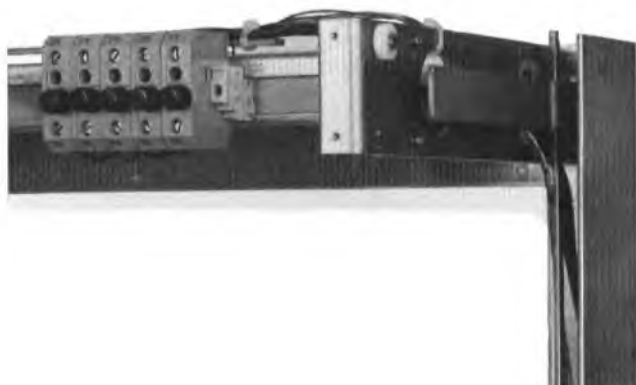
FIG. 4—Rack-top fuse mounting
