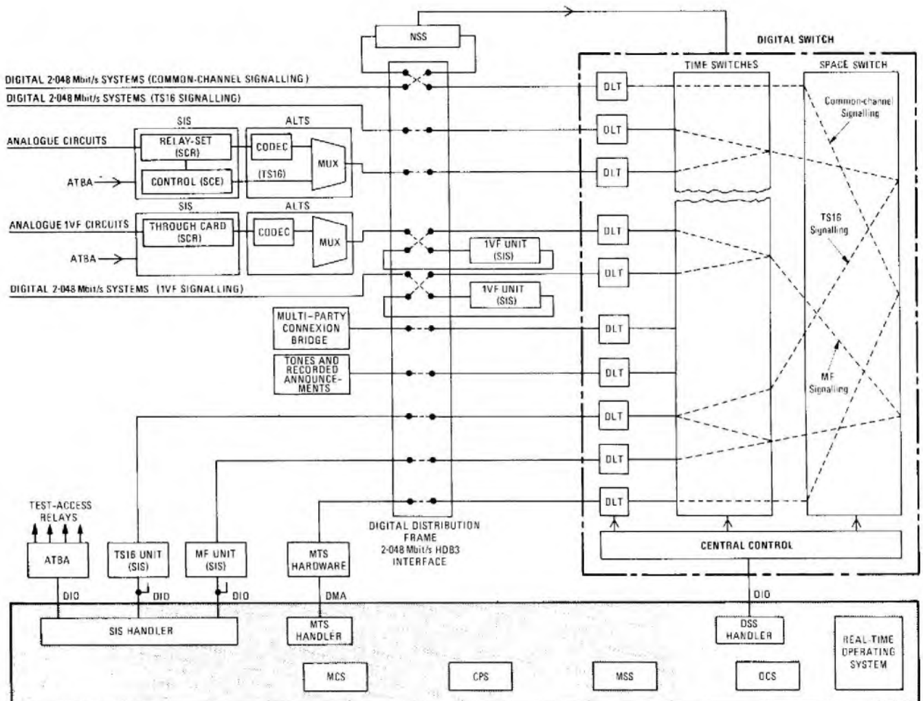
FIG. 2—Block diagram of a digital main-network switching system
