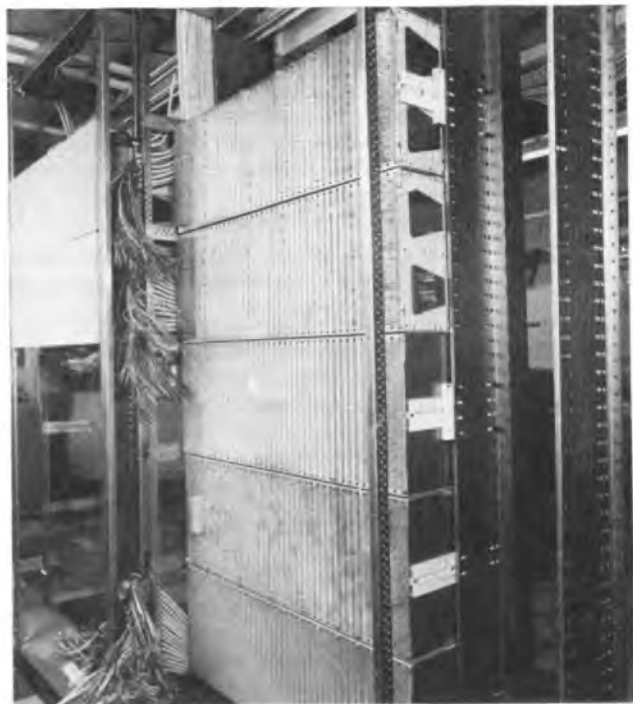
FIG. 8—Prototype System-X equipment rack
