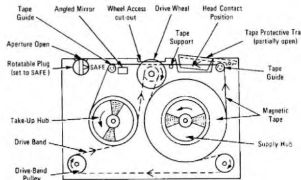
FIG. 3—Data tape-cartridge
