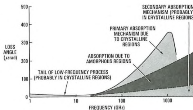
FIG. 6—Analysis of the polypropylene structure
