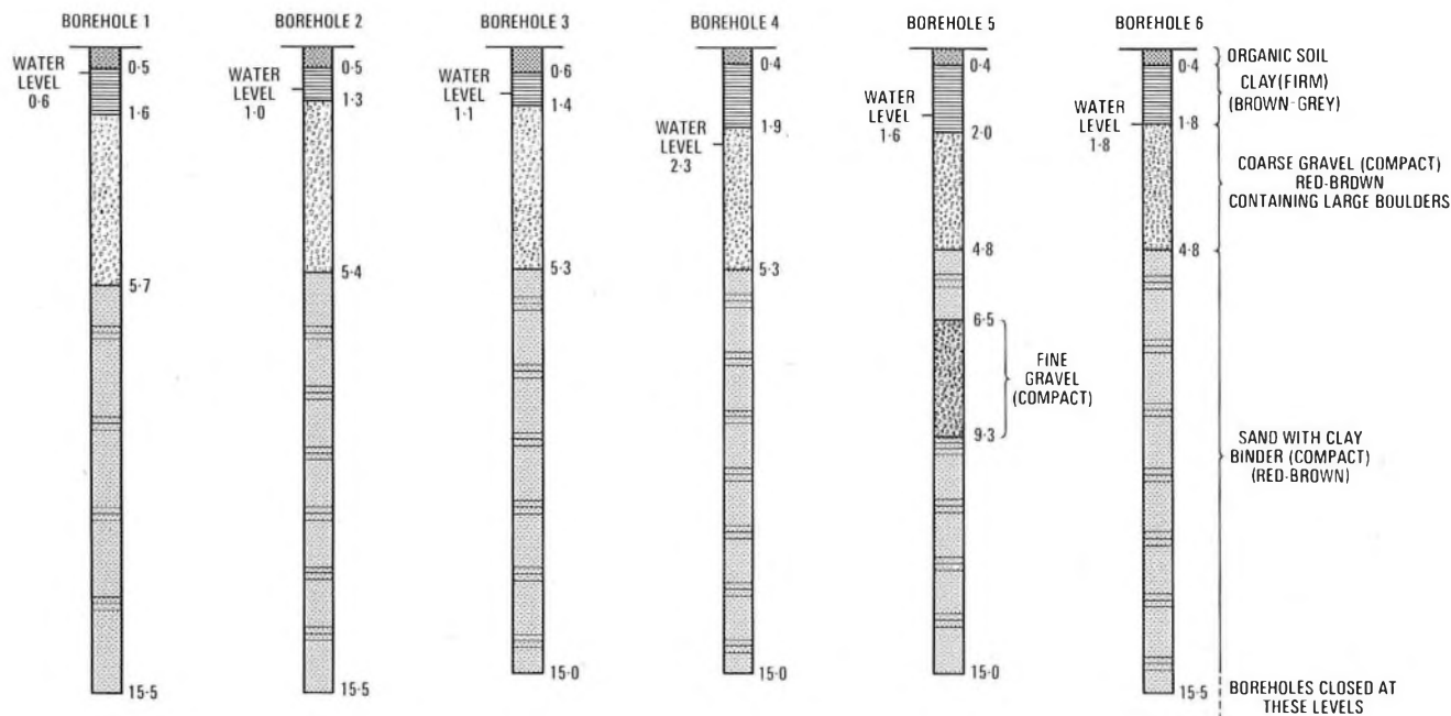
All depths in metres FIG. 11—Ground strata in trial boreholes
