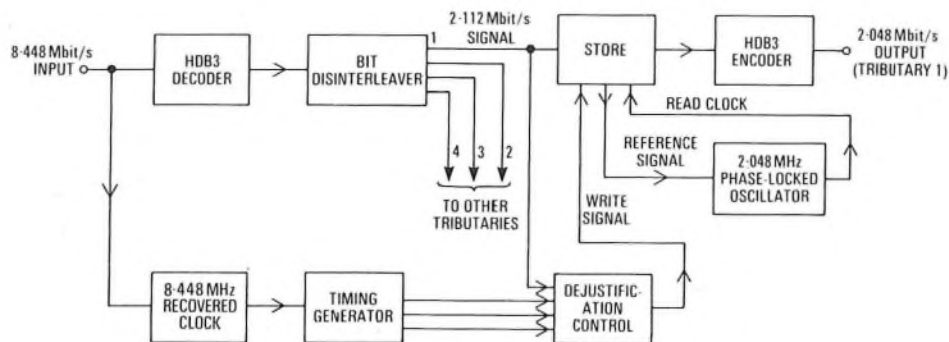
FIG. 3—Block diagram of 8.448 Mbit/s-2.048 Mbit/s demultiplexing equipment
