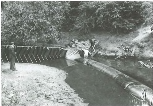
FIG. 2—Erection of the portable dam
