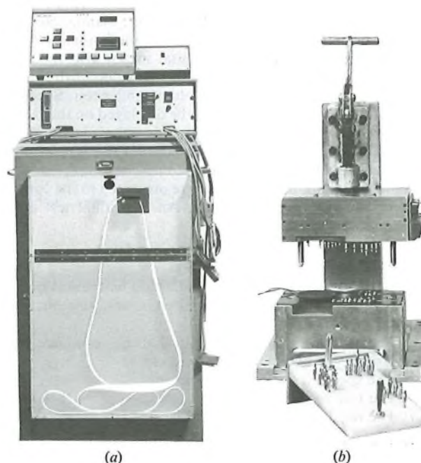
(a) PAT 2 (b) Bed-of-nails jig, showing interchangeable probe-assembly inserts
