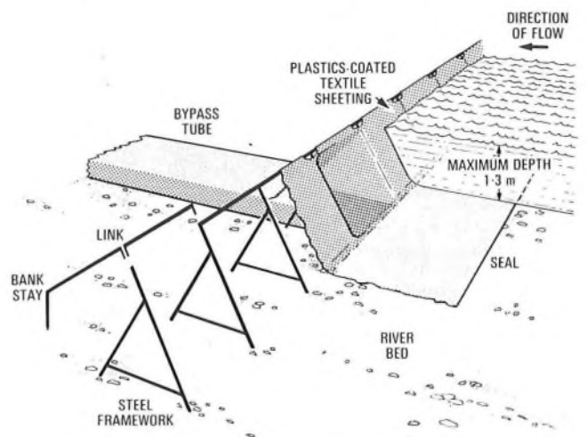
FIG. 1—Principle of the portable dam
