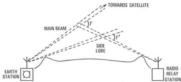
FIG. 8—Tropospheric forward scatter
