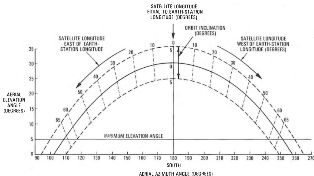
FIG. 1—Aerial azimuth and elevation angles for a latitude of around 52° when operating to geostationary satellites
