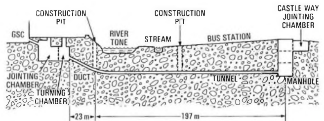
FIG. 2—Section along the line of the tunnel
