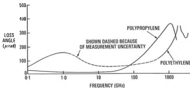
FIG. 5—Dielectric-loss-angle/frequency spectra of polyethylene and polypropylene
