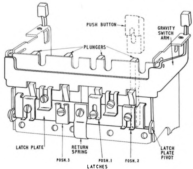
FIG. 2—LATCH-PLATE MECHANISM
