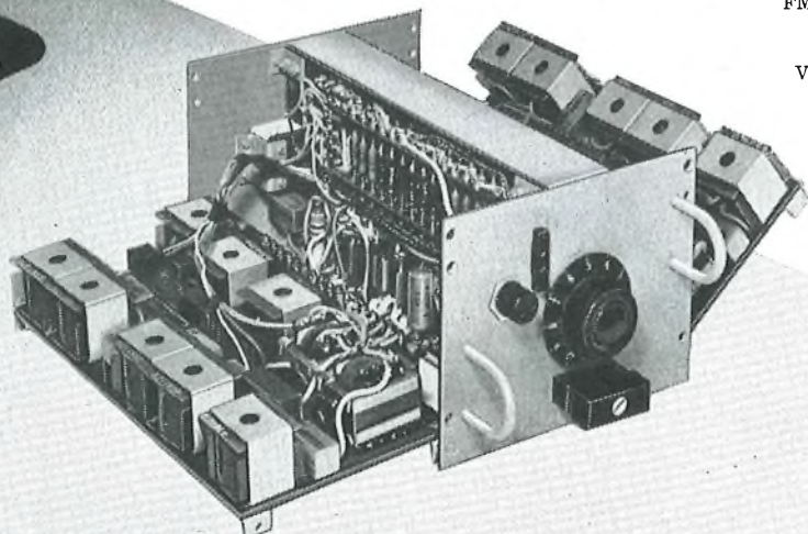
Channel Unit
