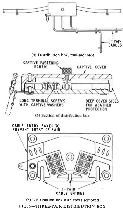
FIG. 5—THREE-PAIR DISTRIBUTION BOX
