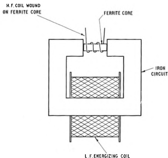
FIG. 3—ARRANGEMENT OF FERRITE MODULATOR
