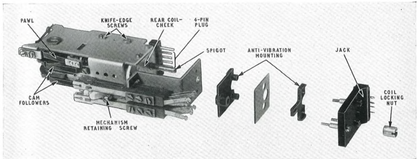
FIG. 4—MOUNTING DETAILS
