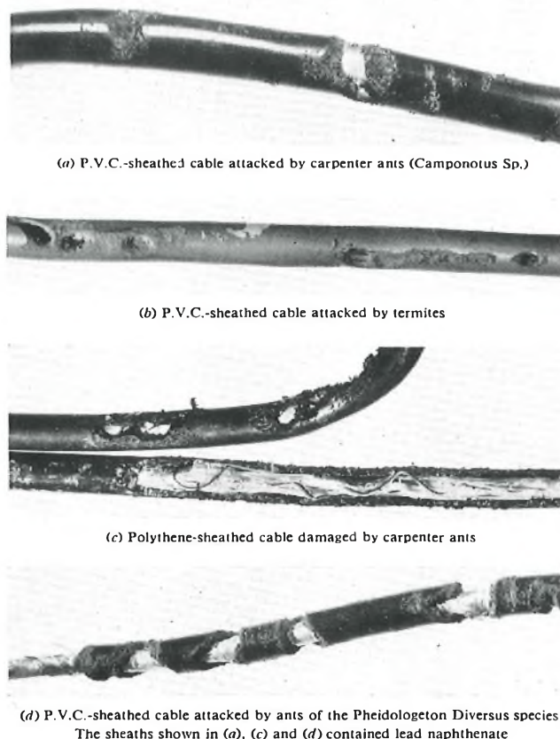
FIG. 6—EFFECTS OF INSECT ATTACKS ON PLASTIC-SHEATHED CABLES
