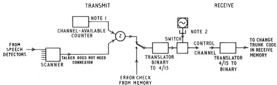
FIG. 5—SIMPLIFIED BLOCK SCHEMATIC DIAGRAM OF MAIN DISCONNECTION AND ERROR-CORRECTION CIRCUITS
