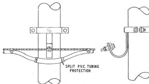
FIG. 2—AERIAL-CABLE SUSPENSION FROM STEEL POLES
