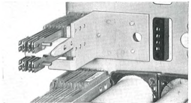
FIG. 6—SPRING-SETS WITH MECHANISM REMOVED
