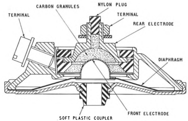
FIG. 3—CROSS-SECTION OF TRANSMITTER
