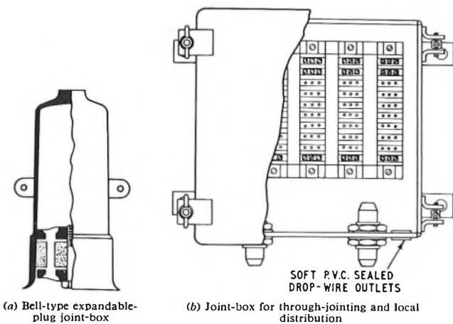
FIG. 4—JOINTING AND DISTRIBUTION BOXES
