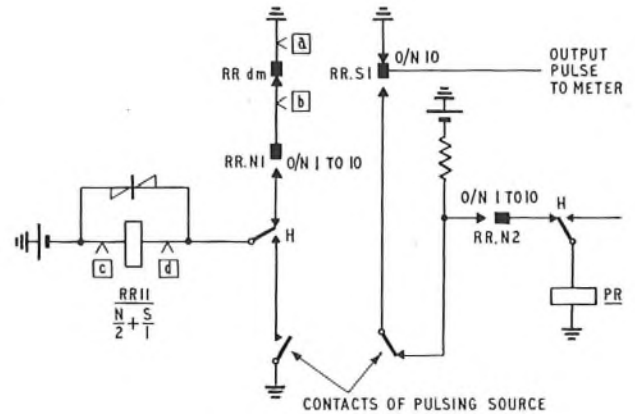
FIG. 2—TYPICAL CIRCUIT ELEMENT
