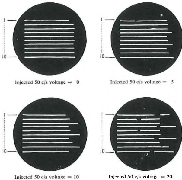
Each oscillogram shows a train of 10 pulses (digit "0") FIG. 1—DISTORTION AND SPLITTING OF LOOP/DISCONNECT PULSES DUE TO 50 c/s INDUCTION
