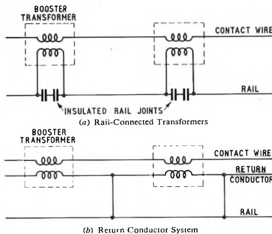
FIG. 4—METHOD OF CONNECTING BOOSTER TRANSFORMERS
