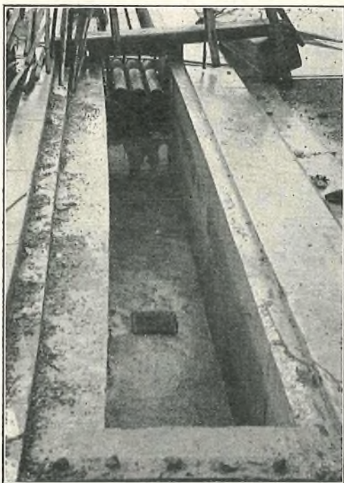
FIG. 11.—JOINTING CHAMBER IN ABUTMENT.
