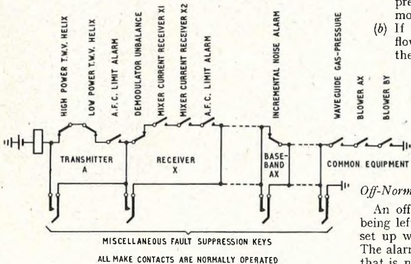
FIG. 34.—BRAEWYNNER MISCELLANEOUS-FAULTS CHAIN (SIMPLIFIED).
