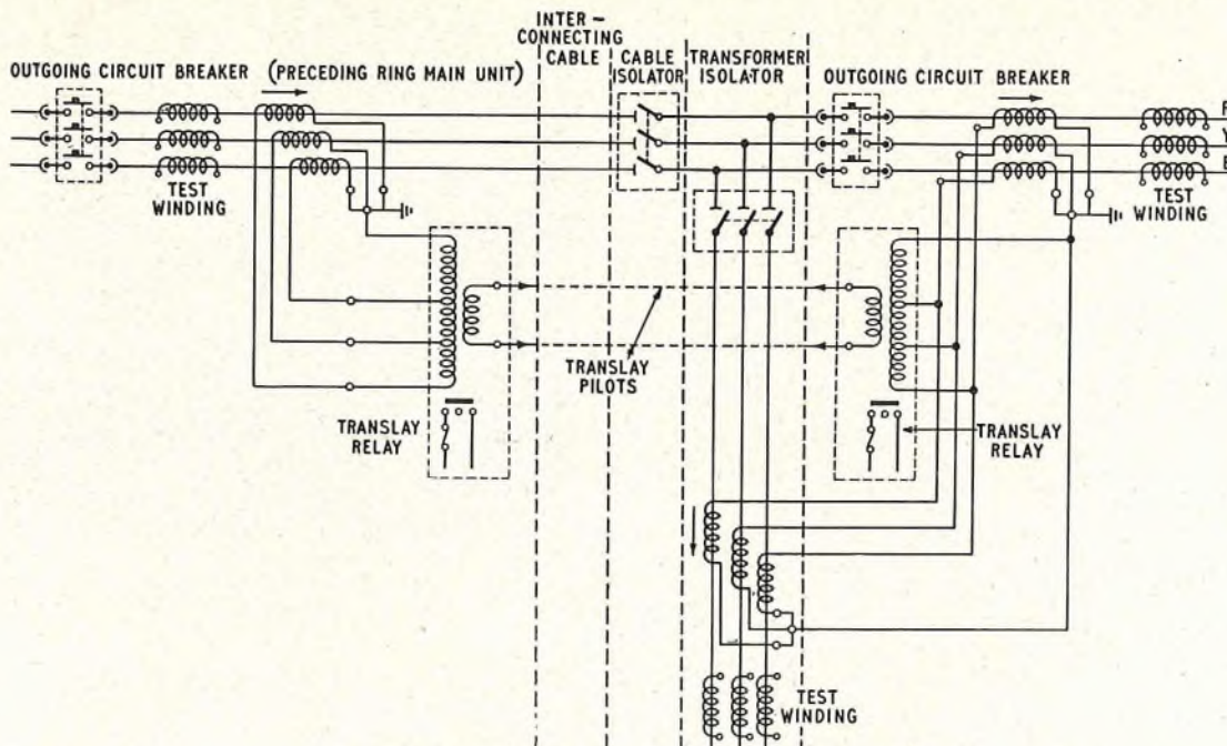
FIG. 4.—"Translay" AS APPLIED TO A TEED CIRCUIT.
