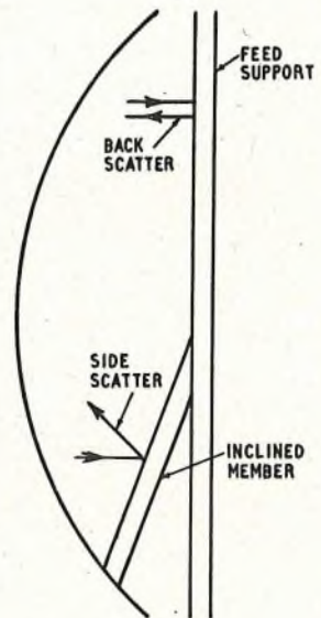
FIG. 6.—OBSTRUCTION BY FEED SUPPORT MEMBERS.
