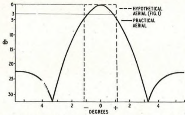
FIG. 2.—RADIATION DIAGRAMS OF HYPOTHETICAL AND PRACTICAL AERIELS.
