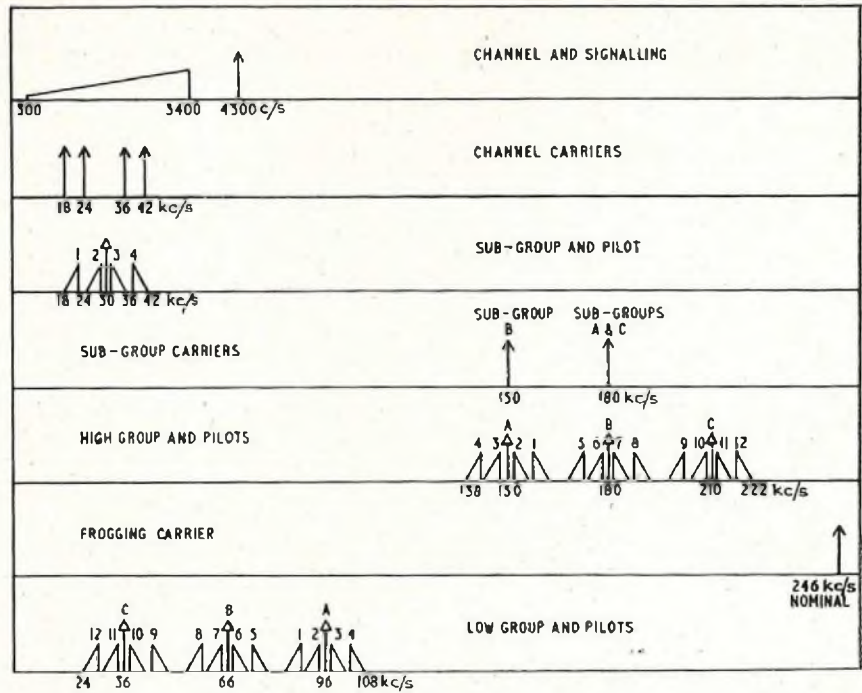
FIG. 3.—FREQUENCY ALLOCATION.
