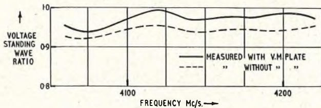
FIG. 17.—EFFECT OF VERTEX MATCHING PLATE.
