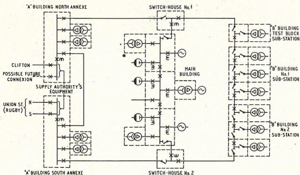
FIG. 1.—SCHEMATIC CIRCUIT ARRANGEMENT OF HIGH-VOLTAGE DISTRIBUTION.
