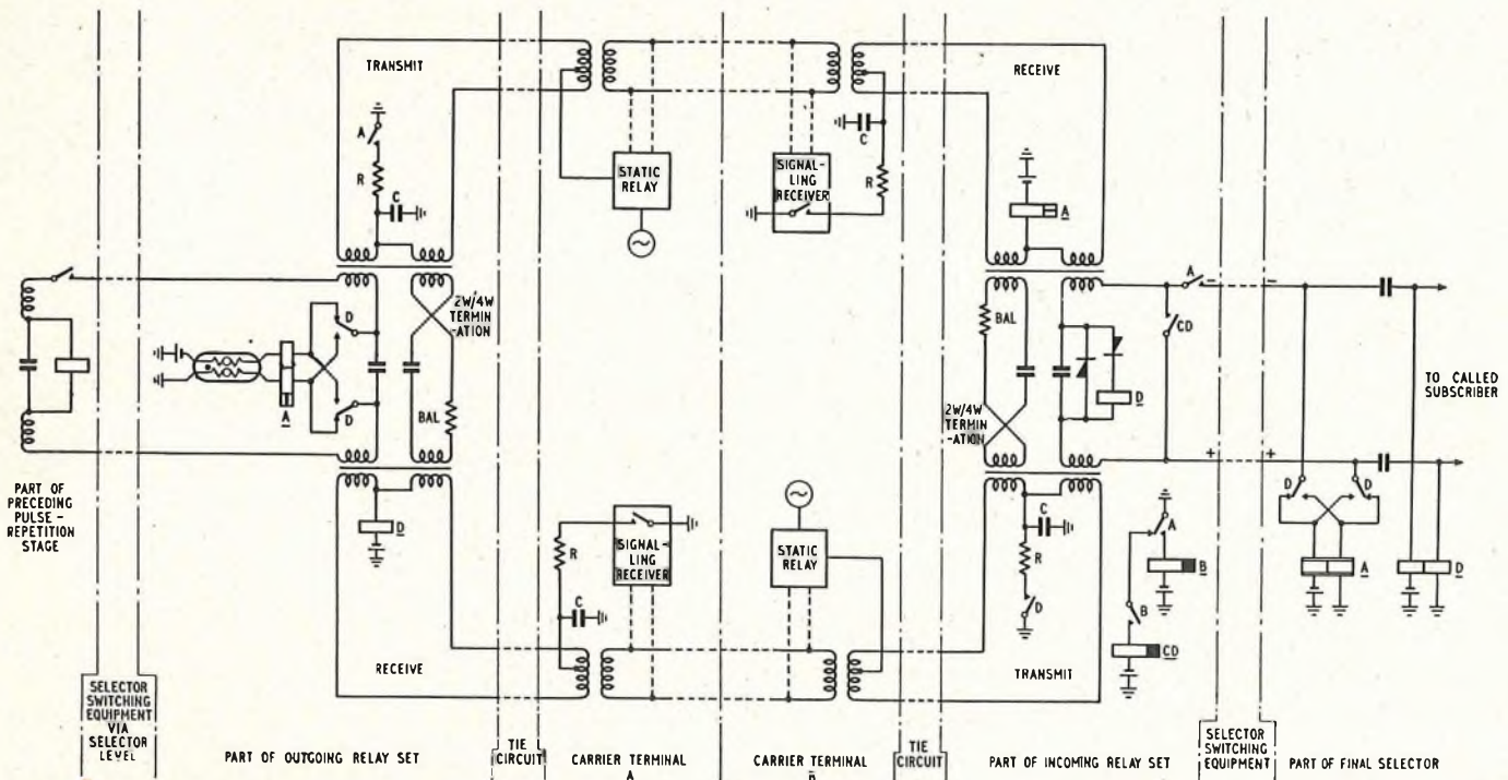
FIG. 5.—SIGNALLING ARRANGEMENTS.
