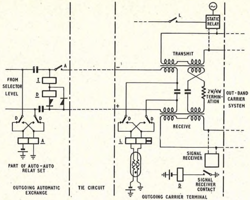
FIG. 11.—ARRANGEMENTS REQUIRED AT OUTGOING CARRIER TERMINAL TO PROVIDE DIALLING FACILITIES WITH LEVEL ACCESS FROM AN AUTOMATIC EXCHANGE.
