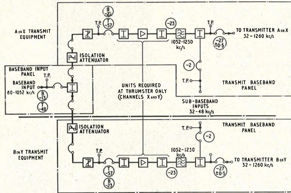
FIG. 30.—BASEBAND EQUIPMENT FOR TRANSMITTERS.
