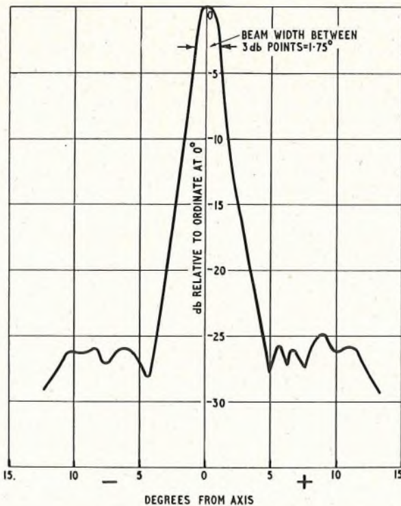
FIG. 14.—E-PLANE RADIATION PATTERN.
