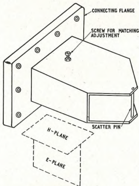
FIG. 8.—WAVEGUIDE FEED.
