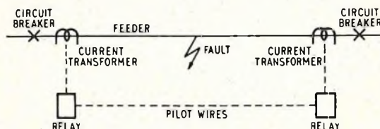
FIG. 3.—PRINCIPLE OF "TRANSLAY" SYSTEM OF PROTECTION AS APPLIED TO A HYPOTHETICAL SINGLE-WIRE FEEDER WITH EARTH RETURN.
