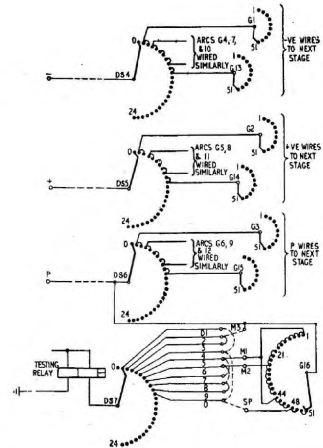
FIG. 4.—SELECTION OF MOTOR UNSELECTOR ARCS AND OUTLET GROUPS BY DIGIT SWITCH.
