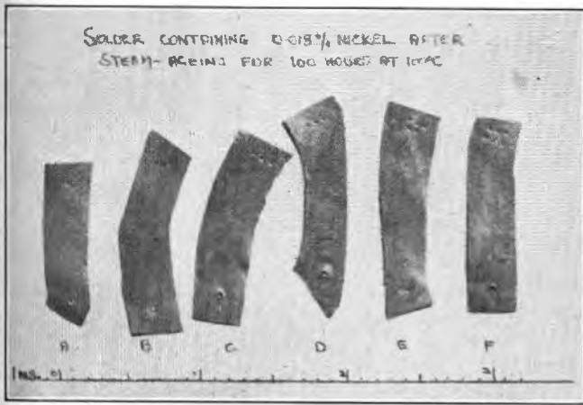
FIG. 9.—TEST PIECES CONTAINING NICKEL AFTER STEAM-AGING.
