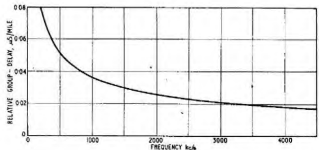
FIG. 2.—BIRMINGHAM-MANCHESTER COAXIAL CABLE; GROUP DELAY RELATIVE TO ASYMPTOTIC VALUE. (5.58 microseconds/mile = 179,500 miles/sec.)
