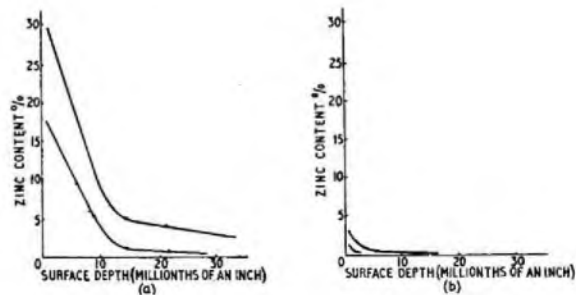
FIG. 6.—COMPARISON OF ZINC CONTENT IN SURFACE SOLDER APPLIED TO TAGS BY (a) MASS SOLDERING ON BRASS TAGS; (b) USING NI-PLATED BRASS TAGS AND A TEMPERATURE-CONTROLLED SOLDER BATH.
