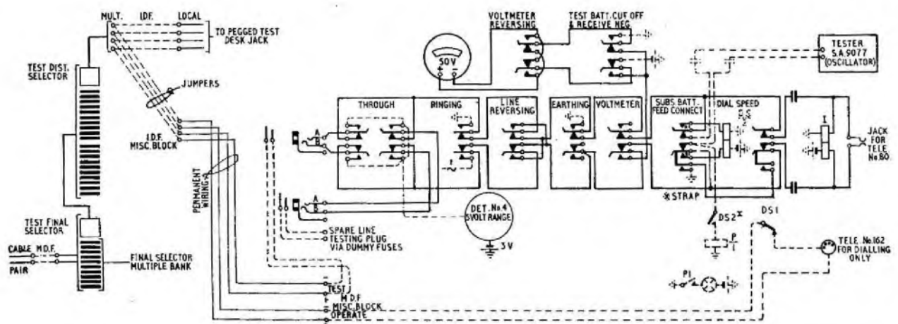
FIG. 2.—TESTER AT 2607 MODIFIED (AS SHOWN BY DOTTED CONNECTIONS) FOR USE AT AUTOMATIC EXCHANGES ONLY.
