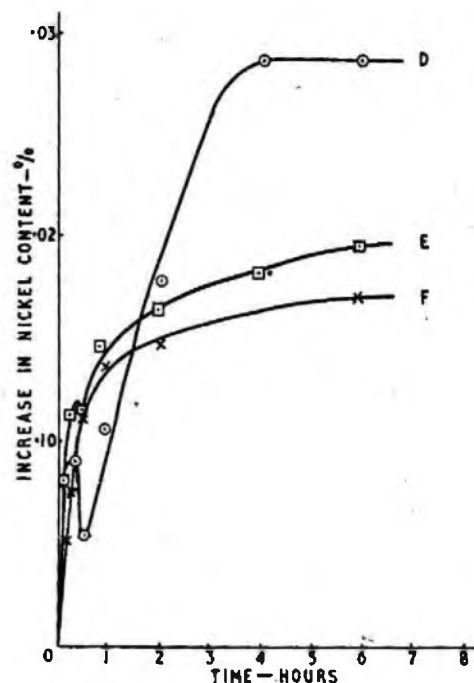
FIG. 3.—NICKEL CONTENT OF 60/40 SOLDER AFTER PROLONGED CONTACT WITH NI-PLATED BRASS WIRE WHEN SOLDER TEMPERATURE WAS: D—350°C; E—250°C; F—210°C.
