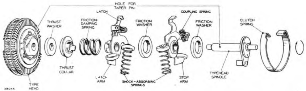
FIG. 6.—EXPLODED SKETCH OF TYPEHEAD.
