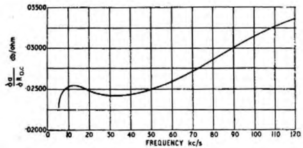
FIG. 4.—DIFFERENTIAL COEFFICIENT OF ATTENUATION WITH RESPECT TO D.C. RESISTANCE v. FREQUENCY.
