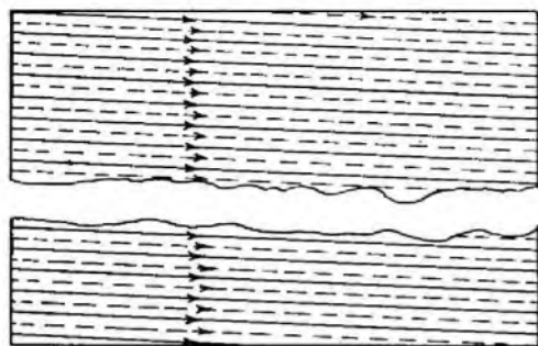
— LINES TRACED OUT DURING ODD FRAMES - - - LINES TRACED OUT DURING EVEN FRAMES FIG. 3.—INTERLACED SCANNING.
