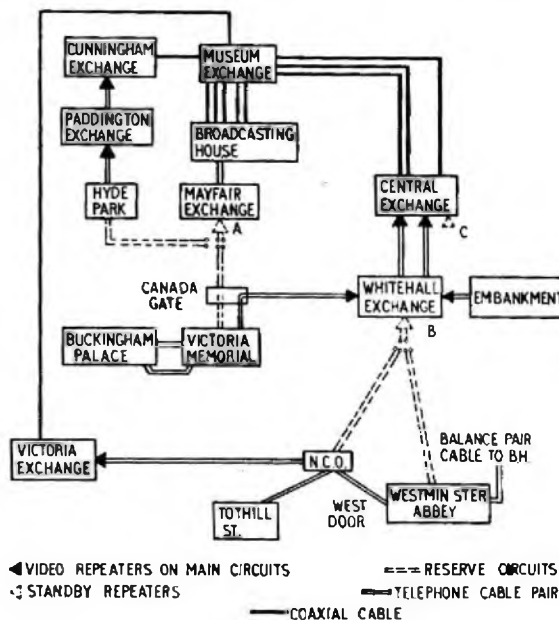
FIG. 11.—TELEVISION CIRCUITS.
