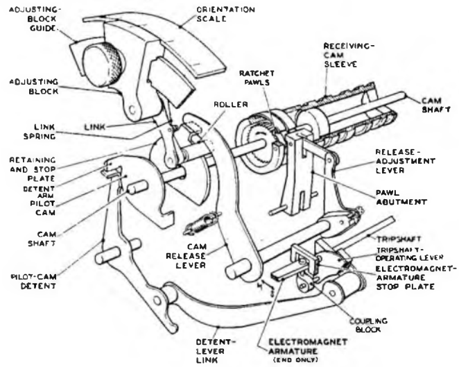
FIG. 4.—ORIENTATION MECHANISM.
