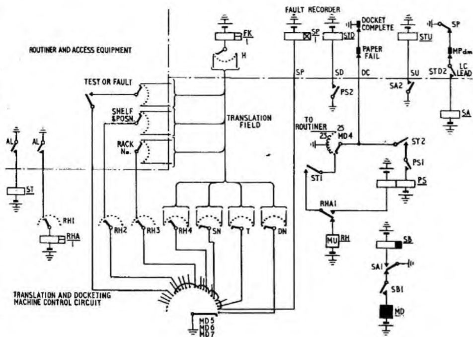
FIG. 8.—CONNECTIONS BETWEEN ROUTINER, CONTROL CIRCUIT AND RECORDER.
