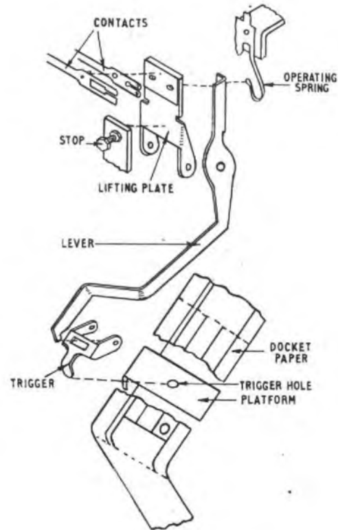
FIG. 6.—DOCKET FAIL ALARM MECHANISM—EXPLODED VIEW.
