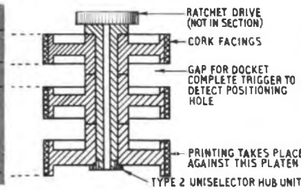
FIG. 2.—COMPLETED DOCKET AND PLATEN IN SECTION.
