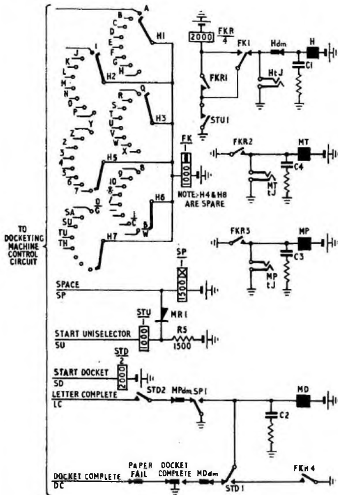
FIG. 7.—CIRCUIT OF RECORDER.
