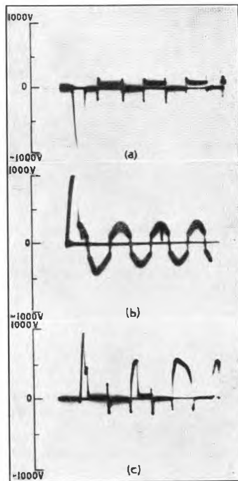
FIG. 3.—TYPICAL WAVEFORMS ACROSS OLD TYPE GAS DISCHARGE TUBES,
