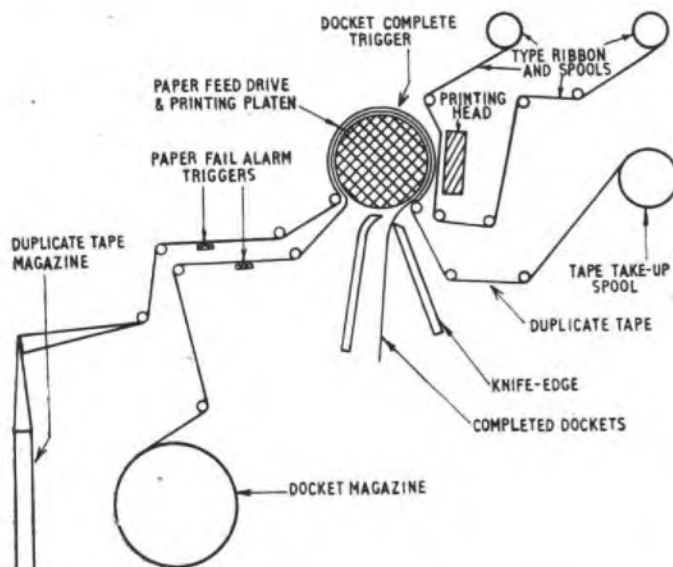
FIG. 3.—PATH OF PAPER THROUGH RECORDER.
