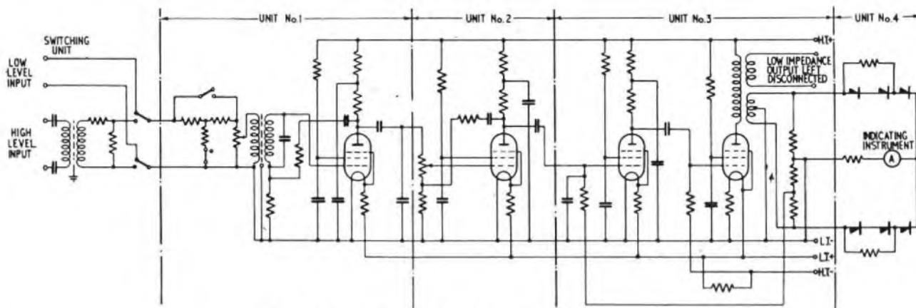
FIG. 4.—CIRCUIT OF A.C. VOLTMETER AND AMPLIFIER.
