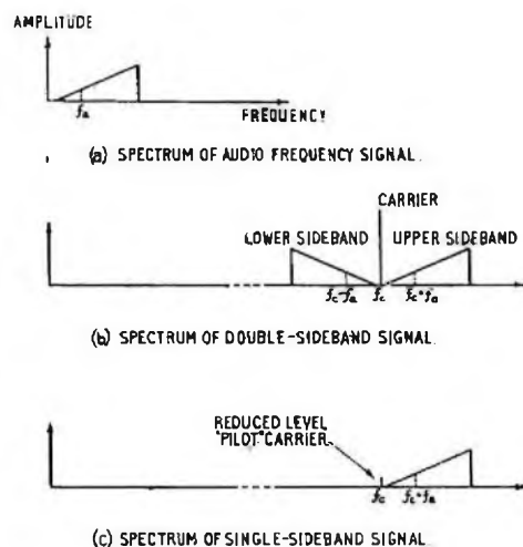
FIG. 1.—SIGNAL SPECTRA.
