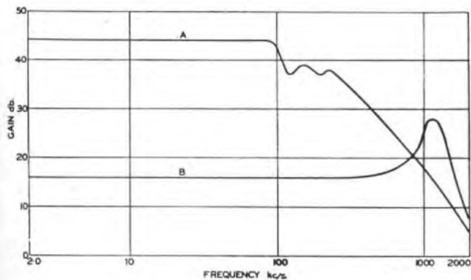
FIG. 7.—GAIN/FREQUENCY CHARACTERISTIC ABOVE 2 kc/s A. WITHOUT NEGATIVE FEEDBACK. B. WITH NEGATIVE FEEDBACK.
