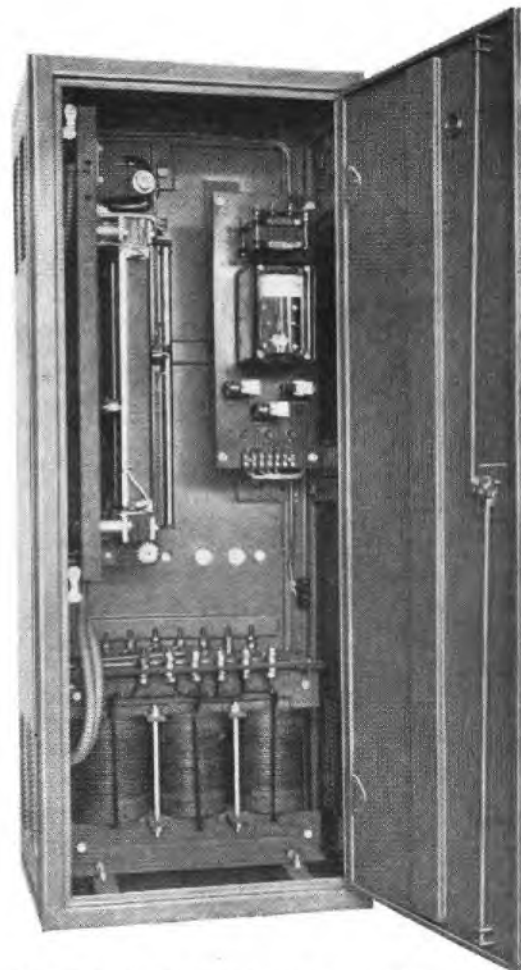
Top: 3-phase, air cooled, floor mounting (cubicle) model. Input 440V ± 10%, output 440V ± 1%, 40 amps.
