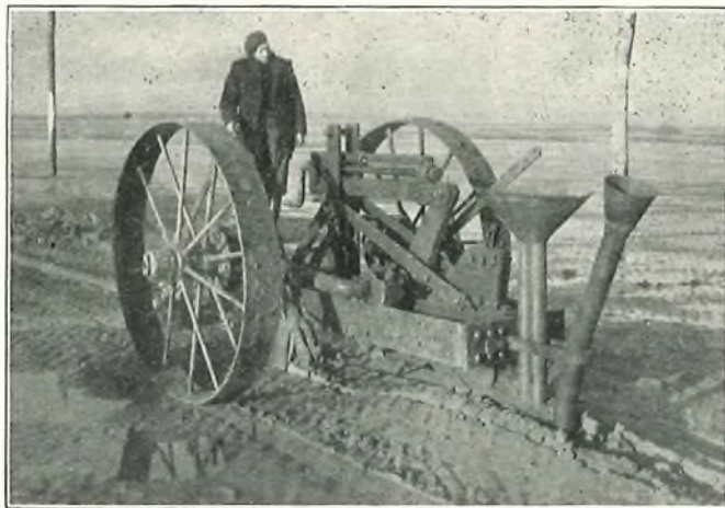
THE MOLE-PLOUGH.
