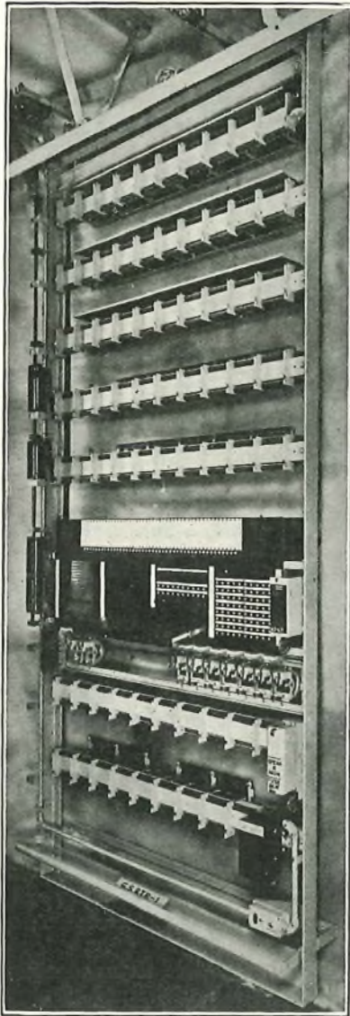
FIG. 1.—FRONT VIEW OF ROUTINER CONTROL RACK.
