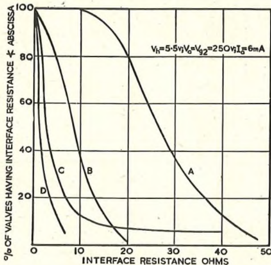
FIG. 4.—DISTRIBUTION OF INTERFACE RESISTANCE OF FOUR BATCHES OF VALVES TYPE CV138 (MADE BY DIFFERENT MANUFACTURERS) AFTER 4,000 HOURS ON LIFE-TEST RACKS.
