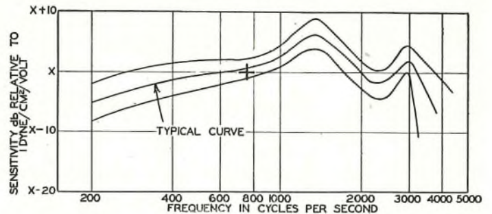
FIG. 6.—PERMISSIBLE LIMITS FOR THE RESPONSE OF MICROPHONES USED WITH INSERT AID.
