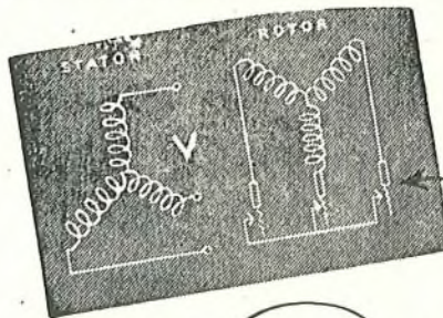
A.C. Polyphase Wound Rotor-Rheostat.
