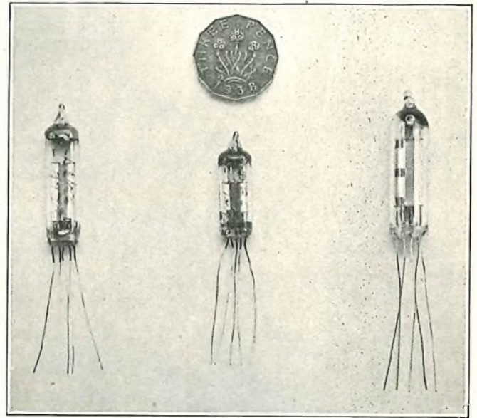
FIG. 7.—LATEST TYPES OF VALVES USED. Left, CV2106; centre, CV2107; right, CV387.
