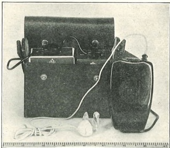
FIG. 2.—A COMPLETE, MK. IIA, INSERT AID.
