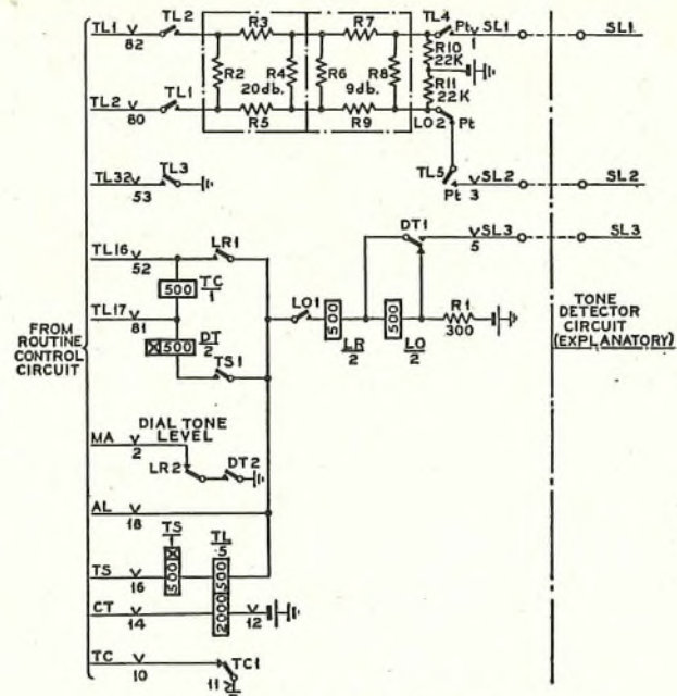
FIG. 5.—CIRCUIT OF A TYPICAL TEST RELAY SET.
