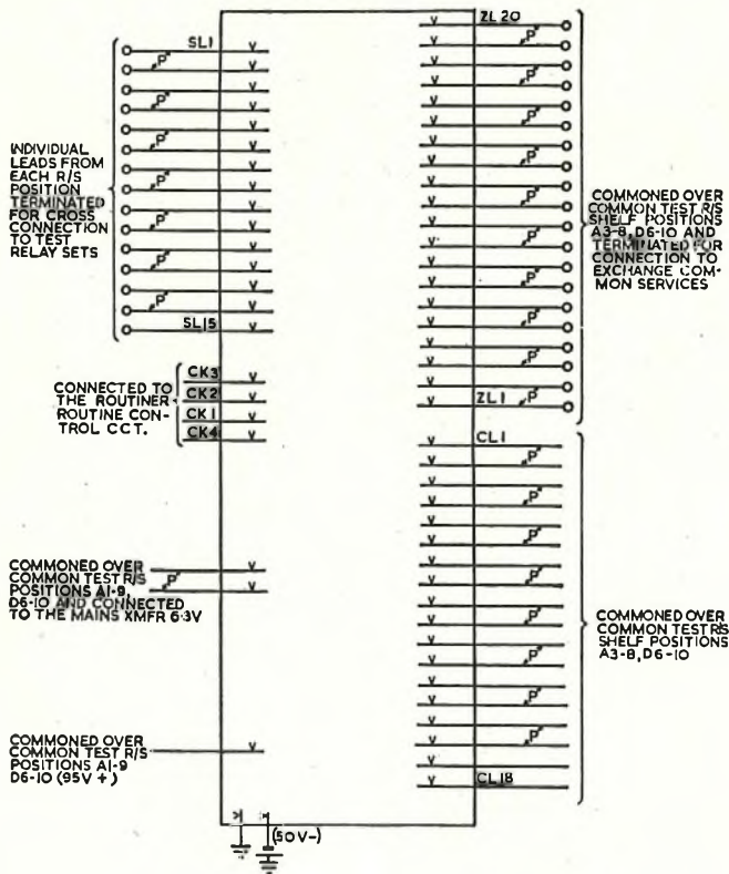
FIG. 6.—WIRING OF A COMMON TEST RELAY SET.
