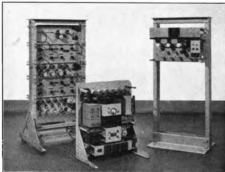
FIG. 5.—TELEPHONE CABLE REPEATER AND POWER PACK (LEFT), COAXIAL CABLE REPEATER (RIGHT).
