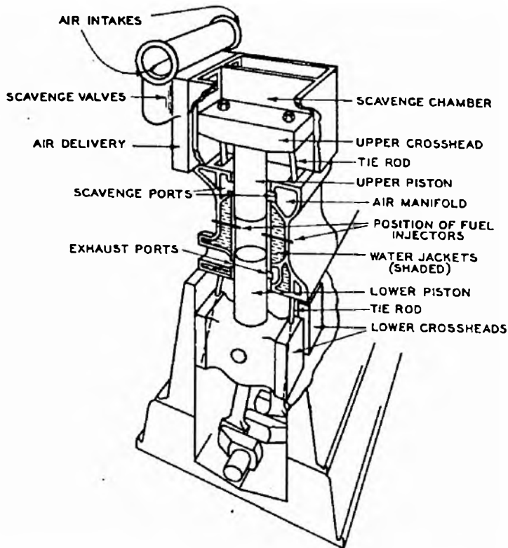
FIG. 2. SECTIONAL VIEW OF TWO CYLINDER UNIT OF FULLAGAR ENGINE.
