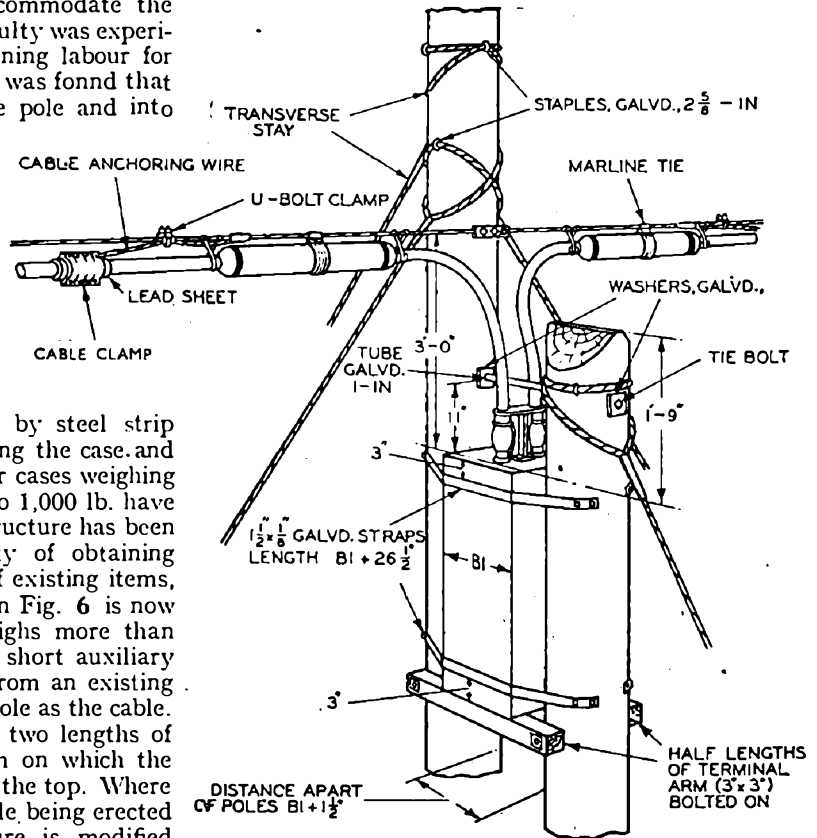
FIG. 6.—MOUNTING OF LOADING COIL CASE.
