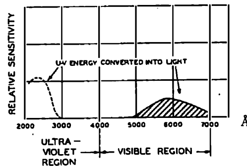
FIG. 2.—GRAPH ILLUSTRATING CONVERSION OF RADIANT ENERGY INTO LIGHT.
