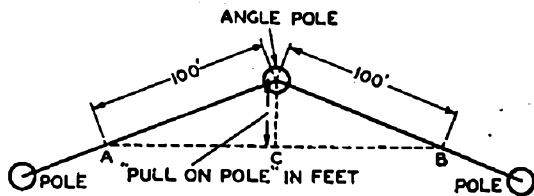
FIG. 2.—"PULL-ON-POLE" MEASUREMENT.
