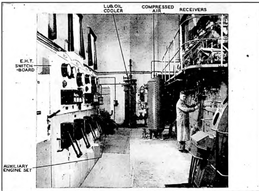
FIG. 3. GENERAL VIEW OF ENGINE AND E.H.T. SWITCHBOARD.
