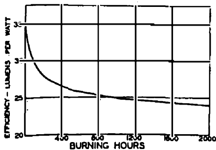
FIG. 5.—TYPICAL EFFICIENCY/LIFE CURVE.
