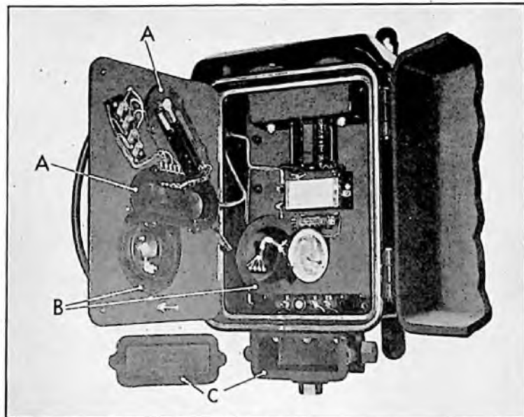
FIG. 3.—TELEPHONE No. 149—INTERNAL LAYOUT.
