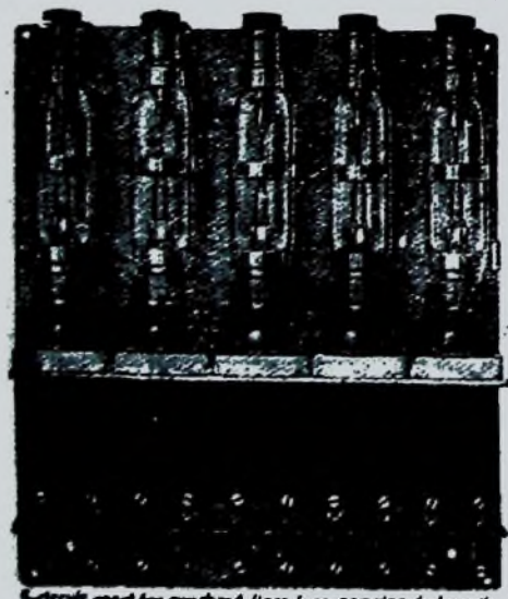
5-drain panel for overhead lines incorporating choke coils, spark gaps, etc.
