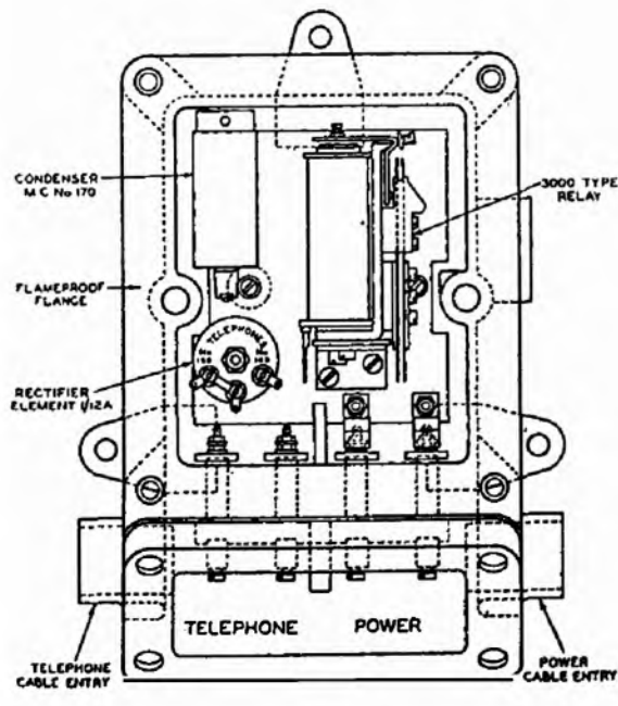
COVERS REMOVED FIG. 6.—RELAY UNIT.
