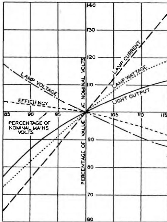
FIG. 7.—GRAPH ILLUSTRATING EFFECT OF SUPPLY VOLTAGE VARIATIONS.
