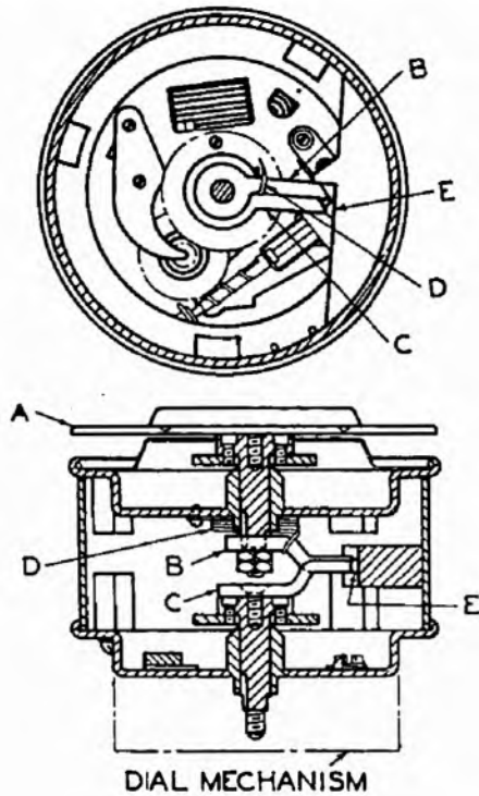
FIG. 5.—DIAL MECHANISM FITTED WITH SLIPPING CLUTCH DEVICE.
