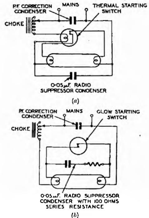
FIG. 4.—TYPICAL LAMP OPERATING CIRCUITS.
