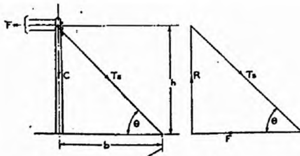
FIG. 1.—FORCES ACTING ON STAYED POLE.
