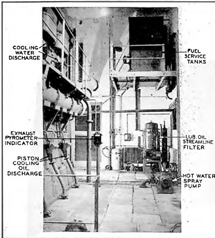
FIG. 4. VIEW OF ENGINE ROOM SHOWING POSITION OF ELEVATED STORAGE TANKS.
