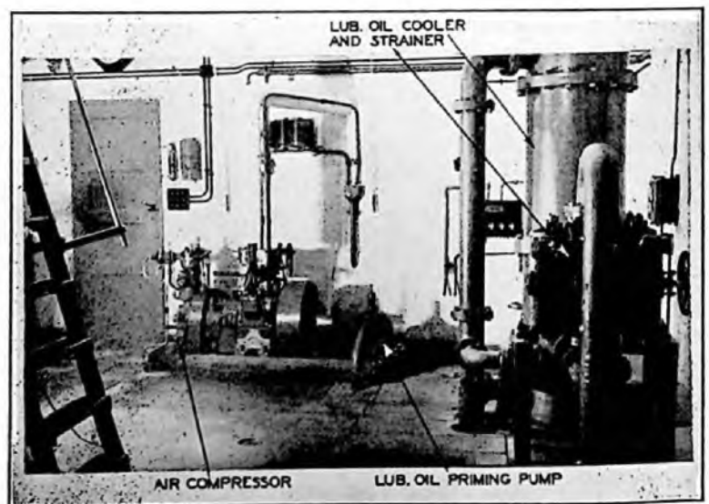
FIG. 5. AUXILIARY EQUIPMENT.
