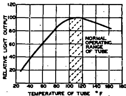
FIG. 6.—GRAPH ILLUSTRATING EFFECT OF TUBE TEMPERATURE ON EFFICIENCY.
