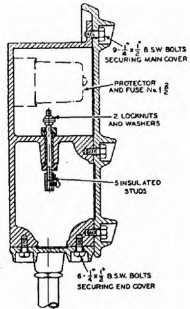
FIG. 7. PROTECTOR AND FUSE UNIT.
