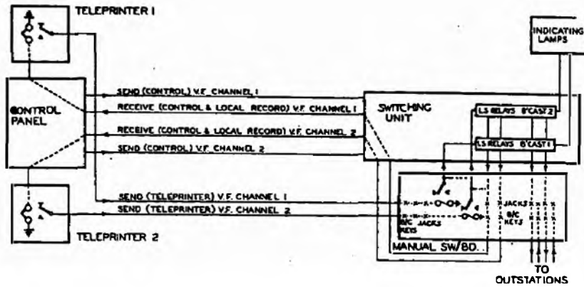
FIG. 3.—SCHEMATIC DIAGRAM OF TELEPRINTER BROADCAST SYSTEM.
