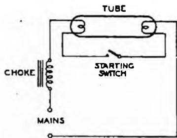
FIG. 3.—ELEMENTARY LAMP OPERATING CIRCUIT.
