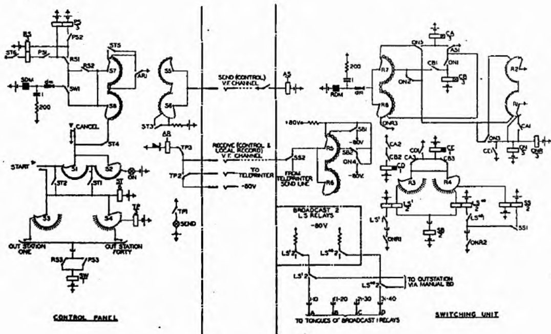
FIG. 4.—CIRCUIT ELEMENTS ASSOCIATED WITH BROADCAST 1.
