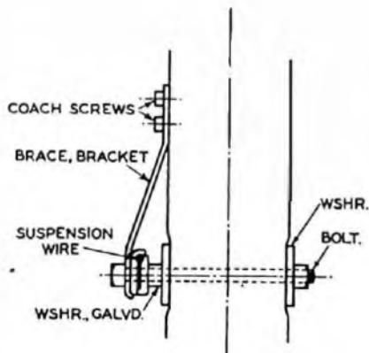
FIG. 4.—METHOD OF ATTACHMENT FOR SUSPENSION WIRE.
