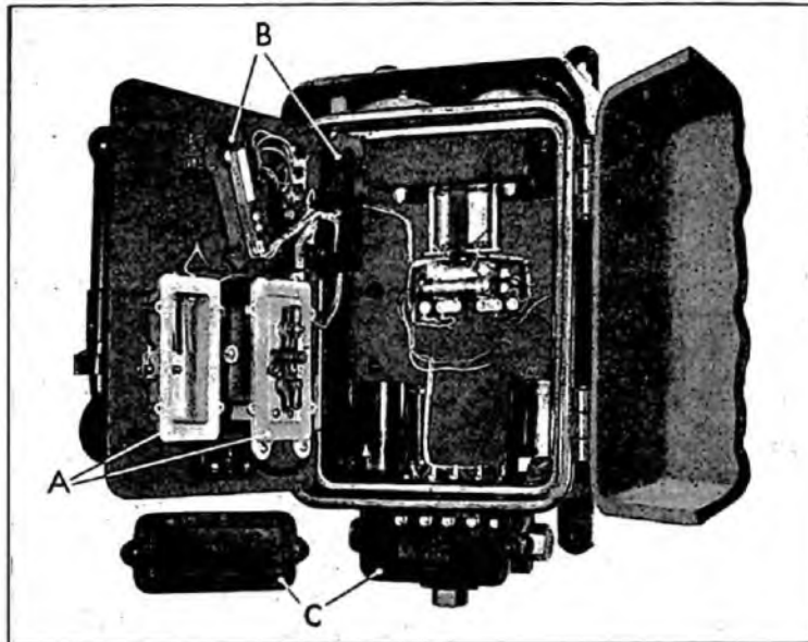
FIG. 4.—TELEPHONE No. 153—INTERNAL LAYOUT.
