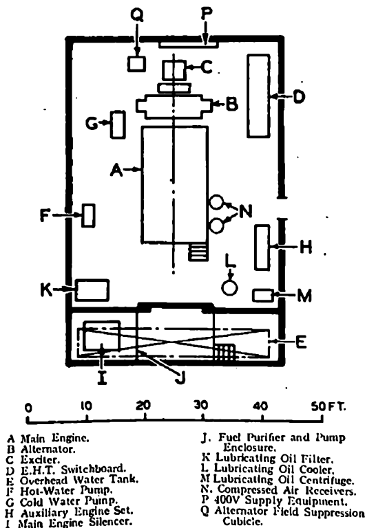
FIG. 1. GENERAL PLAN OF LAYOUT.
