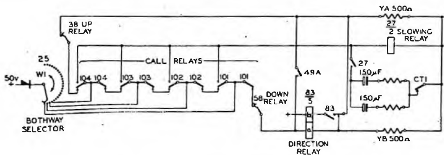
FIG. 4.—DIRECTION AND SLOWING RELAY CIRCUIT.
