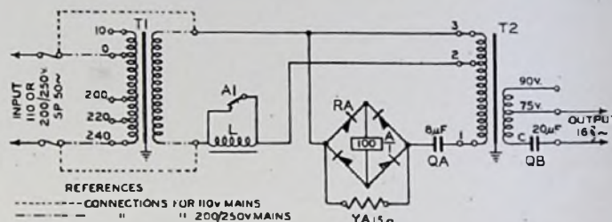
FIG. 7.—SCHEMATIC DIAGRAM OF RINGING CONVERTER NO. 1.
