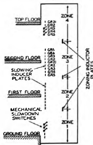
FIG. 2.—TYPICAL LAYOUT OF ZONE AND INDUCER PLATES.
