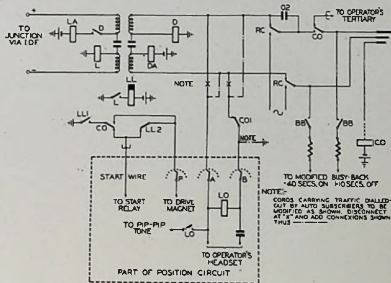
FIG. 4.—SIMPLIFIED SCHEMATIC OF S.F.J. CORD CIRCUIT SHOWING WIRING MODIFICATIONS TO PREVENT PREMATURE METERING.
