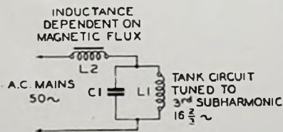
FIG. 1.—ELEMENTS OF BASIC CIRCUIT.
