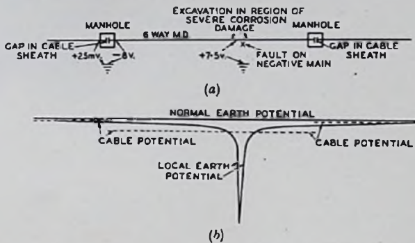
FIG. 2.—TYPICAL LEAKAGE CONDITION FROM D.C. SYSTEM.
