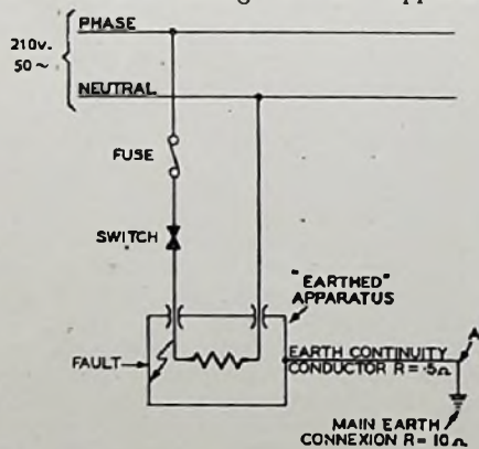
FIG. 1.—TYPICAL A.C. FAULT CONDITION.
