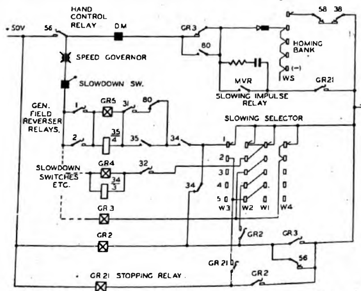
FIG. 6.—SLOWING SELECTOR, GENERATOR FIELD RELAYS, ETC.
