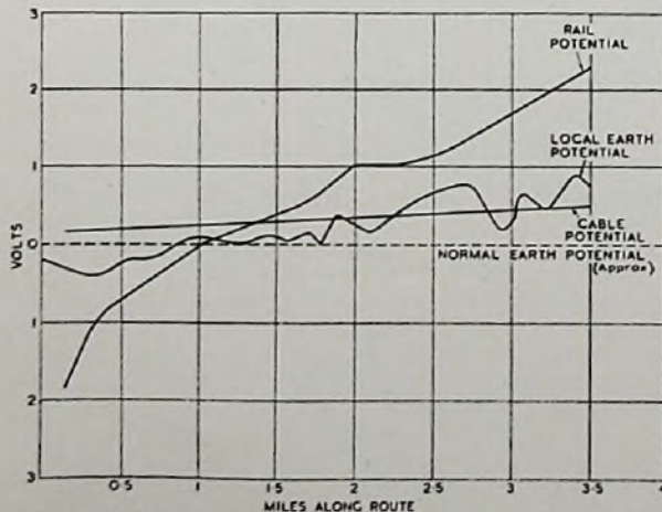
FIG. 6.—TEST RESULTS ON TRAMWAY ROUTE IN LIVERPOOL.
