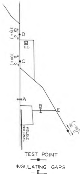
FIG. 13.—RESULT OF FITTING A TEMPORARY GAP AT A.
