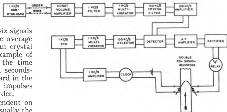
FIG. 7.—APPARATUS FOR THE MEASUREMENT OF 1,000 C/S TONE AT RADIO FREQUENCY.
