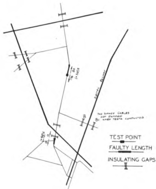
FIG. 8.—RESULTS OF FITTING INSULATING GAPS.
