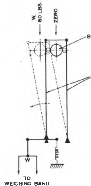
FIG. 8 —WEIGHING MECHANISM.
