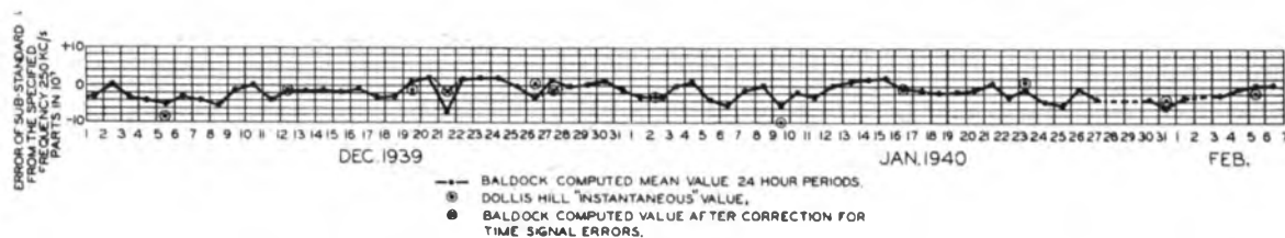
FIG. 13.—COMPARISON OF BALDOCK FREQUENCY SUB-STANDARD, WITH THE DOLLIS HILL STANDARD, DEC. 1ST, 1939, TO FEB. 7TH, 1940.
