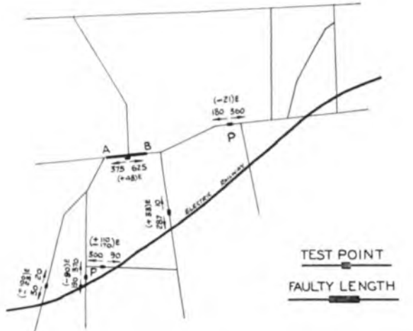
FIG. 5.—RESULTS OF ELECTRICAL TESTS BEFORE FITTING INSULATING GAPS.
