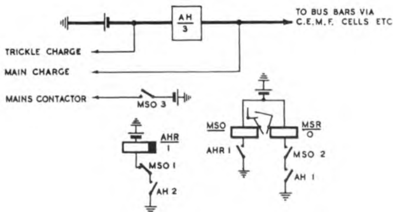
FIG. 2.—TYPICAL CIRCUIT APPLICATION.
