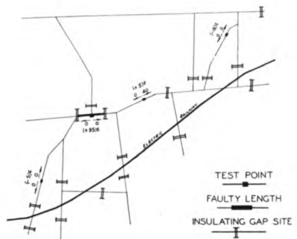
FIG. 6.—TEST RESULTS AFTER FITTING INSULATING GAPS.
