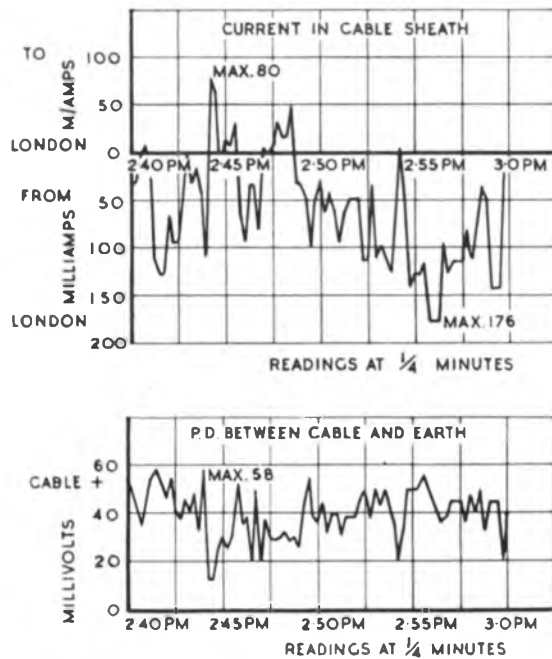
FIG. 10.—ELECTRICAL TESTS AT SOUTH END OF FAULTY LENGTH AFTER FITTING GAPS.
