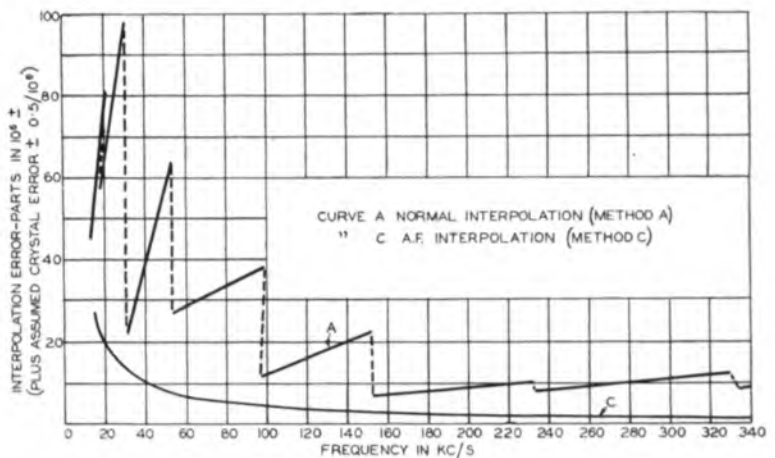
FIG. 5.—I.W. AND A.F. OSCILLATORS—INTERPOLATION ERROR (PLUS ASSUMED CRYSTAL ERROR OF \pm 0.5/10^6 ).
