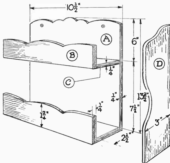
Fig. 2—Details of parts and construction
