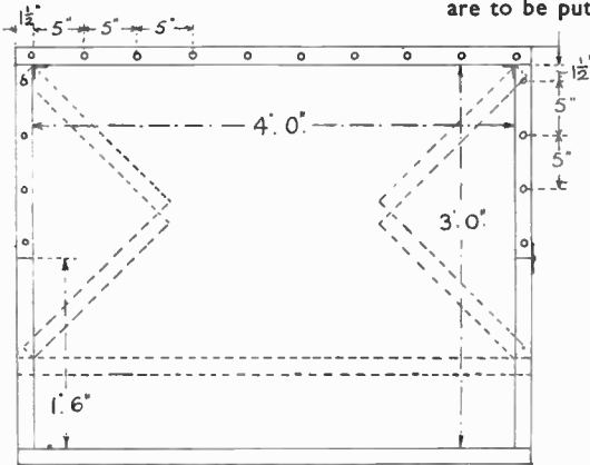
Fig. 1—Plan of frame with folds shown by dotted lines
