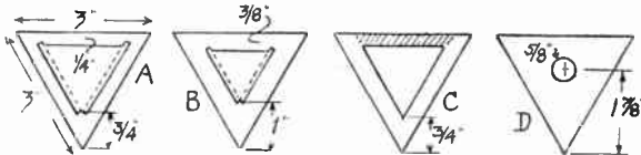
Fig. 1—The triangles to be cut as detailed
