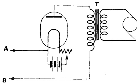
KENOTRON IN CIRCUIT
