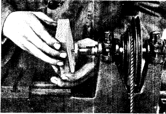
Fig. 4. In this photograph the operator is seen mounting a wood block on the screw chuck
