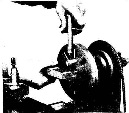
Fig. 10. An angle plate and a dog may be used for fixing the work on a face plate
