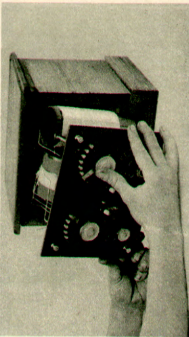
Fig. 20. How the components when mounted upon the panel are fitted into the case
