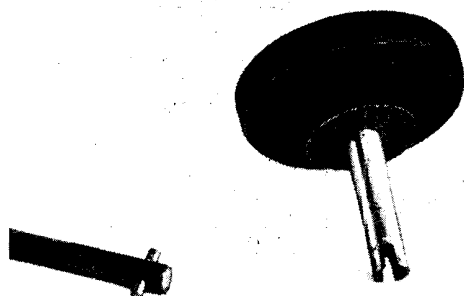
Fig. 11. On the spindle is a cross pin which fits into the slot of the shank of the knob
