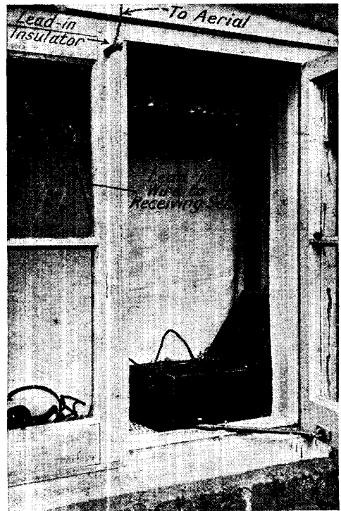
LEAD-IN CONNEXION
