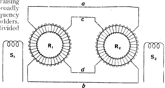
CONNEXIONS OF KORDA FREQUENCY ADDER
