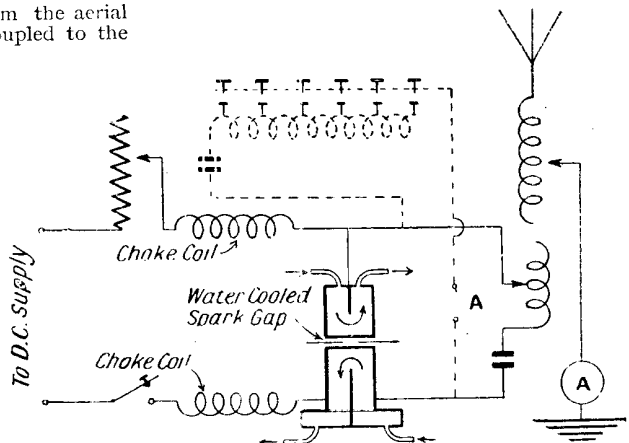
TRANSMITTER EMPLOYING LEVEL SYSTEM
