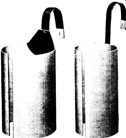
Fig. 7. Two types of the cylindrical zinc electrodes used in the Leclanché cell in Fig. 6 are illustrated. A third type is shown in Fig. 4
