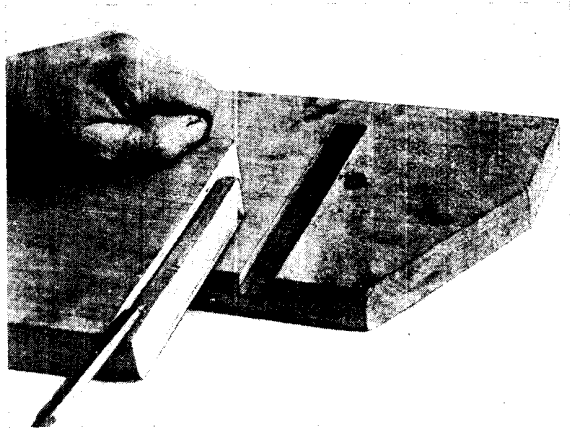
Fig. 4. This is a dovetail, stopped housing joint, and is an improved form of the joints in Figs. 2 and 3, being much more rigid
