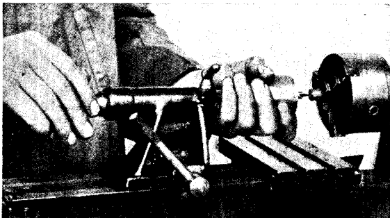
Fig. 16. A Slocomb centre drill is used to form a hollow centre for mounting work in a lathe
