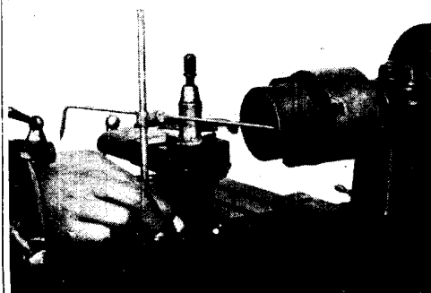
Fig. 20. A surface gauge is being used while dividing work held in the lathe chuck
