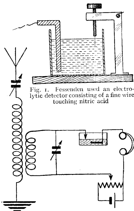
Fig. 2. In this circuit the detector is a liquid barretter, with which is employed a battery with a potentiometer
