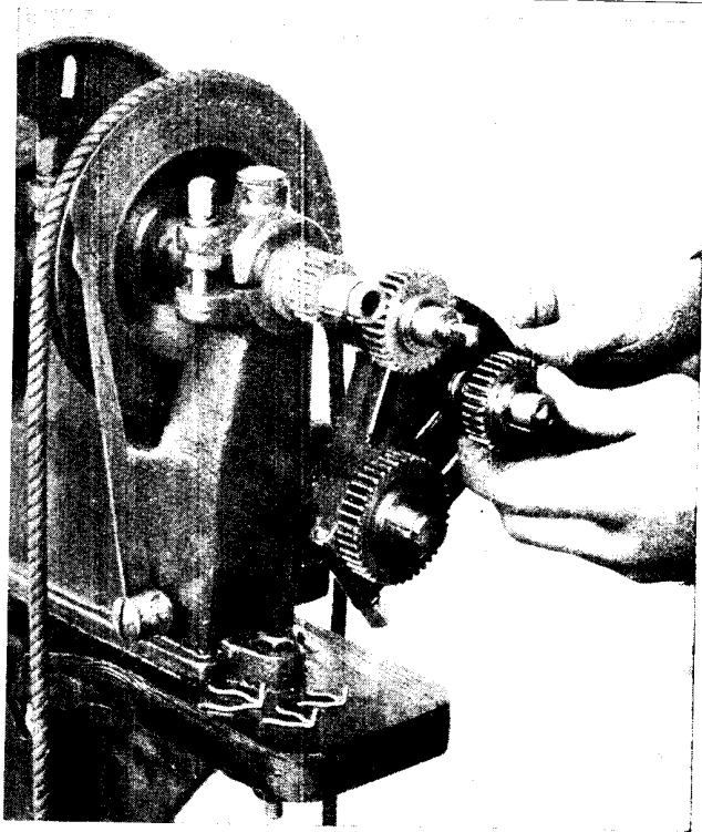
Fig. 25. In order to give the correct ratio between the mandrel and the lead screw the operator is setting up the change wheels
