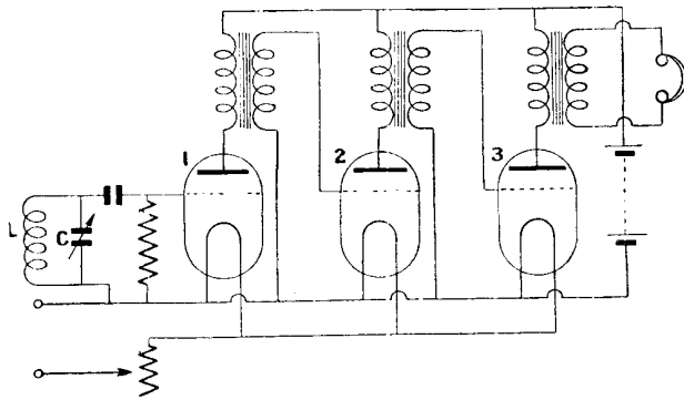
TRANSFORMER-COUPLED NOTE MAGNIFIER
