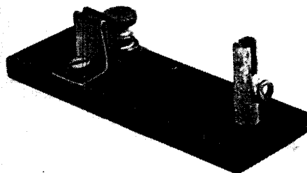
Fig. 5. Spring clips are shown in position on the base. These must be in line with the slot in the blade support
