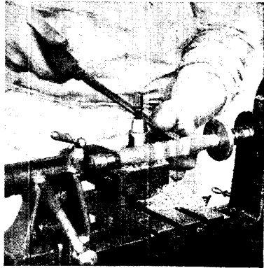
Fig. 5. Here a wooden bar is being turned with the gouge
