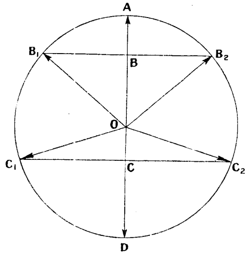
HARMONIC VECTOR RESOLUTION
