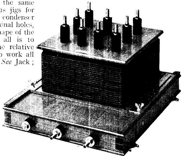
HALF-KILOWATT JIGGER
