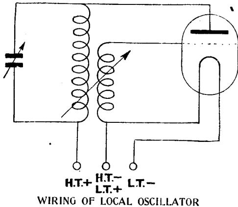
Fig. 6. In this diagram is shown the method of wiring the local oscillator. The valve should be of the hard variety, or a V24 may be used
