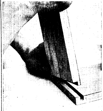
Fig. 3. Square grooved and fingered joints should be used at the end of a piece of board
