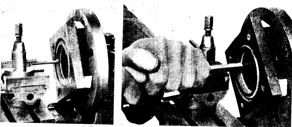
Fig. 26 (left). Mounted in the slide rest is a tool with a V-shaped cutting point bent at the end. This engages the work at an angle, thus enabling a screw thread to be cut internally. Fig. 27 (right). To finish the internal screw thread a hand chaser is used, which reduces the part cut to the exact size required
