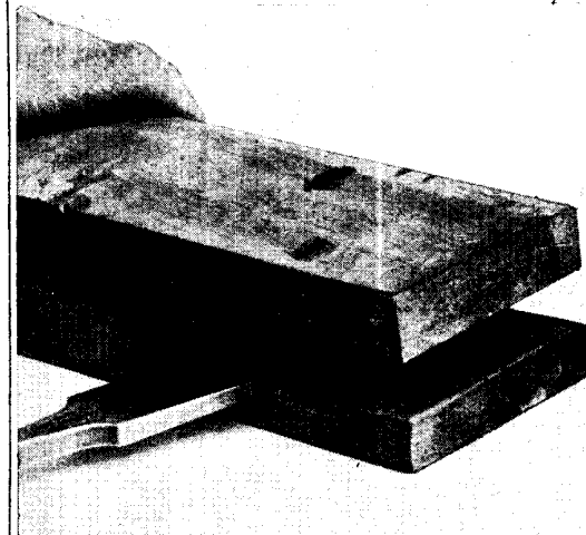
Fig. 5. Simple dovetail joints of this kind are self-locking in one direction. In order to obtain a secure joint the faces of the cut-away portions must be accurately finished and true to measurement
