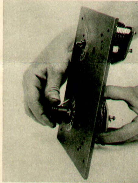
Fig. 14. Both condenser pointers are set at zero before tightening up
