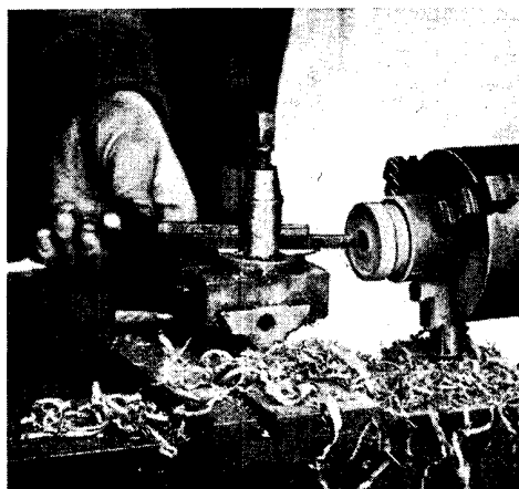
Fig. 12. Ebonite rod is used as material which is turned in a lathe to make a knob. The unturned part can be seen held in the jaws of the chuck
