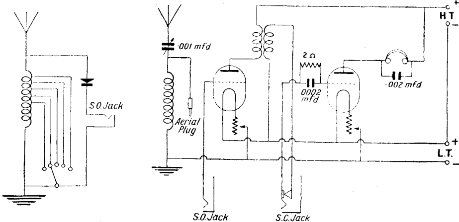
Fig. 3 (left). An S.O. jack is here shown used in a crystal receiving set. Fig 4 (right). Two jacks are employed in this circuit, an S.O. and an S.C., for plugging in the aerial either on to the grid of the high-frequency valve or the grid of the rectifier
