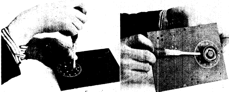
Fig. 4 (left). Illustrated in this photograph is the method of fixing the condenser dial to the panel by small countersunk screws and bolts. Fig. 5 (right). Unless care is taken the condenser pointer may be found out of adjustment with the condenser setting. This illustration shows the method of locking the pointer in position
