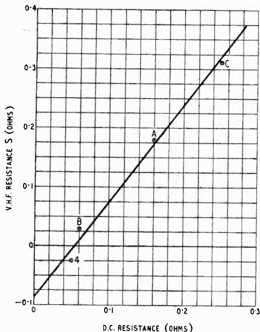
Fig. 4. Relation between v.h.f. and d.c. resistance of sprayed specimens.
