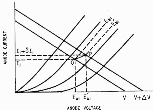
Fig. 6. The change in valve conditions due to an h.t. voltage change is shown.
