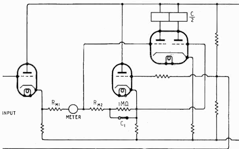
Fig. 4. The use of a relay as an overload protection is shown here.
