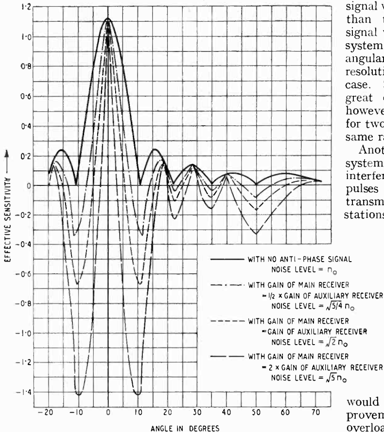
Fig. 7. Effective receiver azimuthal sensitivity diagram.
