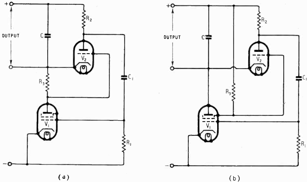
Fig. 2. Basic circuit configurations employing the principle of using the constant-current charging valve to assist the action of the discharge circuit; (a) anode-coupled case; (b) screen-coupled case.
