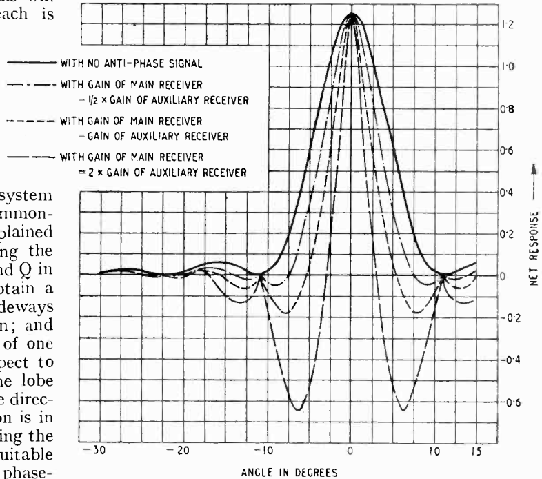
Fig. 8. Overall azimuthal diagram (transmitter radiation \times receiver sensitivity).
