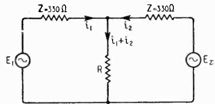
Fig. 4. Equivalent circuit, E_1 , E_2 , i_1 and i_2 are all complex quantities on the usual convention (i.e., multiply by e^{j\omega t} and take the real part).
