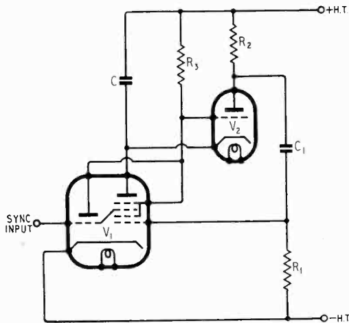
Fig. 6. A triode-hexode charging circuit incorporating sync amplification.
