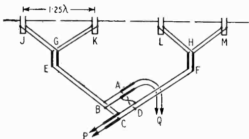
Fig. 2. Feeder bridge used with 4-bay array.
