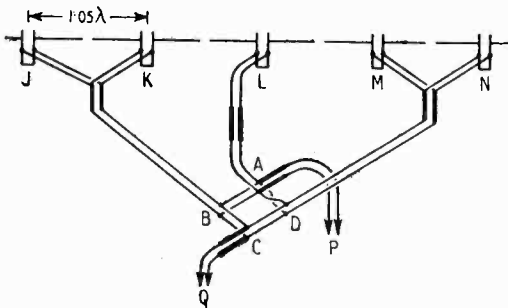
Fig. 5. Feeder bridge used with 5-bay array.
