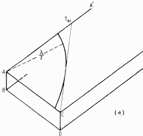
Fig. 9. (a) H_{01} -mode transmitting case; construction for AT_{01} = \lambda_t/2 ; (b) H_{01} -mode attenuating case: construction for AT = \lambda_a/2 .
