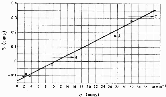
Fig. 2 (above). Comparison of sprayed specimens with thin sheet standards without screening.
