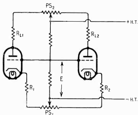
Fig. 2. Insensitivity to h.t. voltage changes is achieved by the adjustment of PS_1 and PS_2 .
