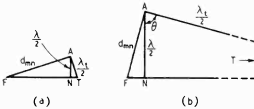
Fig. 3. In both triangles d_{mn} is the same, but in (a) \lambda/d_{mn} is small and in (b) it is large.
