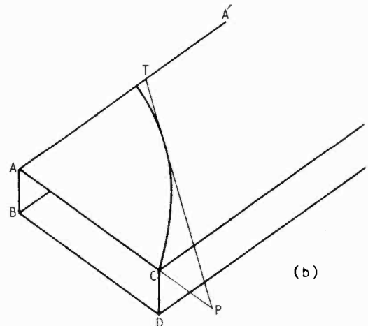
Fig. 9. (a) H_{01} -mode transmitting case; construction for AT_{01} = \lambda_t/2 ; (b) H_{01} -mode attenuating case: construction for AT = \lambda_a/2 .
