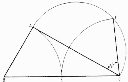
Fig. 13. Construction to determine the angle \psi .
