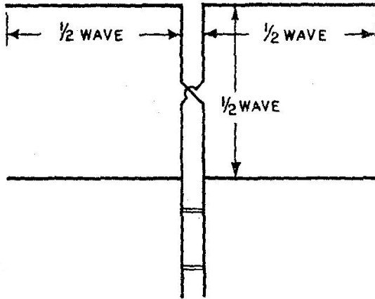
FIG.34 THE LAZY H ARRAY
