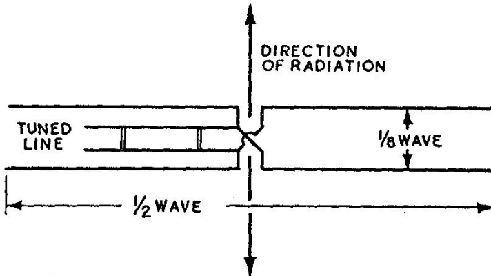
FIG.33 END-FIRE AERIAL
