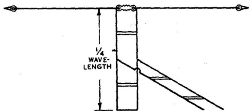
FIG.14 QUARTER-WAVE TRANSFORMER FOR FEEDING INTO A VOLTAGE LOOP. AERIAL AN EVEN NUMBER OF HALF WAVES LONG
