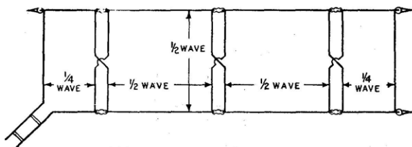
FIG.35 THE STERBA ARRAY
