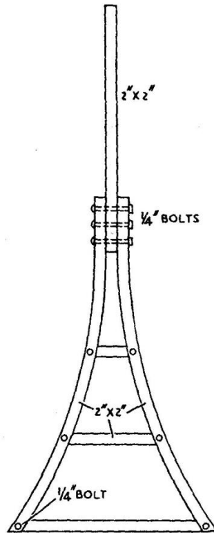
FIG.37 THE 'A' SHAPED MAST
