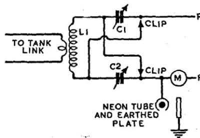
FIG.26 AERIAL TUNING LIMIT
