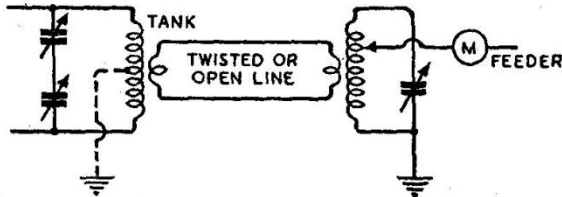
FIG.19 SINGLE WIRE FEEDER COUPLING TO TRANSMITTER DOTTED EARTH LINE INDICATES POINT OF LOW R.F. VOLTAGE
