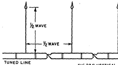
FIG.32 B VERTICAL BROADSIDE AERIAL
