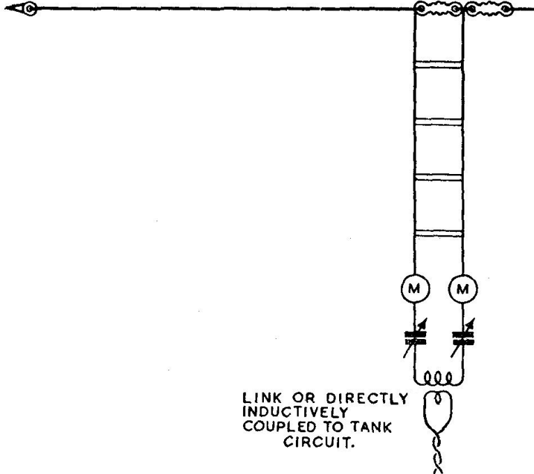
FIG 28 THE ZEPPELIN AERIAL
