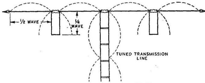
FIG.31 FOUR ELEMENT CO-LINEAR AERIAL VOLTAGE FED
