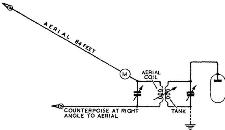
FIG. 29 THE W3EDP MULTI-BAND AERIAL
