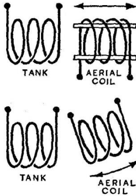
FIG.20 VARIABLE COIL COUPLINGS
