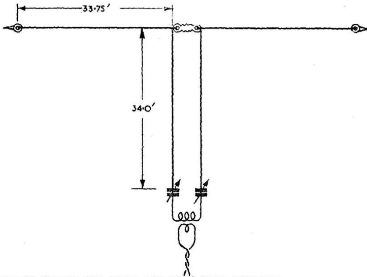
FIG.30 CENTRE-FED AERIAL FOR FOUR BAND WORKING
