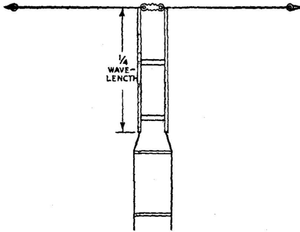
FIG. 13 Q BAR MATCH FOR AERIALS AN ODD NUMBER OF HALF WAVES IN LENGTH
