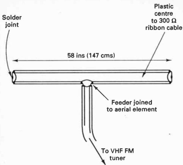
Fig. 3.9 A cheap and easy VHF FM folded dipole.
