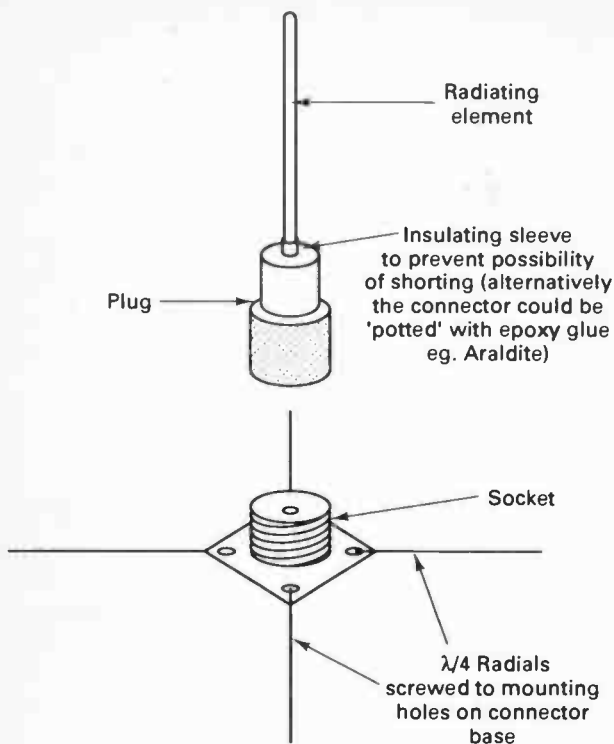
Fig. 6.8 The use of a connector as an aerial base.
