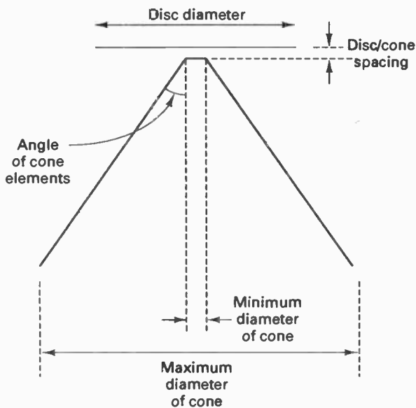
Fig. 7.2 Critical dimensions for a discone.
