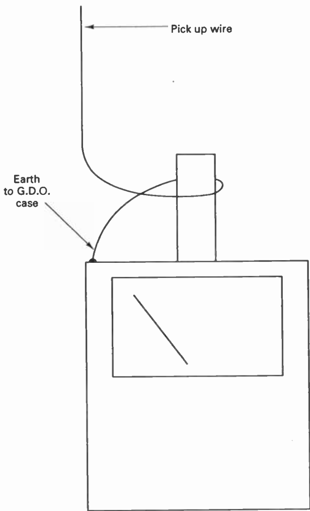
Fig. 8.5 Using a G.D.O. as a field strength meter.
