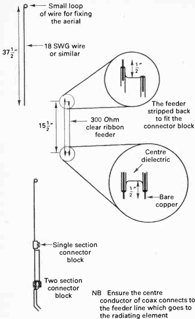
Fig. 6.9 The 2 metre J aerial.
