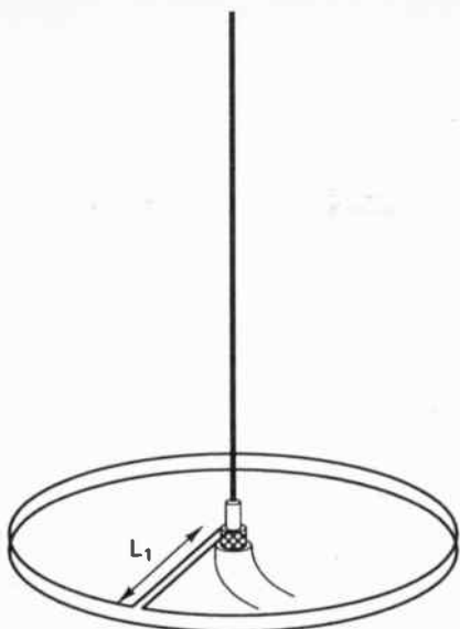
Fig. 6.3 A vertical with an alternative radial system.
