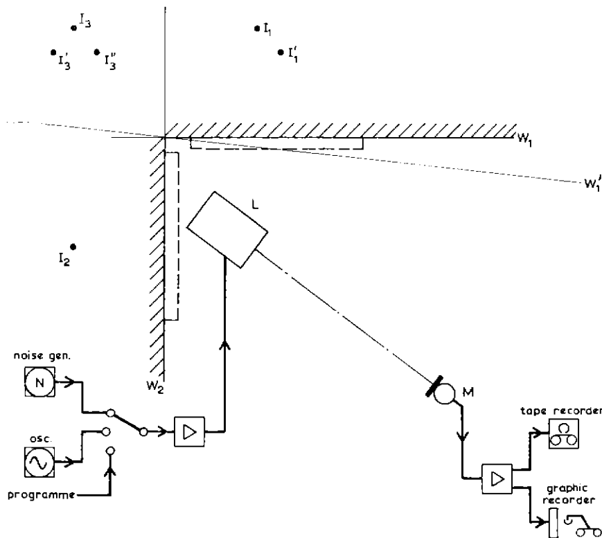
Fig. 10 — Experimental arrangement
