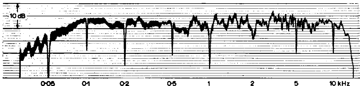
Fig. 12 — Response/frequency characteristic. Loudspeaker in Quality Listening Room (warble tone)
