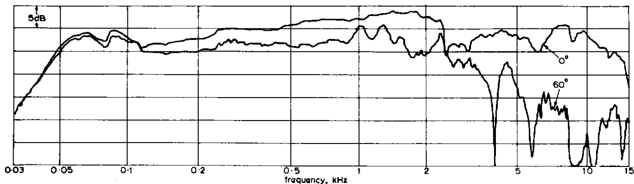
Fig. 1 — Response/frequency characteristics of unequalized low-frequency unit (with slit) in cabinet. Curves at 0^\circ and +60^\circ in vertical plane
