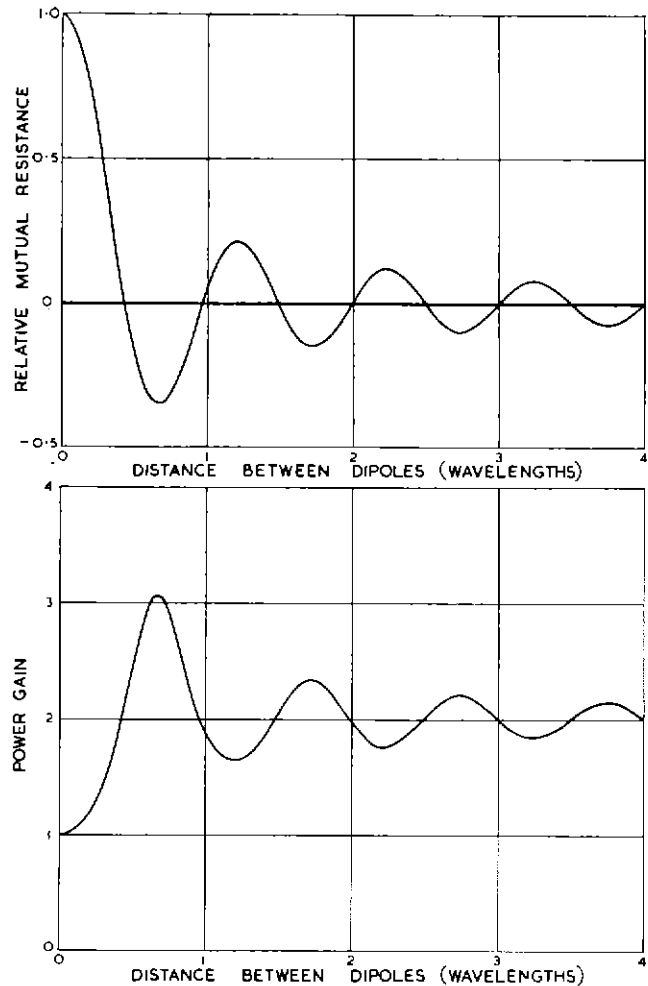
Fig. 2 — The relative mutual resistance and gain of two parallel \lambda/2 dipoles
