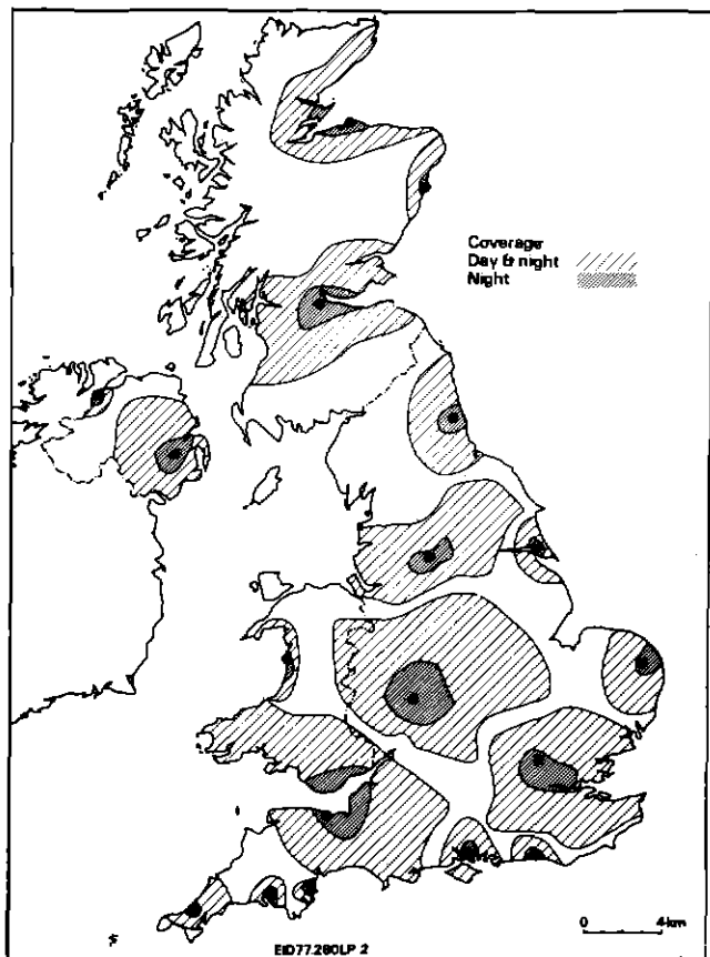
Fig. 5 Radio 1 coverage on 1214kHz
