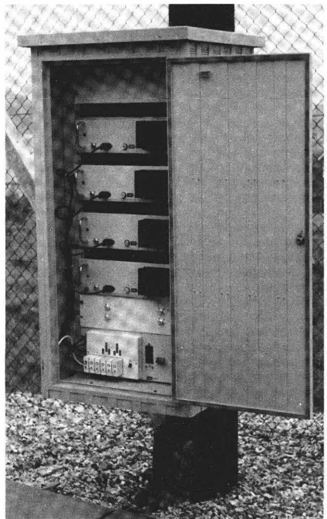
Fig. 4 Four-channel transposer system installed at Tidworth on the Hampshire/Wiltshire border.
