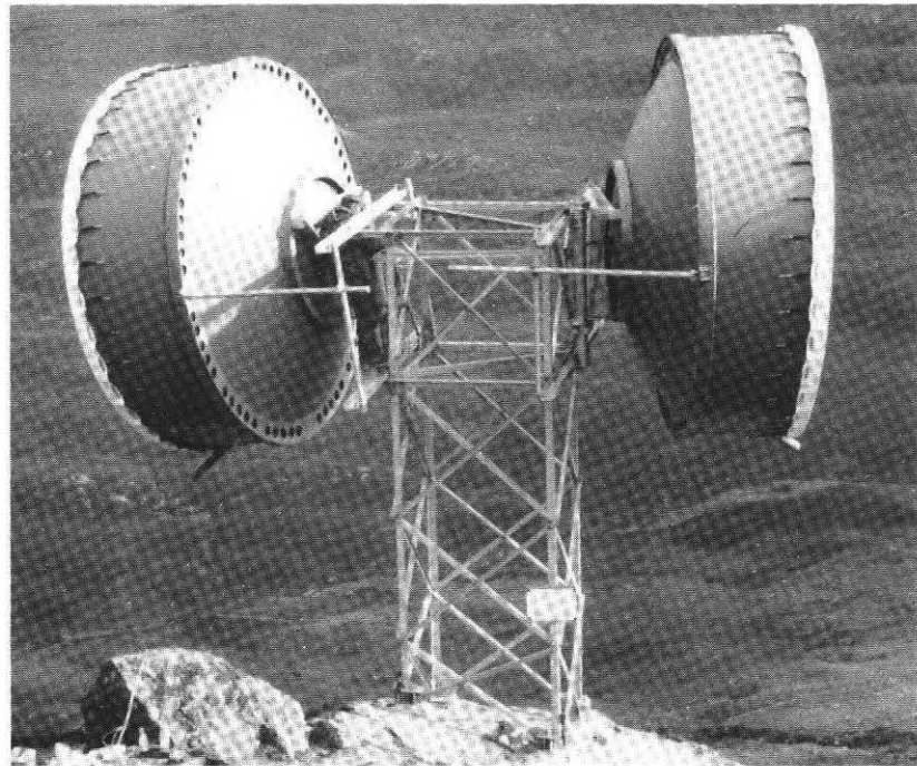
Fig. 5 The passive repeater at Sgurr Marcasaidh uses back-to-back paraboloid aeriels
