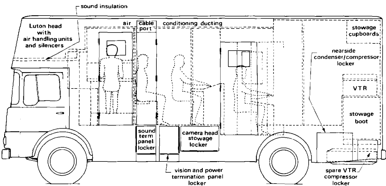
Fig. 1 Layout of the Location Production Unit.
