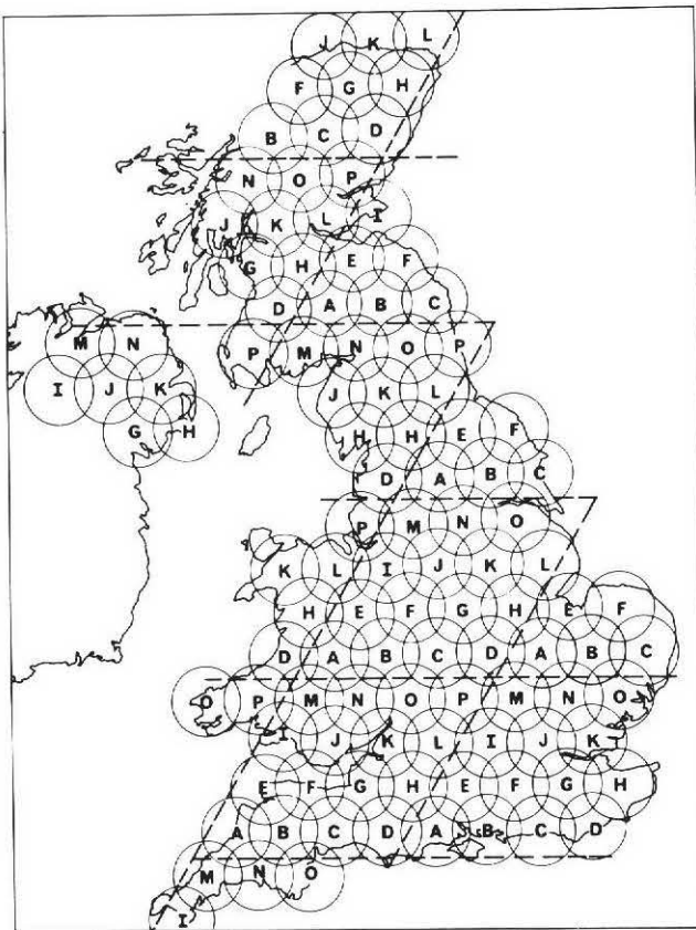
Fig. 7 Traffic information service: transmitter lattice
