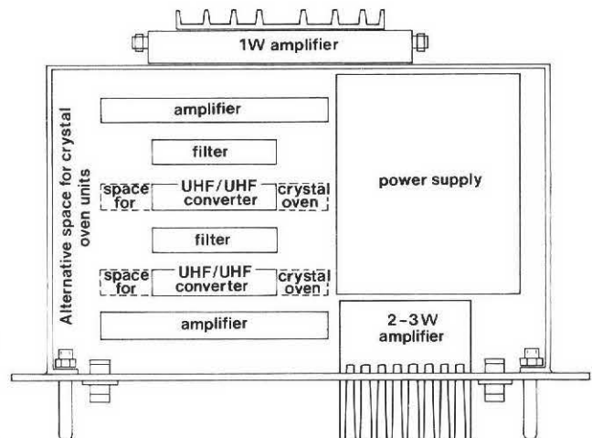
Fig. 3 Second prototype: arrangement of single transposer chassis.
