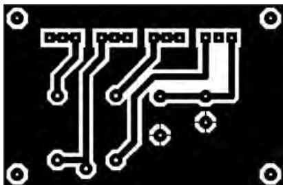
1A - CI platine commande-commutations.
