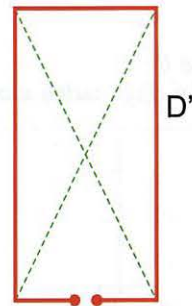
Configuration "x" haute Type Bird Cage (G4ZU)
