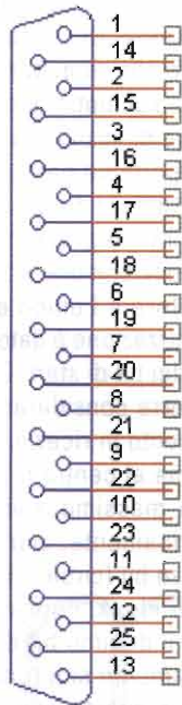
CONNECTOR DB25
