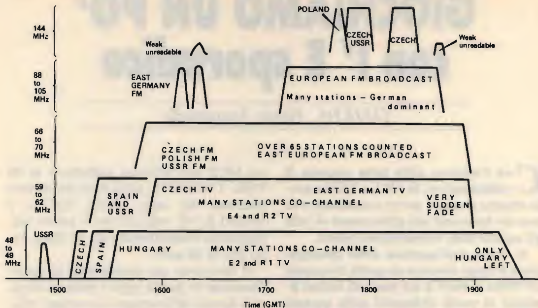
figura 1 Frequency v time for a major sporadic-E event recorded on 10 June 1980 at GM41HJ, Saline, Fife
