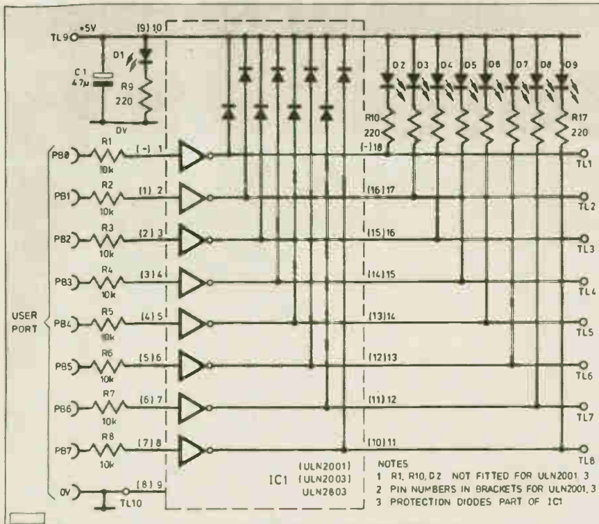
Fig. 2. The complete circuit diagram for the buffer/interface.
