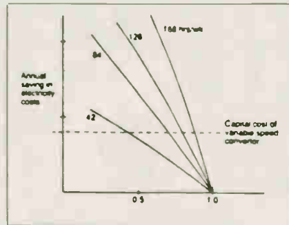
Fig. 1. Annual savings on electrical costs when variable speed drives are used.
