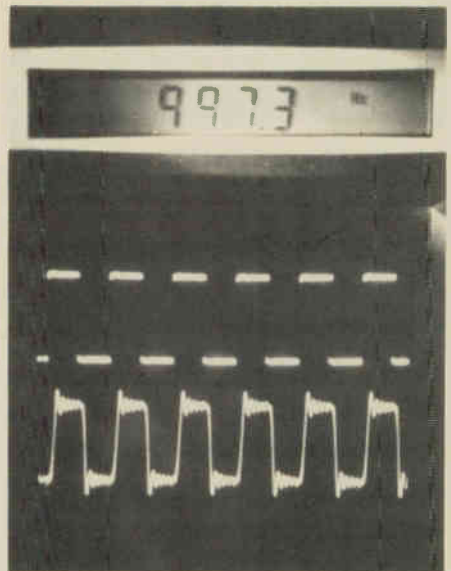
Fig. 6. A 12-bit filtered 1kHz square wave. The upper harmonics that make the square wave square are missing. The upper and lower tones would sound different due to the missing harmonics.
