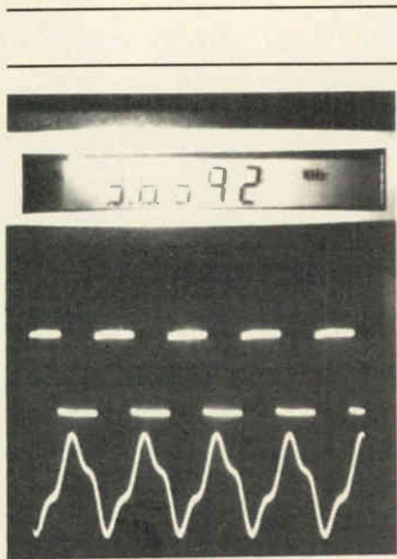
Fig. 7. A 12-bit filtered 3.8kHz squarewave. The squarewave is now reduced to a fundamental with one harmonic.
