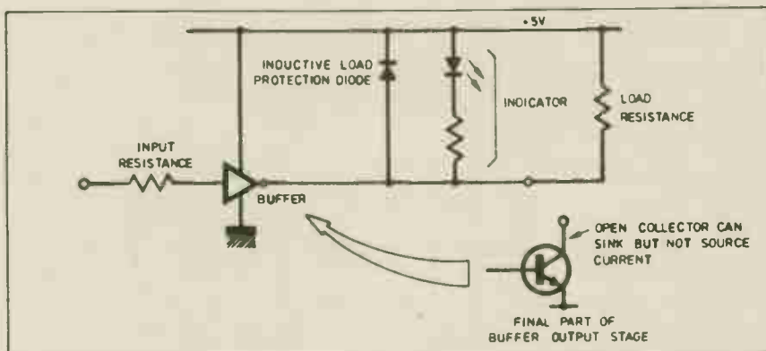
Fig. 1. Single channel arrangement for the buffer/interface.
