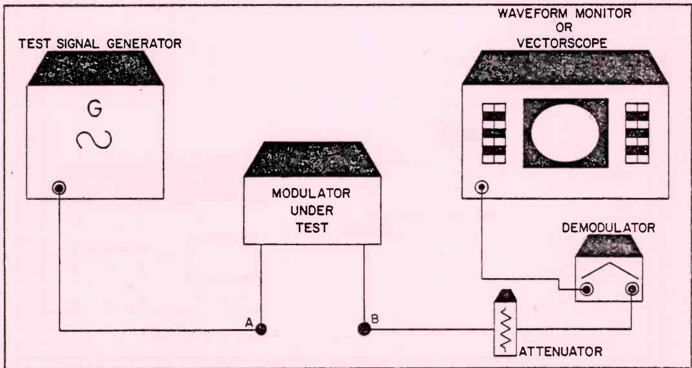
FIGURE 5.11 Arrangement of Test Equipment for the Measurement of Differential Gain and Phase.
