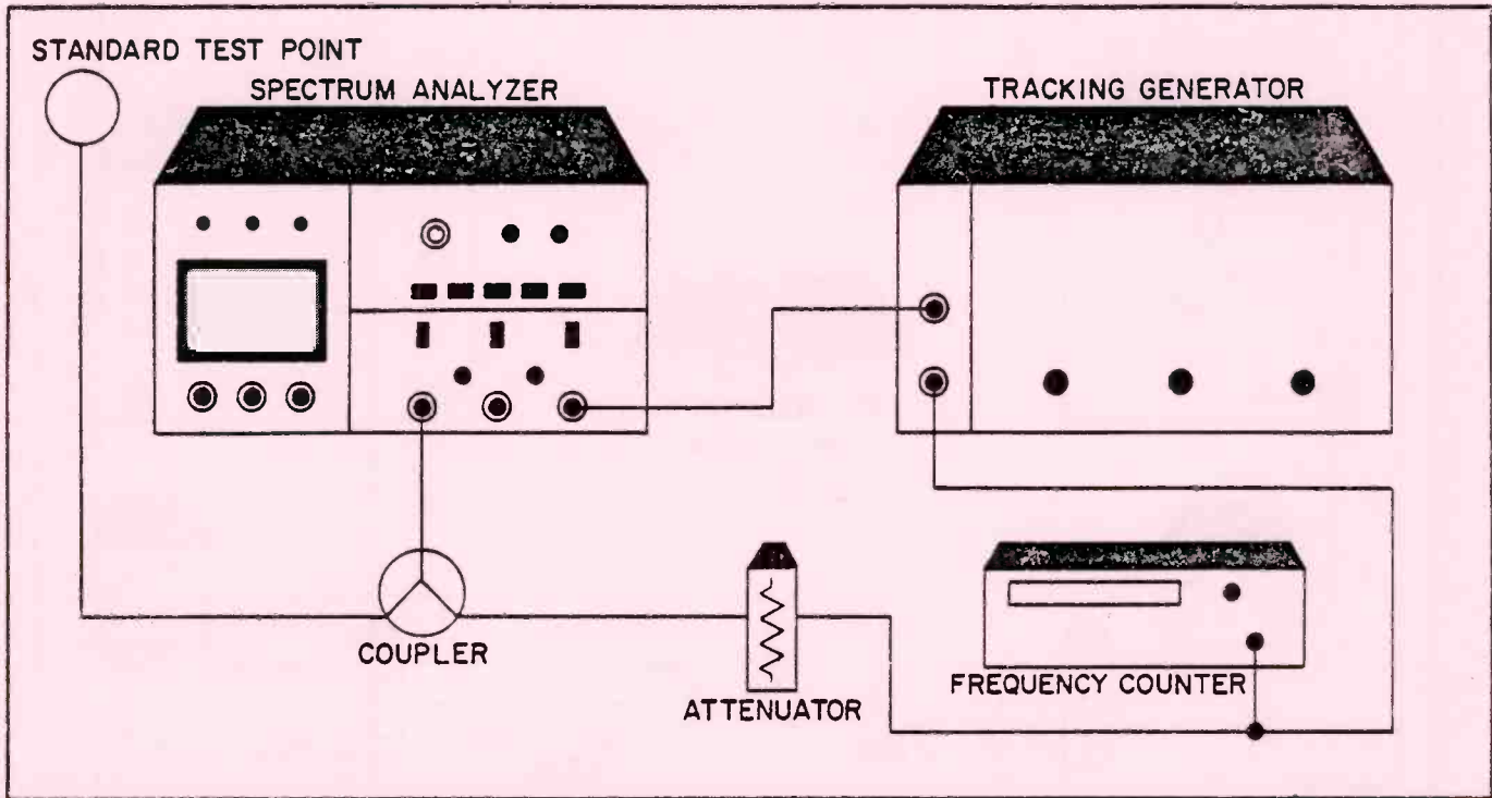
FIGURE 5.10 Arrangement of Test Equipment for the Measurement of the Frequency Stability of Carriers.
