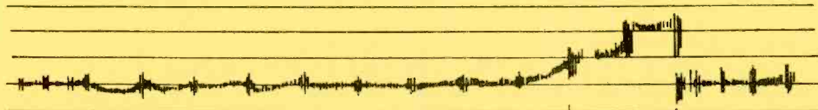
TYPICAL VECTORSCOPE DISPLAY FOR DIFFERENTIAL PHASE
