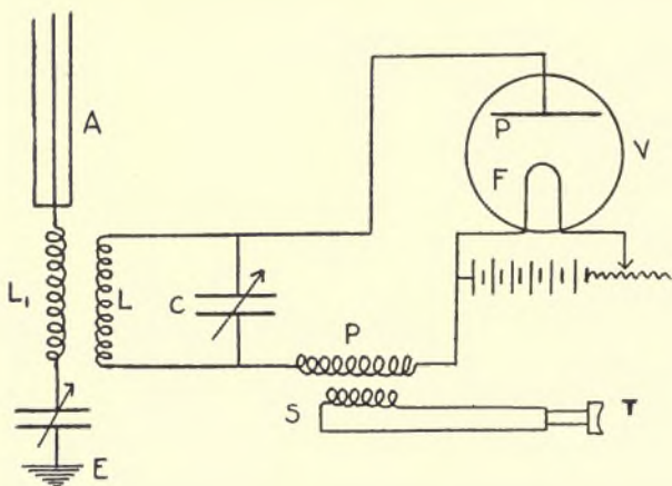
FIG. 101.—CONNECTIONS FOR USE OF FLEMING VALVE AS A SIMPLE RECTIFIER DETECTOR IN A RADIOTELEGRAPHIC RECEIVER.
