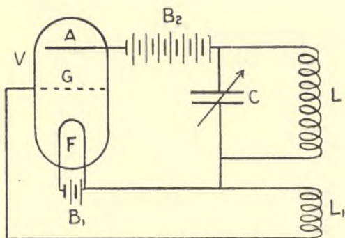
FIG. 83.—Schematic of Circuits for using a Three-electrode Valve, V , as a Generator of Oscillations by inter-coupling Grid and Plate Circuits by Mutual Inductance Coils, L , L_1 .
