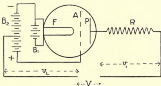
FIG. 90.—The Dynatron as a Voltage Magnifier when used in Series with a Resistance, R .
