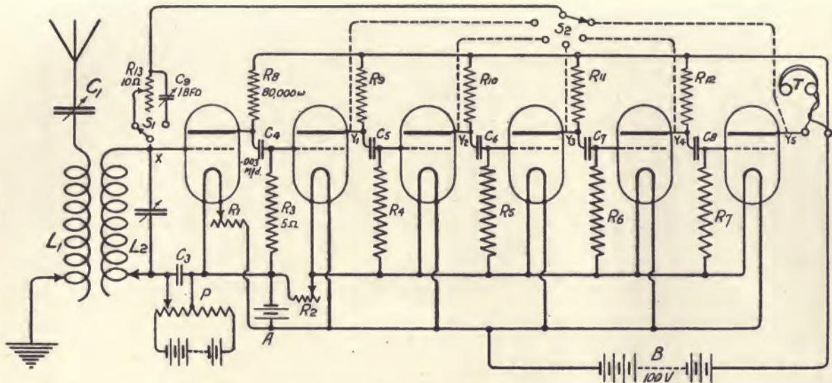
FIG. 136.—Receiving arrangement comprising six Thermionic Valves in Cascade, coupled through high resistances and condensers. A is the Filament Heating Battery, and B is the Plate Battery.
