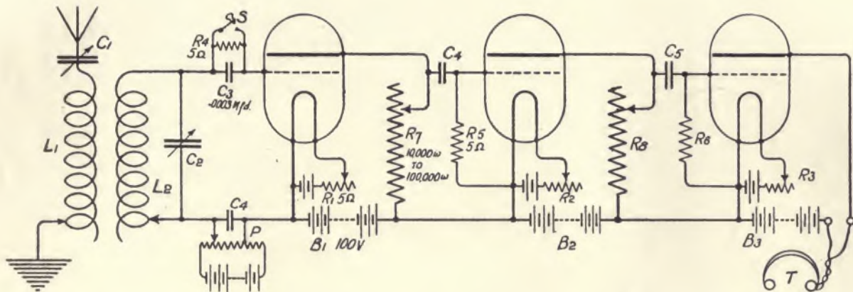
FIG. 133.—Receiving arrangement of Valves in Cascade coupled through high resistances. (J. Scott-Taggart.)
