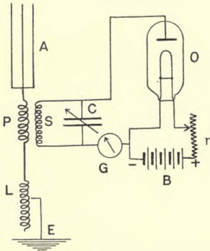
FIG. 29A.—SCHEME OF CONNECTIONS FOR USE OF AN OSCILLATION VALVE AS A DETECTOR IN WIRELESS TELEGRAPHY. A , Aerial Wire. P , S , Jigger. C , Tuning Condenser. O , Oscillation Valve. B , Valve Battery. r , Rheostat. G , Galvanometer or current-detecting instrument.
