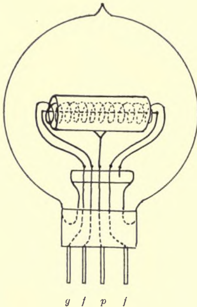
FIG. 67.—SPIRAL AND CYLINDER THREE-ELECTRODE VALVE.
