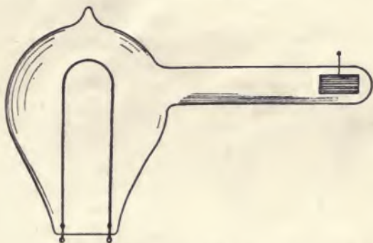
FIG. 5.—Collecting Plate placed at the end of a side tube opening out of the bulb of an incandescent lamp.
