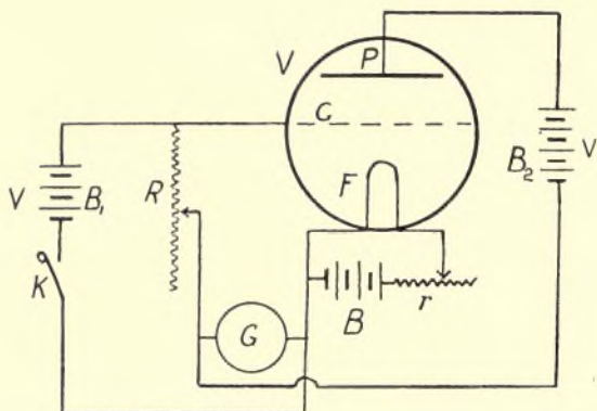
FIG. 79.—Arrangement of Circuits for Measuring Slope of Characteristic Curve. (Captain E. V. Appleton.)
