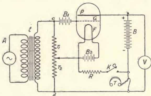
FIG. 142.—Method of J. M. Miller for Measuring the Amplification Factor R_i and internal resistance of a Thermionic Valve.
