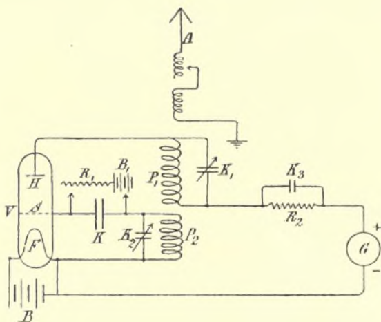
FIG. 124.—Arrangement of Circuits due to Captain H. J. Round, Using a Three-electrode Valve for the Production of Undamped Electric Oscillations in Radiotelephonic Transmitters.
