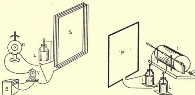
FIG. 25.—ARRANGEMENTS FOR EXHIBITING THE RECTIFYING POWER OF AN OSCILLATION VACUUM VALVE.
