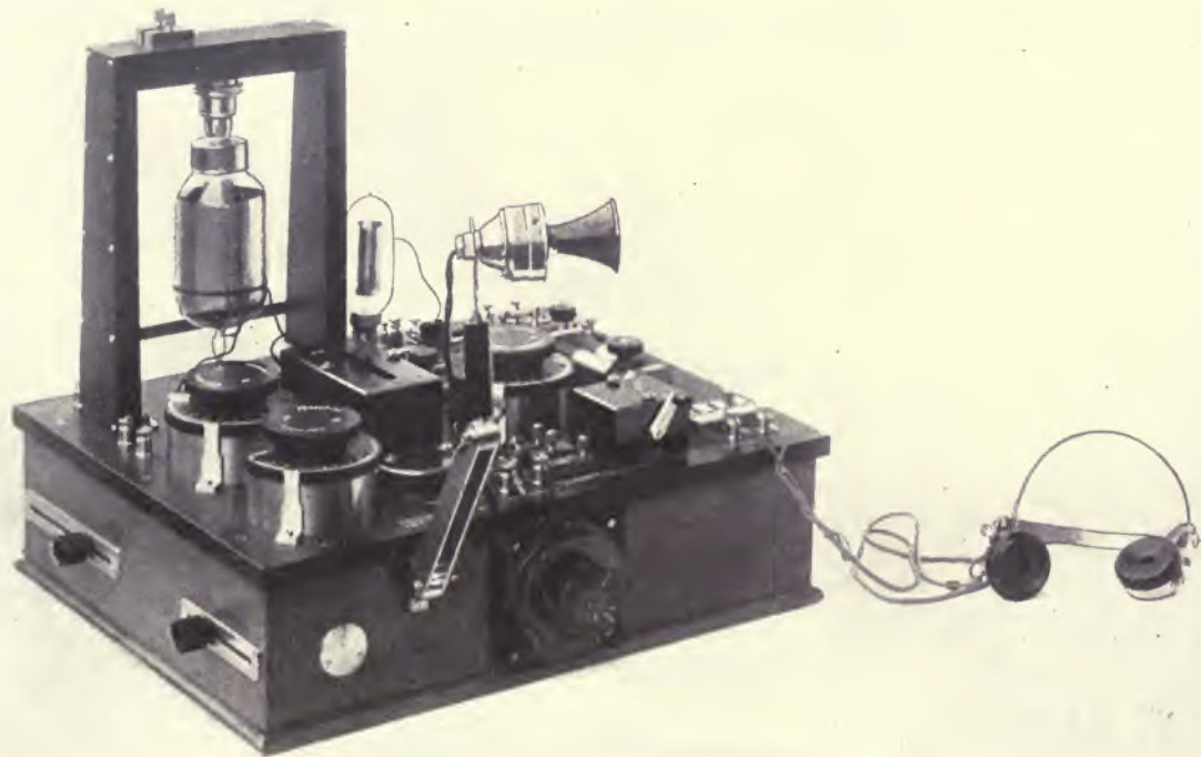
FIG. 126.—Photograph of Wireless Telephone Apparatus Constructed and Used by Marconi's Wireless Telegraph Company, Ltd. (H. J. Round.)
