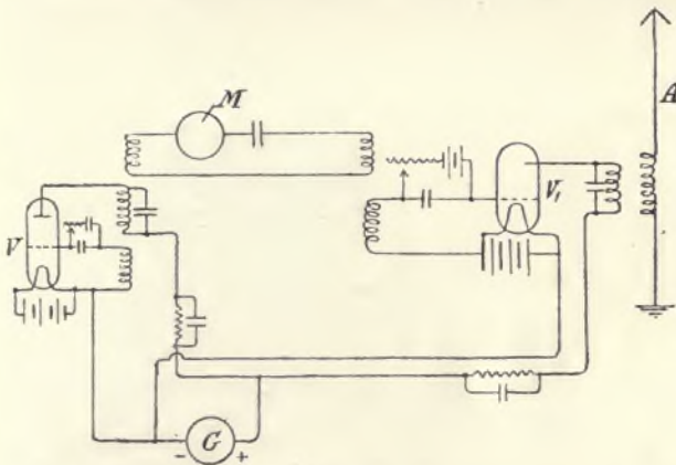
FIG. 125.—Arrangement of Circuits Employing Two Three-electrode Valves, due to Captain H. J. Round, for Production of Undamped Oscillations for Radiotelephony, the Amplitude being Controlled by a Microphone, M , in an Intermediate Circuit.
