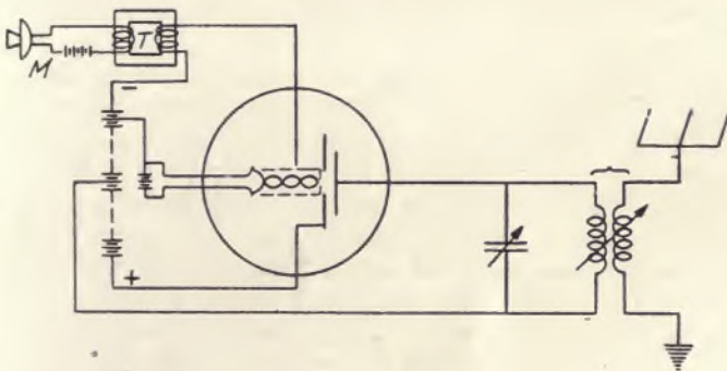
FIG. 127.—Scheme of Circuits for a Radiotelephonic Transmitter Employing a Pliodynatron, made by the General Electric Company of U.S.A., as Oscillation Generator.
