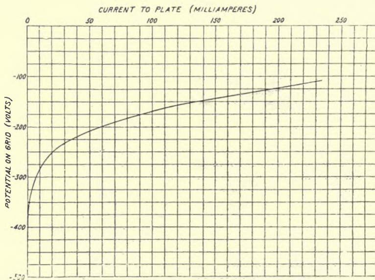
FIG. 70.—Part of Characteristic Curve of Large Pilotron.
