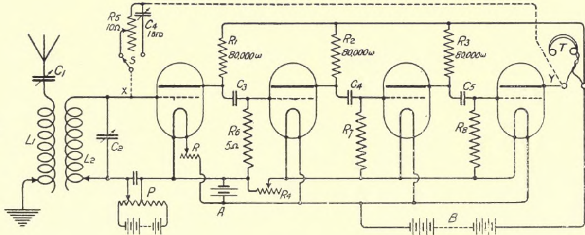
FIG. 135.—Receiving arrangement of great efficiency, comprising four Thermionic Valves in Cascade, coupled through high resistances.
