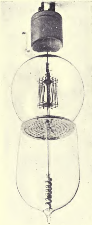
FIG. 72.—Perspective view of Lieben-Reisz Thermionic Relay.
