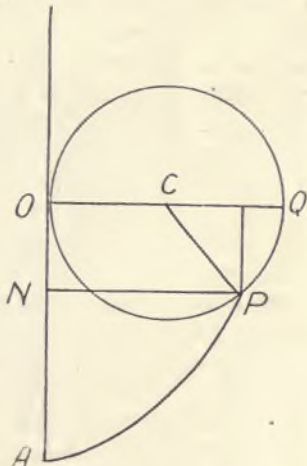
FIG. 21. — Generation of a Cycloid.
