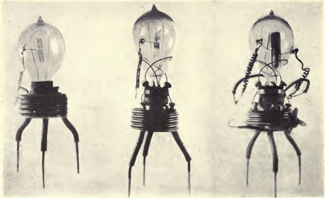
PHOTOGRAPHS OF THE OSCILLATION VALVES FIRST EMPLOYED BY DR. J. A. FLEMING, F.R.S., IN OCTOBER, 1904, FOR THE RECTIFICATION OF HIGH-FREQUENCY ELECTRIC OSCILLATIONS AS USED IN WIRELESS TELEGRAPHY
