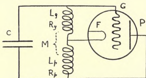
FIG. 99.—Scheme of Connections of Three-electrode Thermion, Coupled to a Single Oscillatory Circuit.
