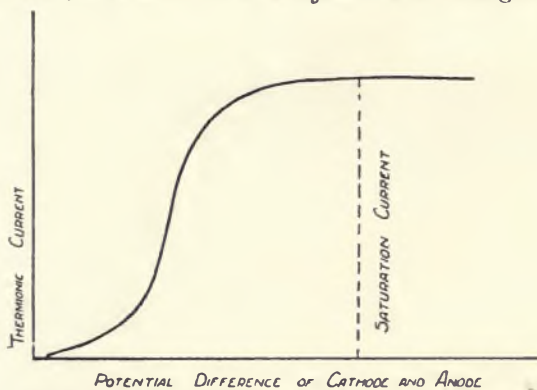
FIG. 23.—Characteristic or Volt-ampere Curve of a highly rarefied gas or nearly perfect vacuum space.
