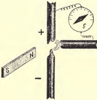
FIG. 14.—An electric arc projected by means of a magnet against a third carbon to show the "Edison effect" in the case of an electric arc.
