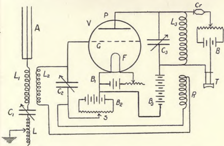
FIG. 107.—Connections for use of a Three-electrode Valve as an Amplifying Relay in Conjunction with a Crystal Detector, Cr, and Telephone. T.
