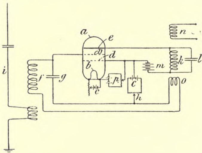
FIG. 121.—Connections of Method due to G. M. Wright for Eliminating or Reducing Atmospherics Depending upon Current-limiting Power of the Thermionic Valve.
