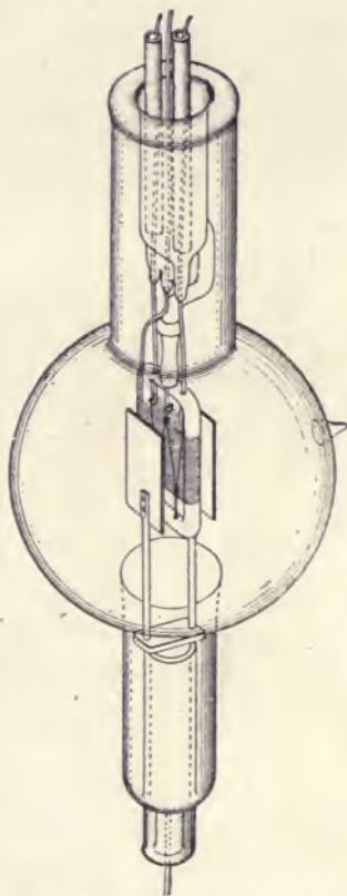
FIG. 69. — High Vacuum Thermionic Amplifier, called a large Pliotron.
