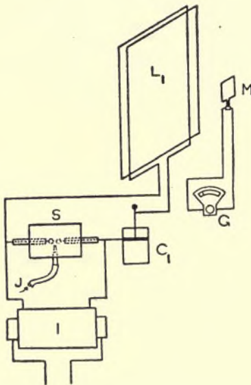
FIG. 47.—SCHEME OF CONNECTIONS OF PRIMARY OSCILLATION CIRCUIT IN THE AUTHOR'S VALVE - TESTING ARRANGEMENT.
