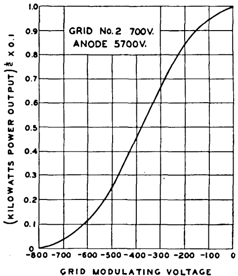
Fig. 11— Modulation characteristics.
