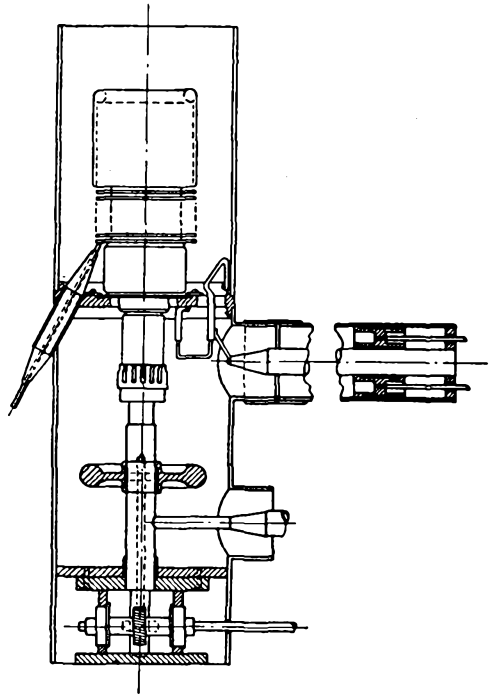
Fig. 4—Cross section of the "half-wave" oscillator circuit.
