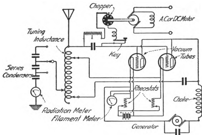
Transmitter No. 5. A radio telegraph outfit using continuous waves.
