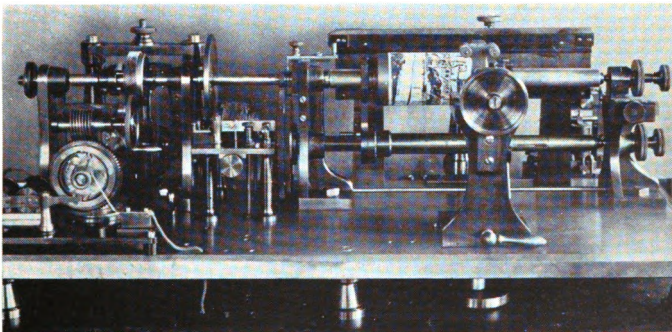
A close-up view of the Belin photographic transmitter used to send the picture shown above
