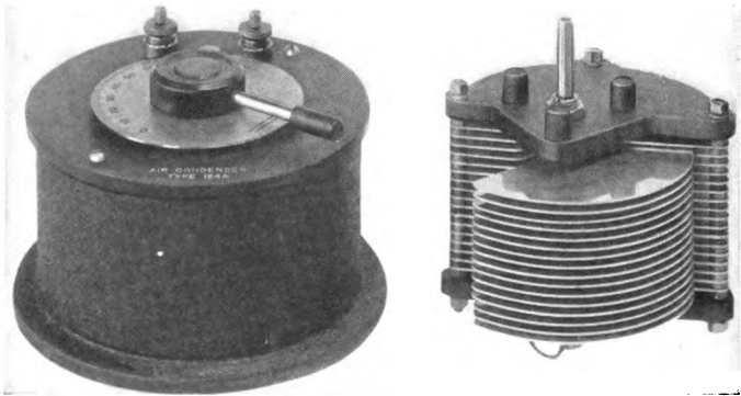
The type of variable condenser used in radio receiving circuits
