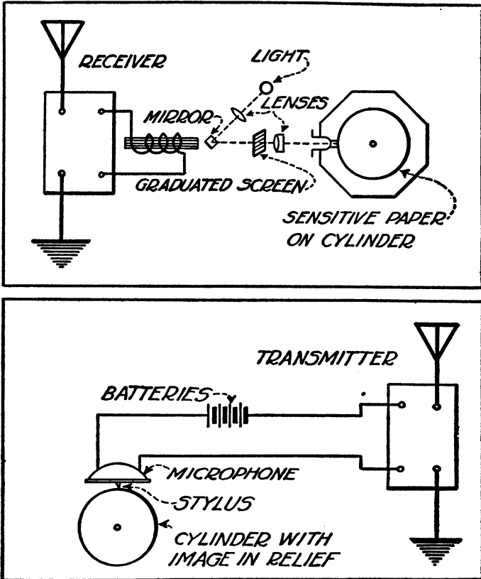
A diagram of the transmitting and receiving apparatus used in the Belin system.
