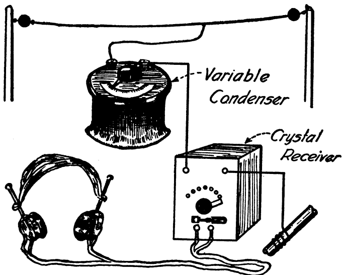
How a variable condenser is connected between the aerial and receiving outfit to reduce the wave-length.
