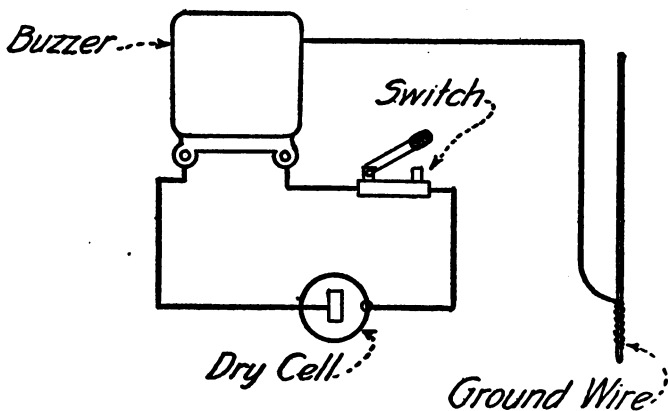
Details of a buzzer testing outfit used in the adjustment of crystal detectors.
