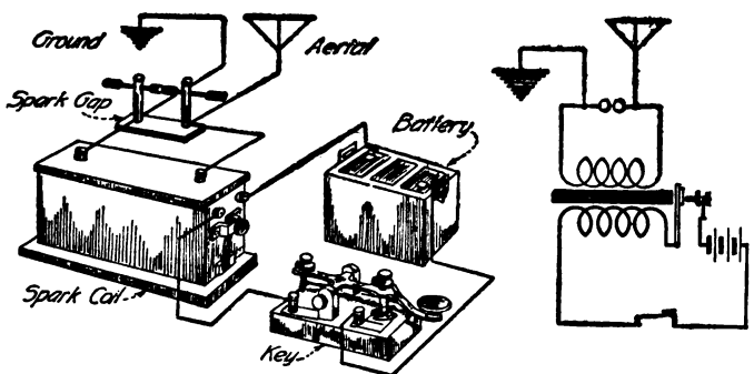
The instruments necessary for a simple radio telegraph transmitter. Diagram of connections is shown at the right
