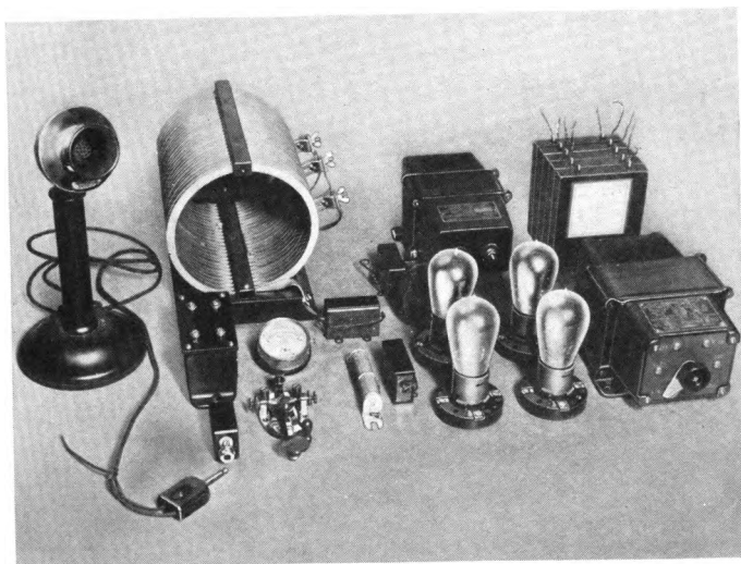
Necessary apparatus for a twenty-watt vacuum tube telephone transmitter
