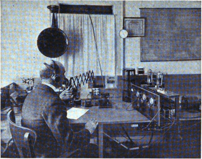
A typical amateur station equipped with a vacuum tube radiophone transmitter
