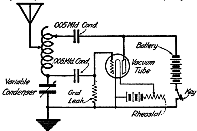
Transmitter No. 3. An outfit employing a single five-watt transmitting vacuum tube.
