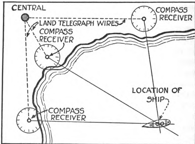
Showing how the radio compass functions.
