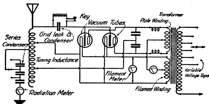
Transmitter No. 4. A ten-watt combination telegraph transmitter.
