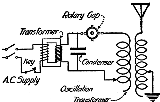
Transmitter No. 2. A powerful transmitter employing a transformer and operating from the electric light circuit.
