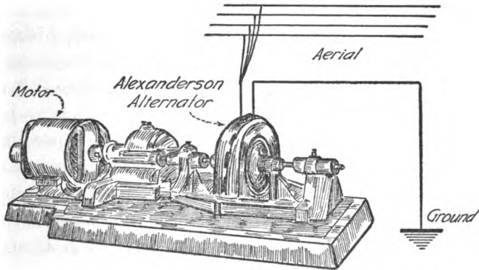
The Alexanderson high-frequency alternator now used in trans-oceanic radio communication.
