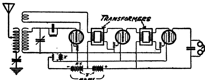
Connections for a two-stage vacuum tube amplifier using the regenerative principle. This is receiving outfit No. 7.
