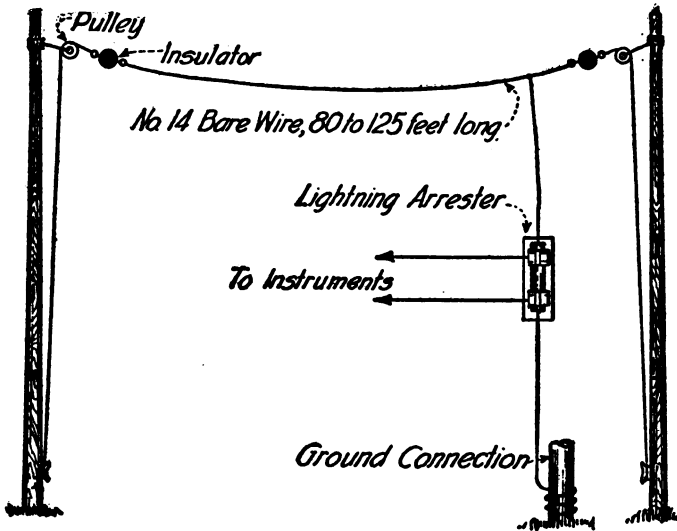
Constructional details of a simple one-wire aerial.
