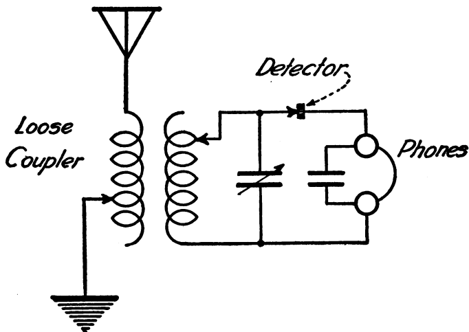
How the loose coupler is used in receiver No. 3.
