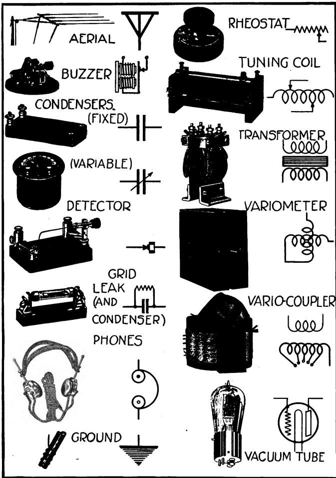
Instruments used in radio receiving outfits and the diagrammatic symbols
