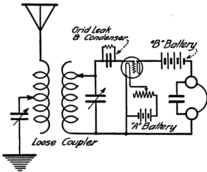
A simple vacuum tube receiver employing the grid leak and grid condenser. This is receiving outfit No. 5.
