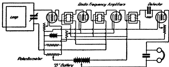
Connections for a radio-frequency amplifier using the loop or indoor antenna. This is receiving outfit No. 8.
