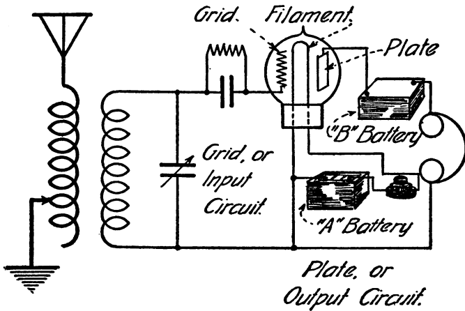
How the three-element vacuum tube of De Forest is used in a receiving circuit.
