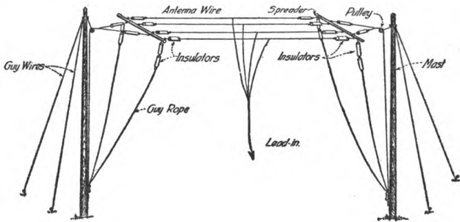
Constructional details of a large four-wire aërial suitable for general amateur use.
