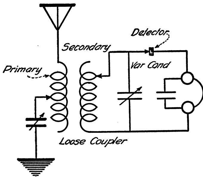
How two variable condensers are used in receiver No. 4.
