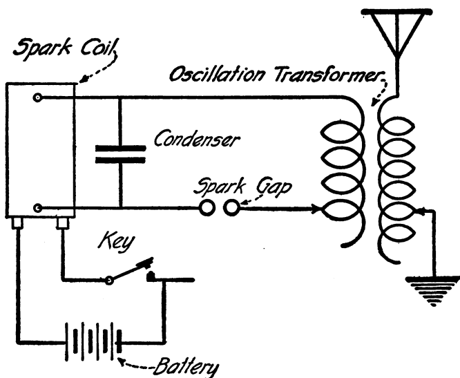
Transmitter No. 1. This is a simple outfit employing a spark coil.
