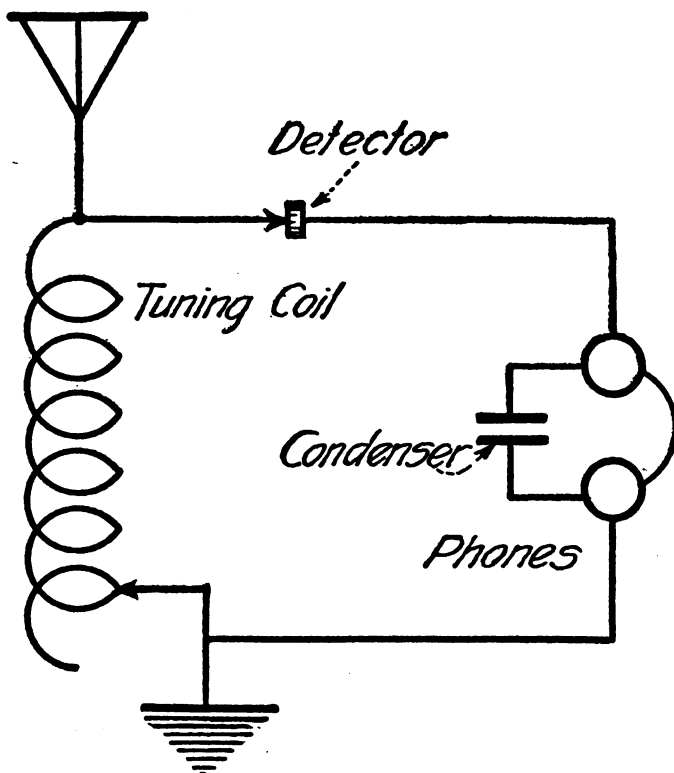
Connections of crystal receiving outfit No. 1.
