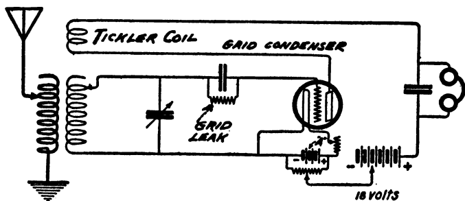
A tickler-coil or regenerative receiver with grid leak and grid condenser.
