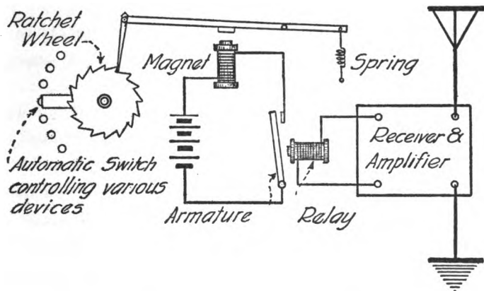
This diagram illustrates the principle of radiodynamics.
