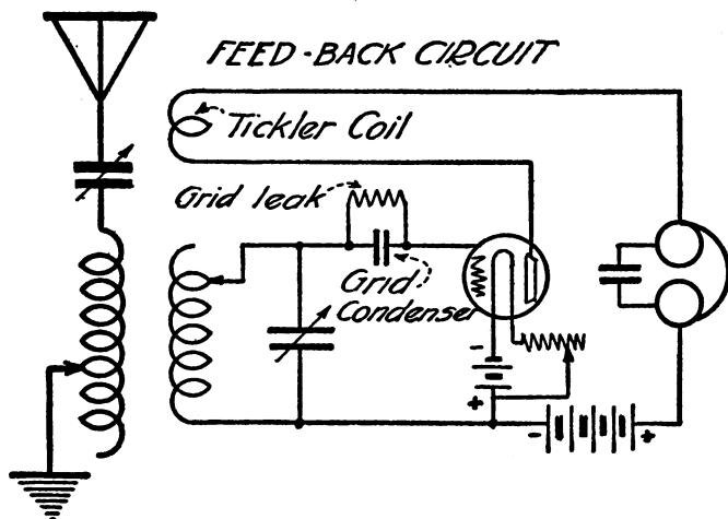
• Connections for a regenerative vacuum tube receiver No. 6.
