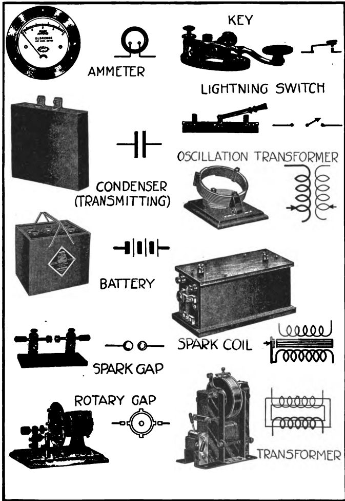
Instruments used in radio transmitters and their diagrammatic symbols
