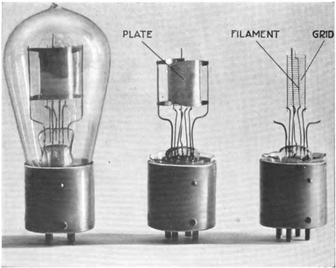
The various parts of a vacuum tube
