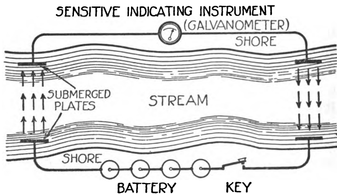
One of the early ground "wireless" systems used in this country for communication over short distances.
