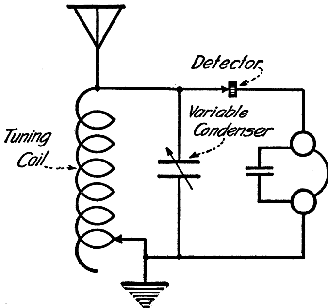
Crystal receiver outfit No. 2 with a variable condenser.
