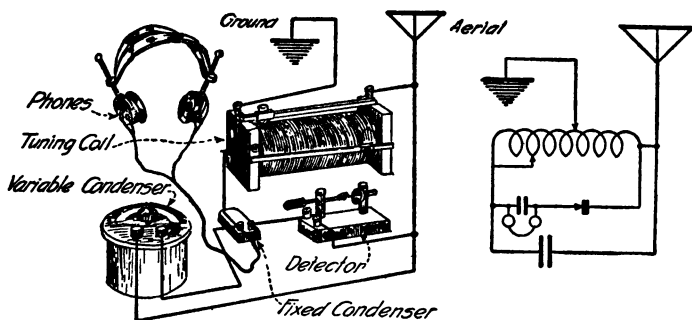
The instruments used in a simple radio receiving outfit.
