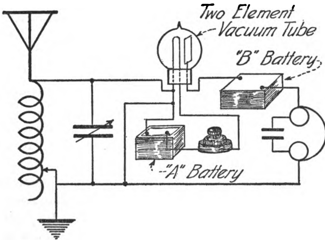
How the two-element vacuum tube is connected in a radio receiving circuit.
