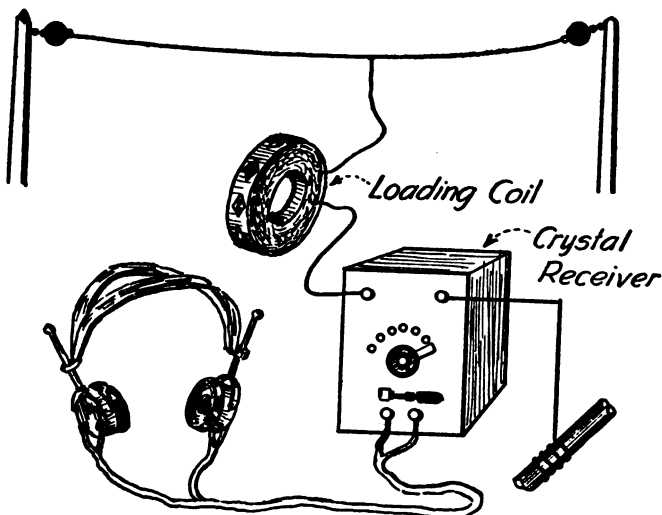
How a loading coil is connected between the aerial and ground of a crystal receiver to increase the wave-length.
