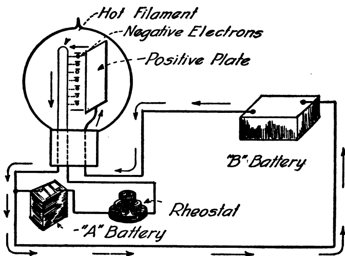
Diagram showing principle of the two-element vacuum tube.
