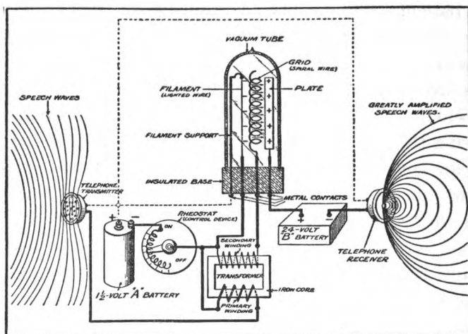
A diagrammatic explanation of the operation of the vacuum tube amplifier for the deaf.
