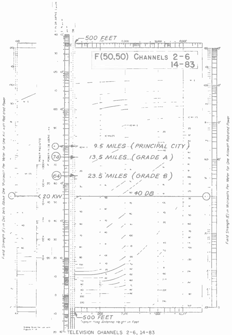
Fig. 2-6. Use the scale supplied with the FCC's F(50,50) chart to determine coverage. 50, 50 indicates that the estimated field strength is exceeded at 50 per cent of the potential receiver locations for at least 50 per cent of the time.
