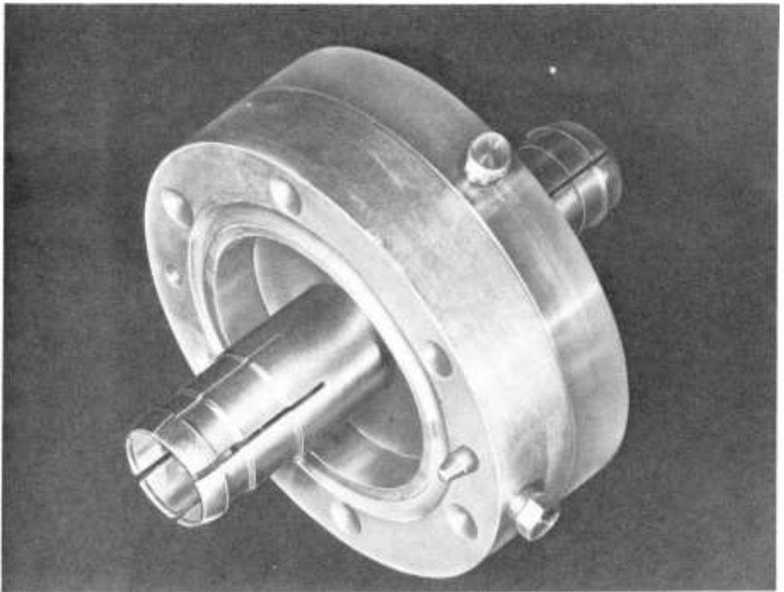
Fig. 6-16. A gas block or barrier for 3/16-inch coaxial line.
