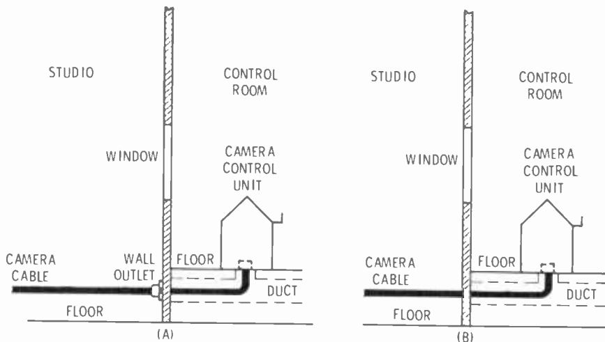
Fig. 10-8. Camera cable connections: (A) Connected to wall outlet; (B) Run through the wall directly to the control unit.
