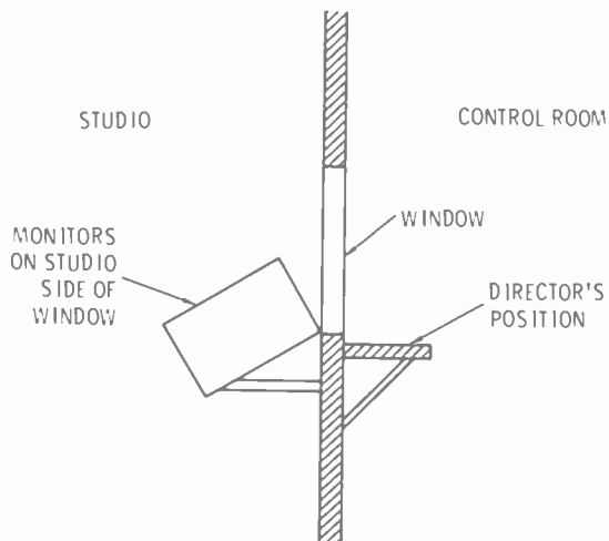
Fig. 10-6. For the director's position, video monitors may be mounted in this fashion on the studio side of the control room.
