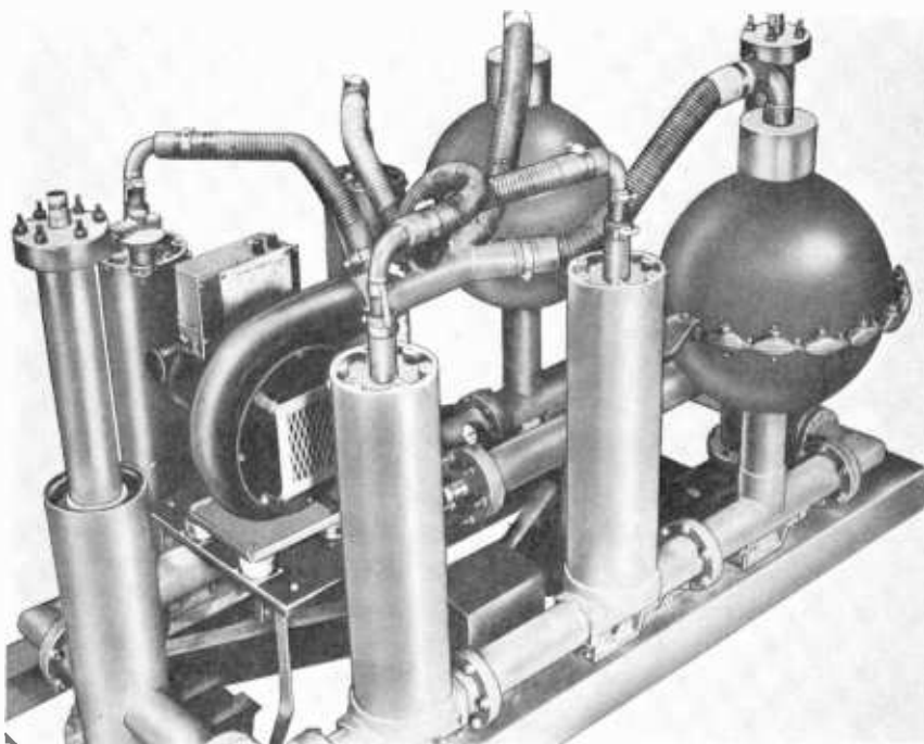
Fig. 5-20. The complete filterplexer. (RCA)
