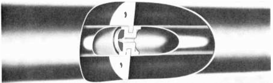
Fig. 6-1. The cut-away view of a teflon insulator in a coaxial transmission line. (RCA)
