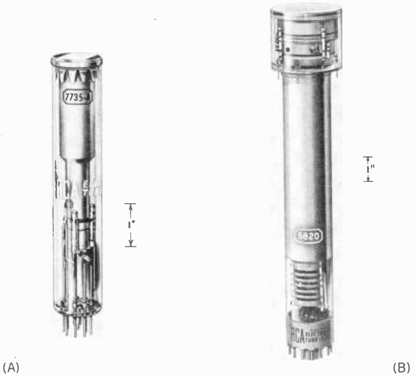
Fig. 3-17. (A) A 1-inch diameter vidicon tube. (B) A 3-inch diameter image orthicon tube. (RCA, Tube Division)
