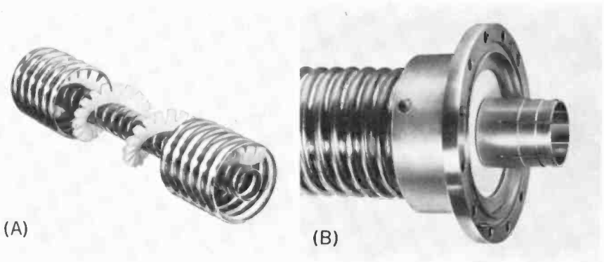
Fig. 6-6. Heliax cable: (A) 3-inch—notice the continuous insulator; (B) 5-inch, fitted with a standard 6-1/8-inch diameter EIA flange. (Andrew Corp.)
