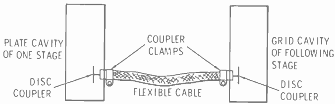
Fig. 5-11. Cavities are connected with disc couplers and flexible cable.
