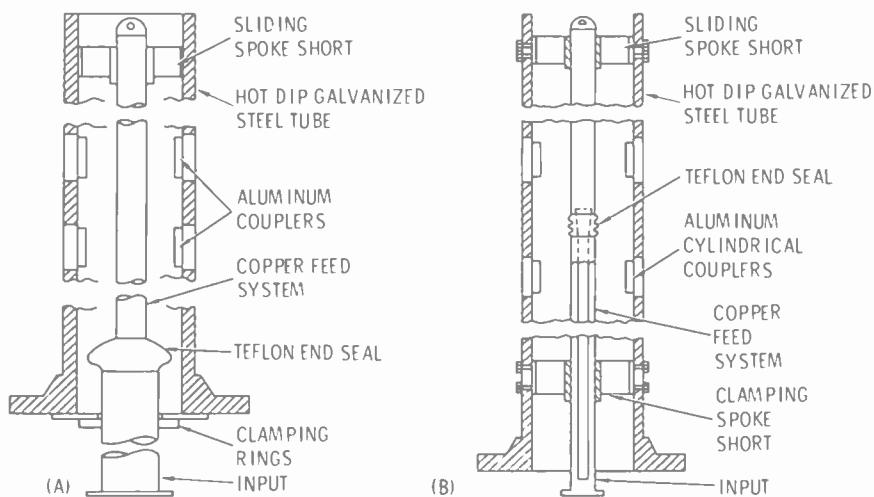
Fig. 7-15. Two methods of feeding r-f energy to different RCA antenna models: (A) the end-fed antenna; (B) the center-fed antenna. (RCA)
