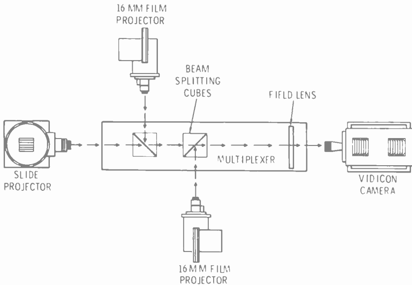
Fig. 4-5. A film camera chain with a single camera, projection equipment, and multiplexer.
