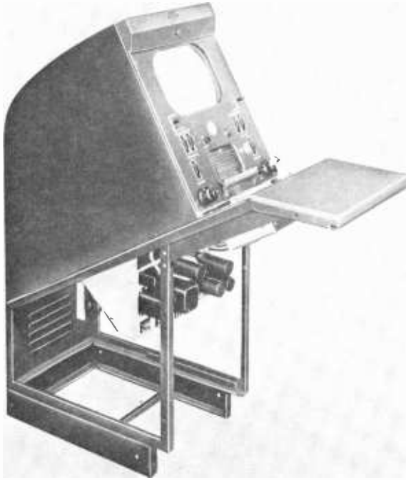
Fig. 4-8. The RCA TS-5A video switcher mounted in a standard console housing with a master monitor. In this arrangement, the fader pushbutton assembly is mounted in the well of the console. (RCA)
