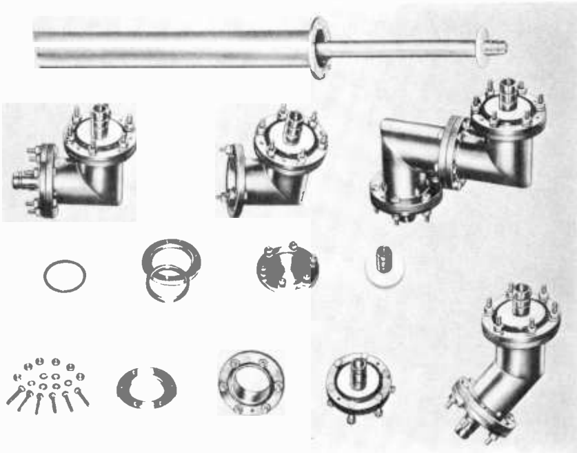
Fig. 6-3. The various mitered elbows and other fittings of standard 3-1/8-inch teflon line. (RCA)
