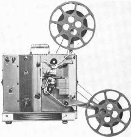
Fig. 8-13. A small 16 mm projector, the RCA 400 Jr., suitable for film previewing. (RCA)
