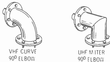
Fig. 6-2. Comparing the uhf mitered elbow and the vhf curved elbow.
