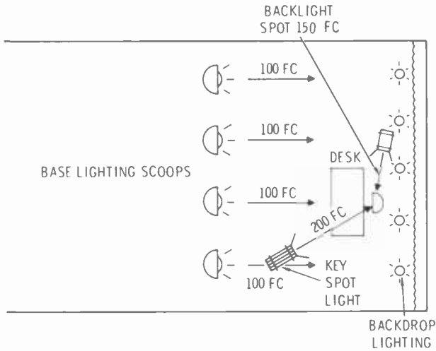
Fig. 3-5. The basic lighting elements with light intensities indicated: key, back, base, and backdrop.
