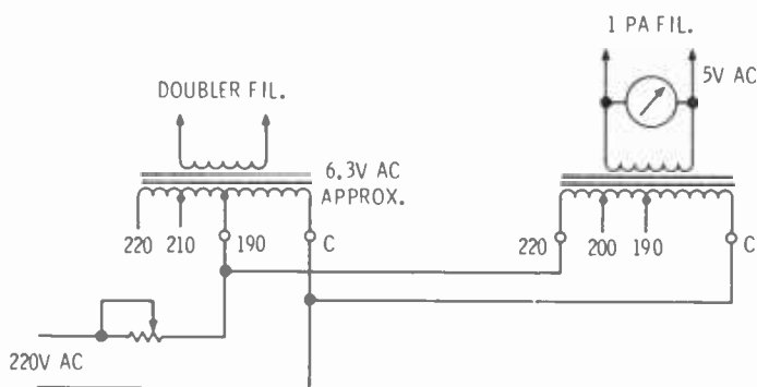
Fig. 5-24. Change the filament transformer primary taps to get correct voltage on your old doubler tube and new 1PA tube.
