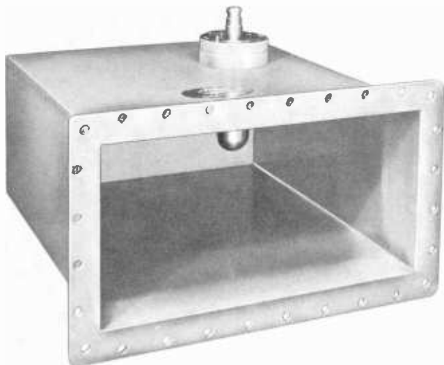
Fig. 6-19. A transition from waveguide to rigid transmission line. (Andrew Corp.)
