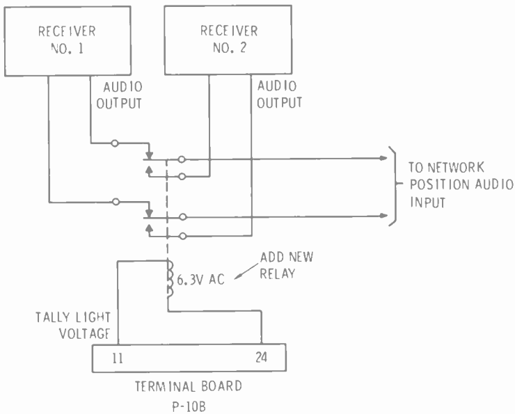
Fig. B-4. TC-4A modifications to operate two off-air receivers' audio into one switch position of the console.
