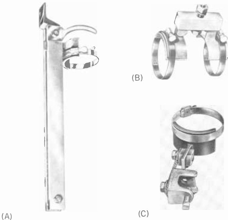
Fig. 6-13. (A) A spring hanger; (B) A rigid clamp to anchor the line at the top of the tower; (C) A grounding clamp, used when the line is insulated and some sections are to be grounded. (Andrew Corp.)
