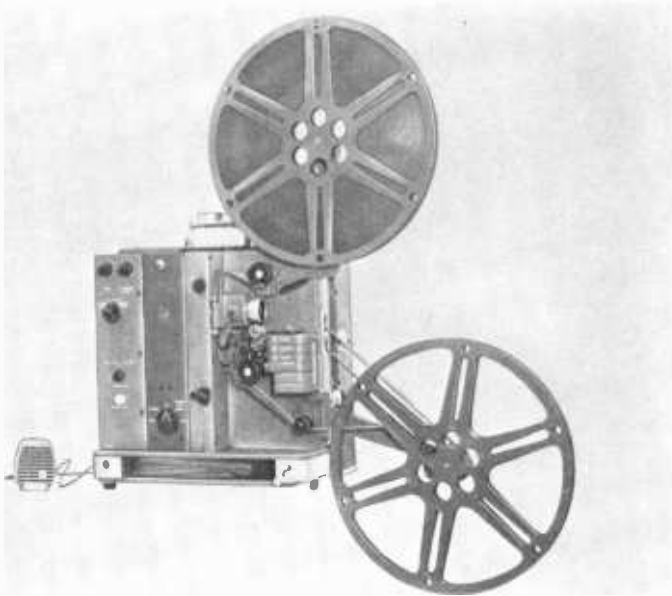
Fig. 8-14. A small 16 mm projector, the RCA 400 Magnetic, suitable for previewing film with optical or magnetic sound tracks. This projector is also a magnetic recorder. (RCA)
