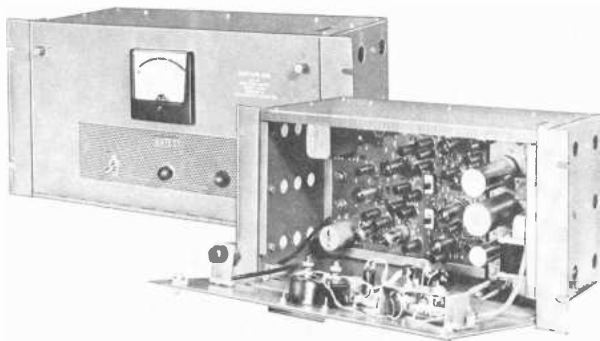
Fig. 4-15. The "Level Devil," an audio age amplifier: (rear) with its panel closed; (front) with its panel opened. (Gates Radio Company)
