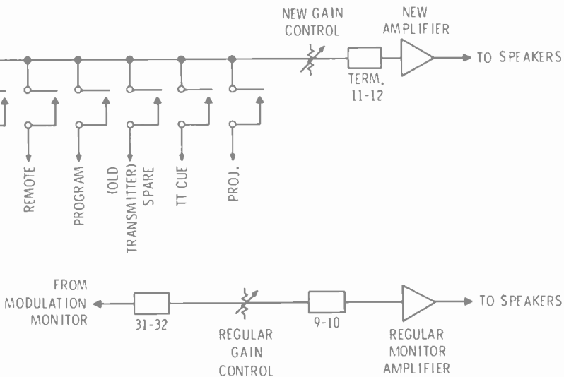
Fig. B-5. TC-4A modifications to separate regular air monitoring so that it is in operation at all times. Addition of fader and amplifier so that all cue positions may be monitored without bothering the regular speaker system.
