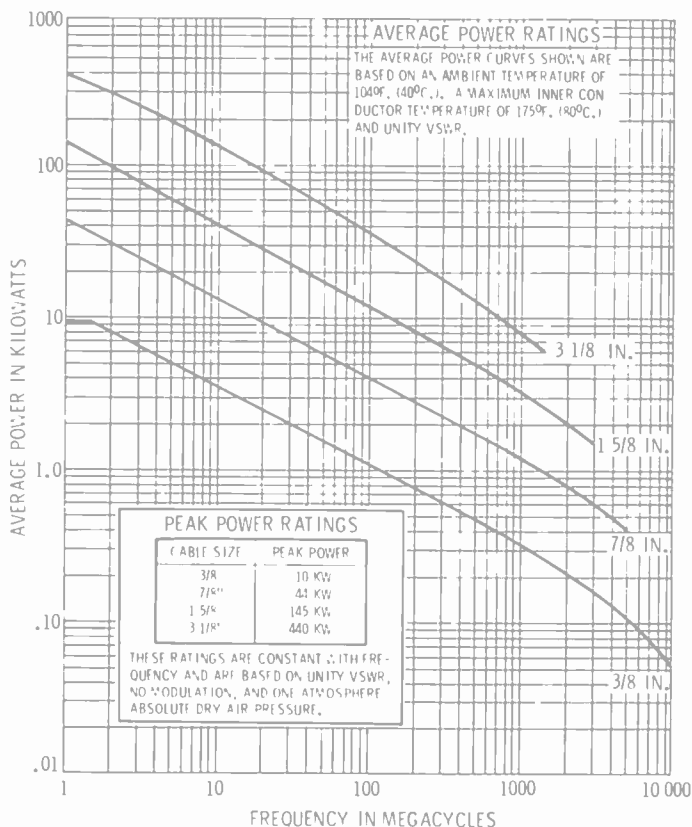
Fig. 6-8. Average power ratings for 50 ohm heliax. (Andrew Corp.)
