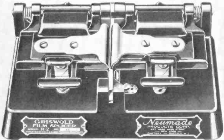
Fig. 8-11. A manual, 16 mm film splicer. (Neumade Products Corp.)
