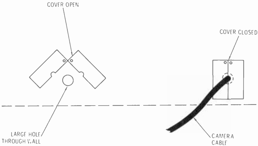
Fig. 10-9. A cover should close off the hole when the cable runs into the control room.
