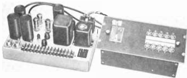
Fig. 4-7. The RCA TS-5A video switcher, lap-dissolve unit. (RCA)
