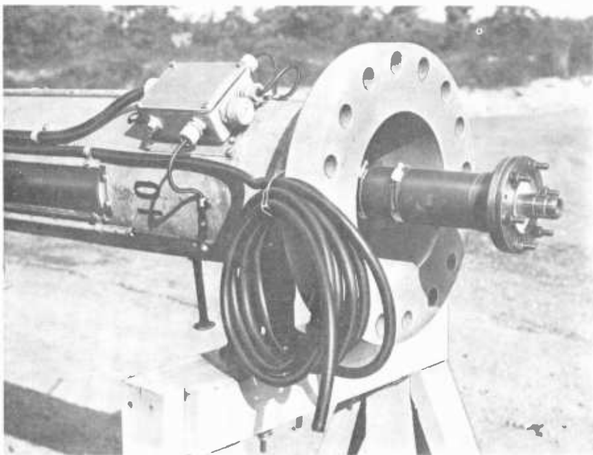
Fig. 7-14. The coaxial feedpoint is prominent at the base of the uhf pylon antenna. Also shown are the cable to the beacon light and the junction box for the heaters. (RCA)
