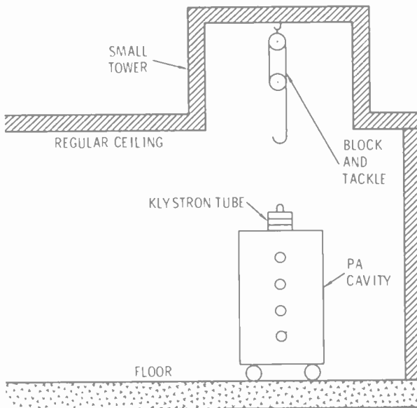
Fig. 9-4. If the transmitter room ceiling is too low, a small tower should be built to facilitate replacement of klystron tubes.
