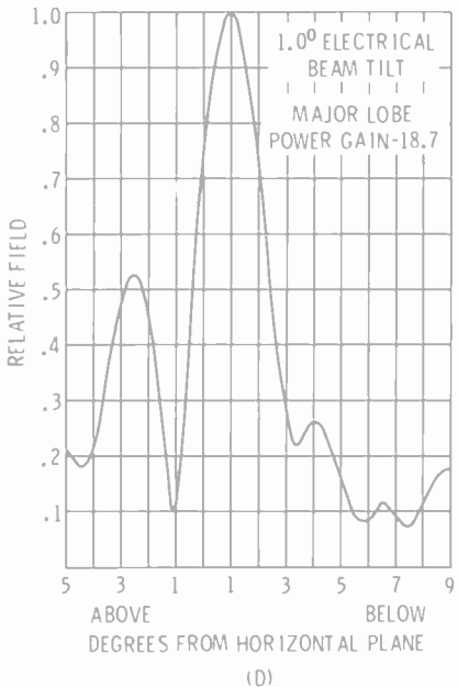
Fig. 7-12. Calculated vertical patterns for the TFU-24DL and TFU-24DM antennas. (RCA)
