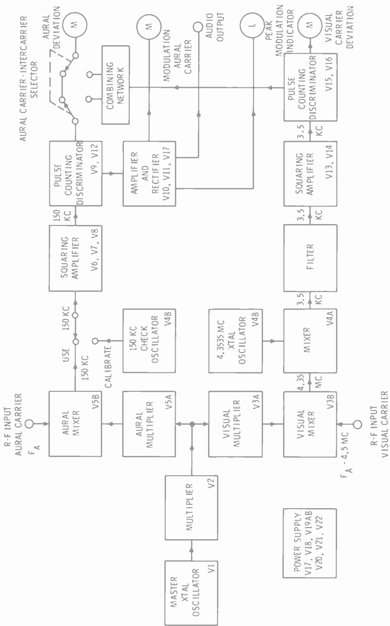
Fig. 5-13. The block diagram of the Heathkit-Packard 535F 'TV' station monitor. (Heathkit-Packard)
