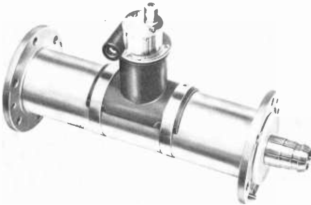
Fig. 5-15. A directional coupler mounted in a short section of 3-1/8-inch transmission line. (RCA)
