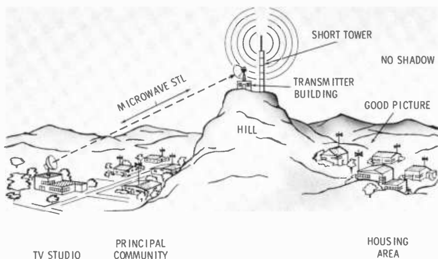
Fig. 1-3. Shadow areas can be eliminated by placing the transmitter on the highest location possible and using microwave between the studio and the transmitter.
