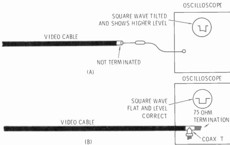
Fig. 11-14. (A) A square wave will be tilted and will read at a high level when the cable is not terminated. (B) With a screw-type termination and T coax connector used as shown the wave will appear and read as it should.
