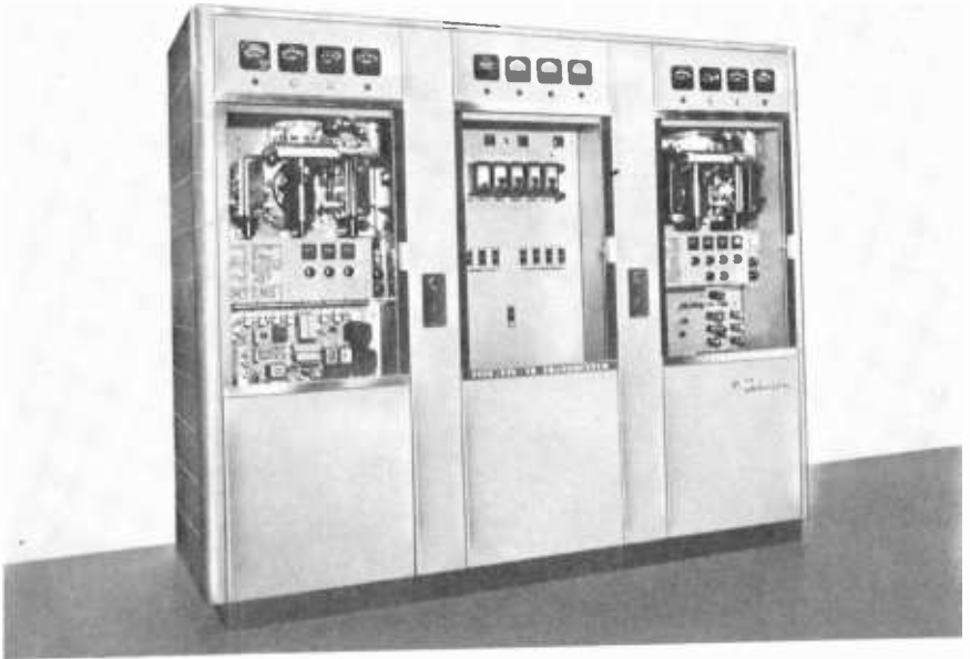
Fig. 5-16. A view of the RCA TTU-1B uhf transmitter with its front doors open. The aural section is on the left; the visual section on the right. (RCA)
