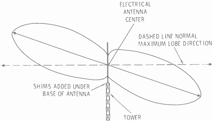
Fig. 7-5. Using mechanical beam tilt, the pattern is raised on one side and lowered on the other.
