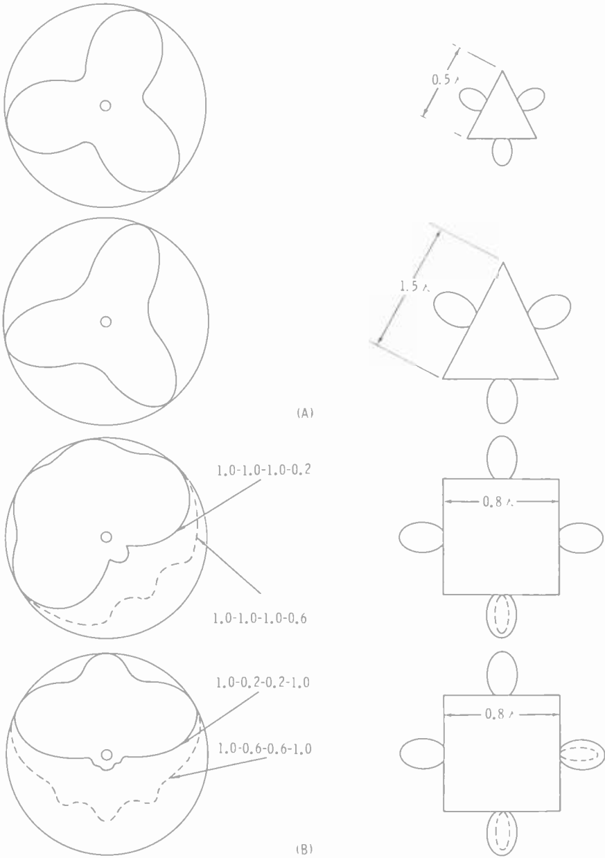
Fig. 7-20. Some of the more than 150 calculated patterns available with the GE zig-zag uhf antenna: (A) Three panels forming an equilateral triangle whose side d varies from 0.5 \lambda to 1.5 \lambda in 0.1 \lambda steps ( d = 2.0 \lambda, 2.5 \lambda, 3.0 \lambda ); (B) Four panels forming a square of 0.8 \lambda side. (GE)
