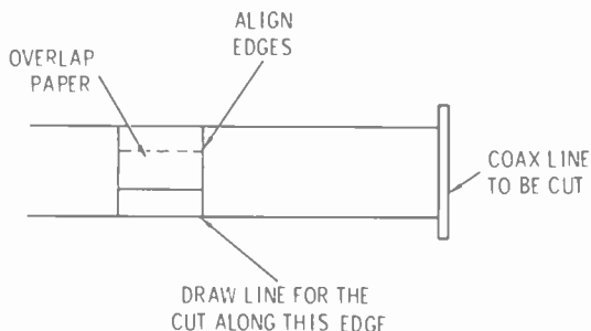
Fig. 6-10. Mark coax line with a piece of paper as your guide in order to ensure a perfect circular cut.
