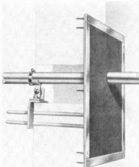
Fig. 6-15. The horizontal anchor and building entrance. This rigidly anchors the horizontal run at the building. (Andrew Corp.)
