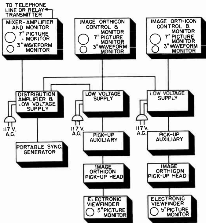
Figure 71. Block diagram of dual image-orthicon camera chain.
