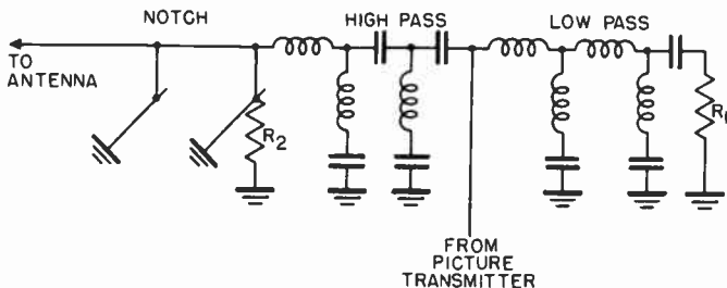
Figure 47. Vestigial sideband filter.
