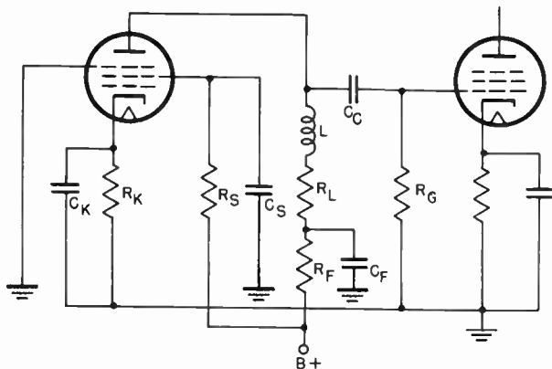
Figure 68. Video amplifier with high and low frequency compensation components.
