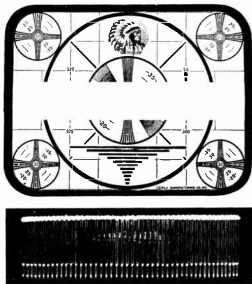
Figure 127. Oscillogram of several horizontal lines and test pattern with marker to indicate portion of pattern used.
