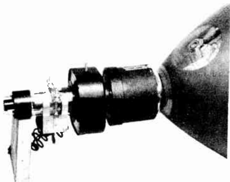
Figure 129. The ion trap magnet is mounted between the tube base and the focus coil.
