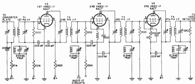
Figure 50. Overcoupled i-f amplifier with wavetraps.
