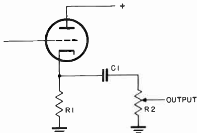
Figure 3. Cathode follower input stage.
