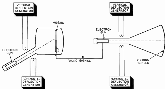
Figure 49. A simplified television system.
