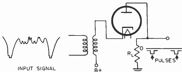
Figure 80. Diode sync clipper.
