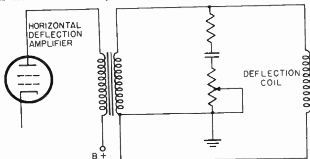
Figure 121. Simplified schematic of damping circuit using resistor and capacitor.
