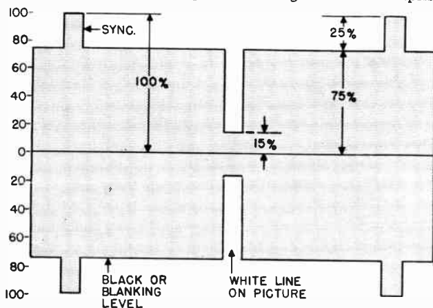
Figure 54. Modulation limits of transmitter.
