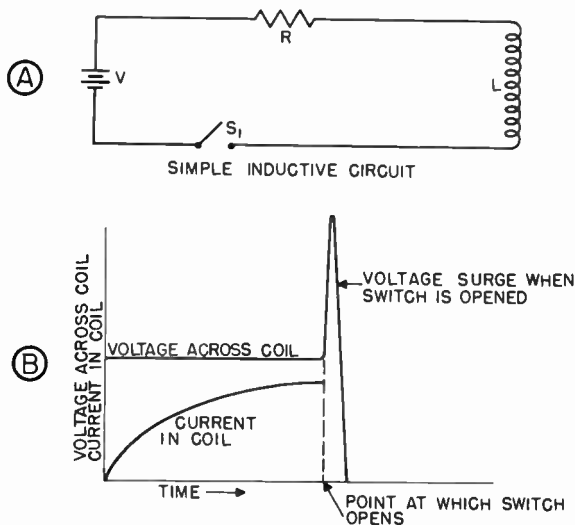
Figure 90. Operation of inductive differentiating circuit.
