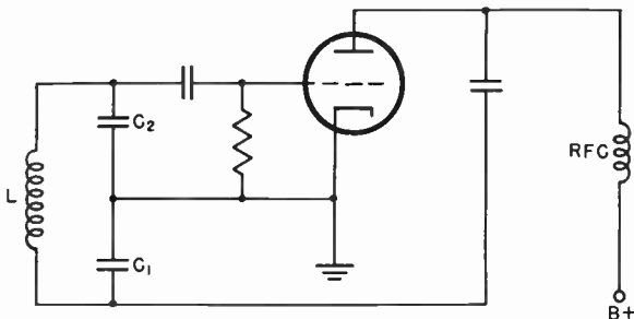
Figure 12. Colpitts oscillator.
