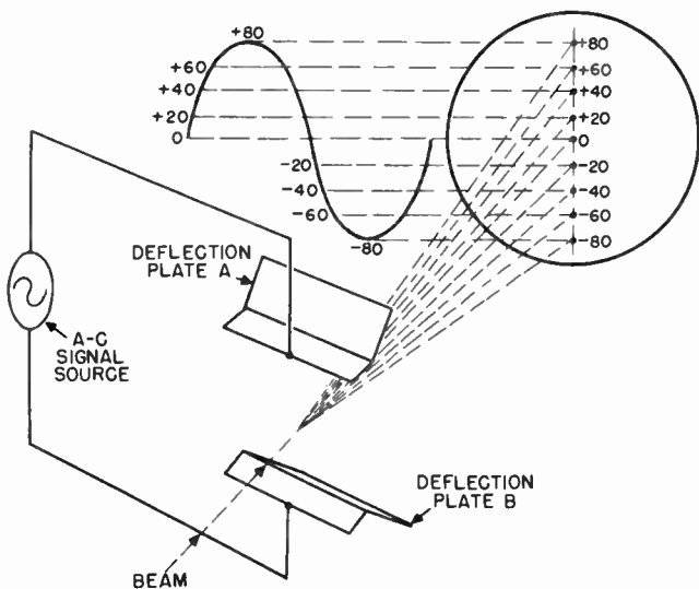
Figure 30. The electron beam traces out a vertical line when a high frequency sine wave is applied to the vertical deflection plates.
