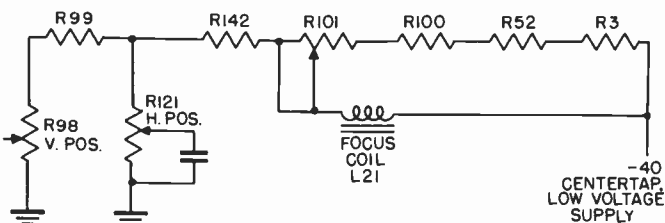
Figure 36. Focus coil circuit.
