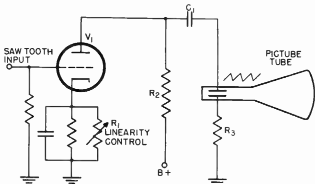
Figure 111. Sweep amplifier for use with electrostatic deflection.
