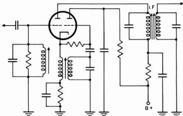
Figure 18. Mixer-oscillator using dual triode with common cathode.
