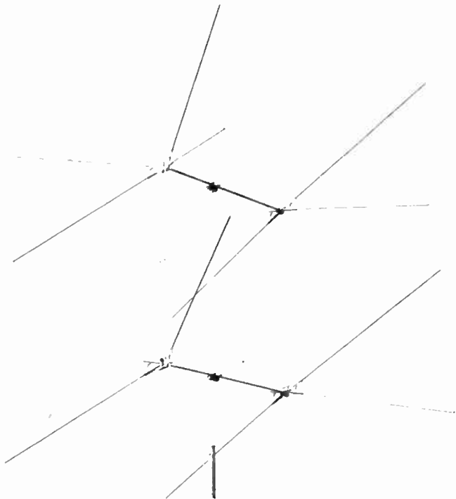
Figure 62. Four-unit double-V stacked antenna. (courtesy Telrex)
