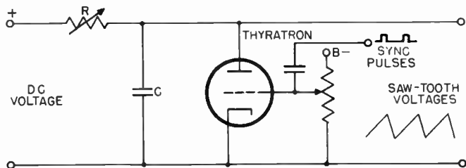
Figure 107. Thyatron saw-tooth generator circuit.
