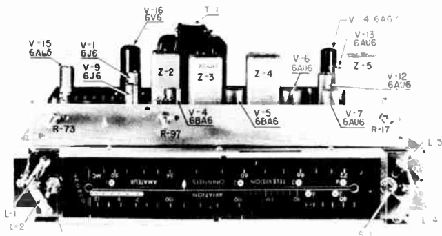
Figure 44. R-F, I-F chassis showing slide-rule dial. (courtesy DuMont)
