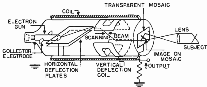
Figure 4. Construction of the orthiconoscope.
