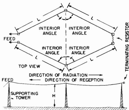
Figure 76. Rhombic antenna.
