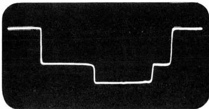
Figure 123. Horizontal blanking and sync pulse.
