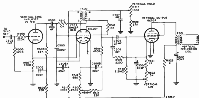
Figure 25. Vertical-deflection circuits.
