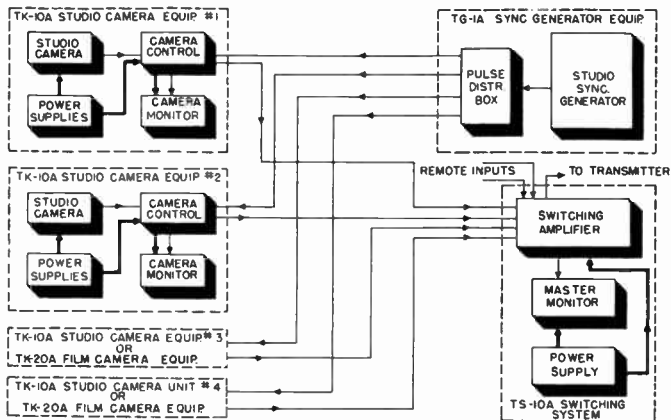
Figure 85. Block diagram of RCA studio camera equipment.
