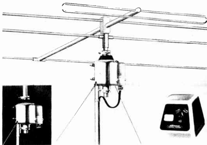
Figure 47. Rotatable antenna. (courtesy Alliance Mfg.)
