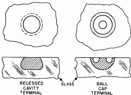
Figure 125. Intensifier terminals.
