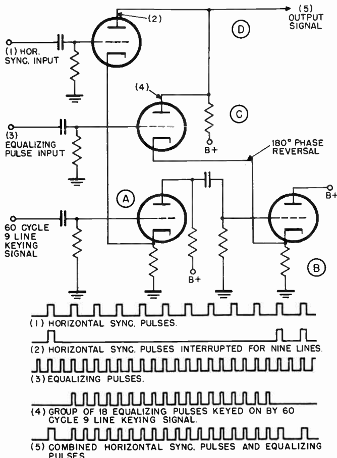
Figure 32. Circuit used to insert equalizing pulses into horizontal sync pulses.
