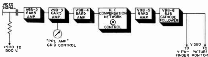
Figure 16. Block diagram of video amplifier used in image orthicon camera.
