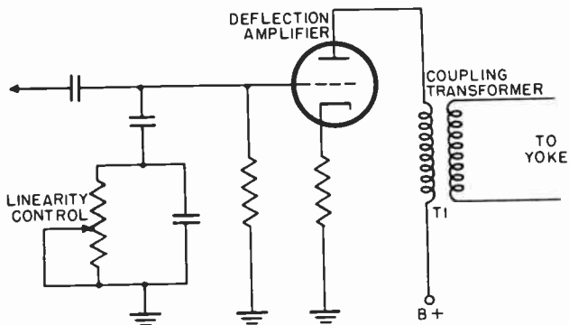
Figure 118. Simplified schematic of deflection amplifier with linearity control.
