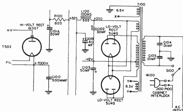
Figure 27. Power supplies.
