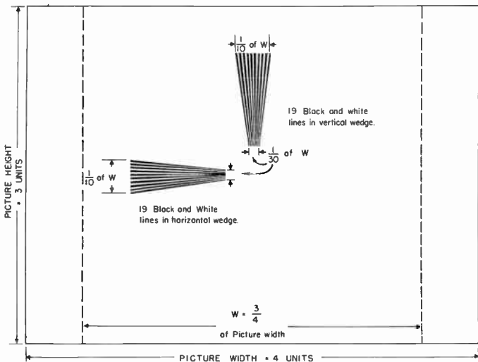
Figure 3. Method used to compute calibration numbers on resolution wedges.
