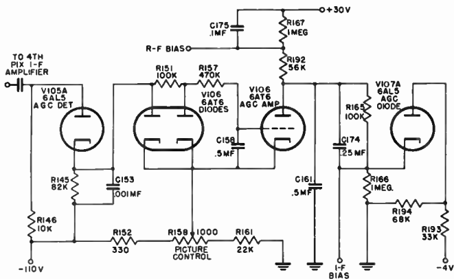
Figure 55. A.G.C. circuit.
