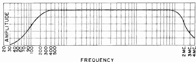
Figure 60. Response curve of video amplifier.
