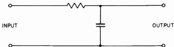
Figure 84. Integrating circuit.
