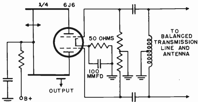
Figure 8. Push-pull r-f amplifier.
