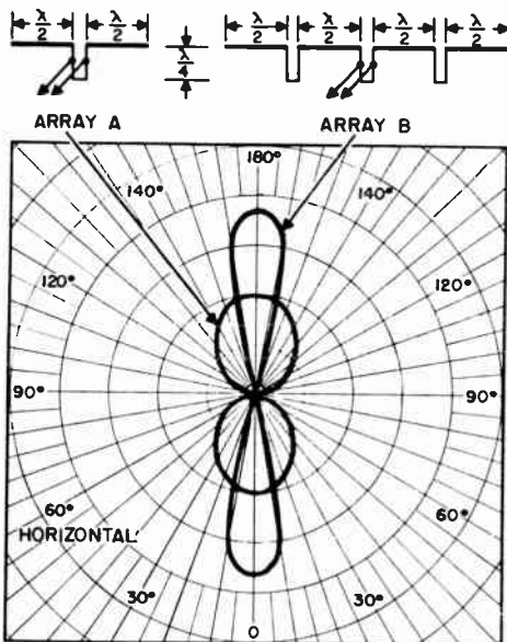
Figure 64. Two types of colinear phased arrays.
