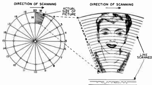
Figure 10. Rotating disc used in Nipkow's television system.
