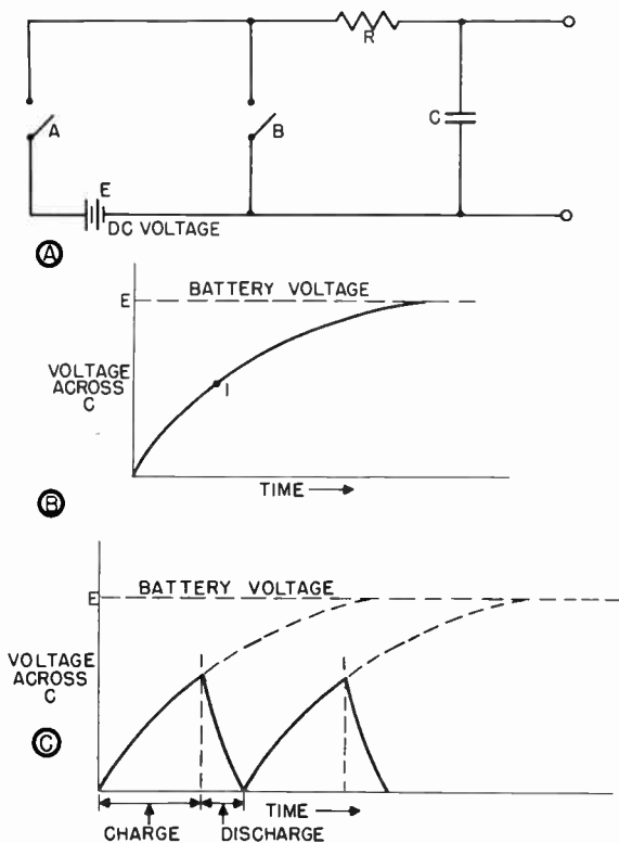
Figure 104. Simple method for producing saw-tooth voltage.
