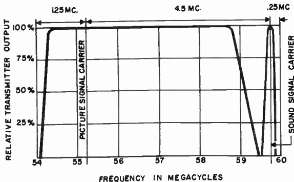
Figure 4. A typical television channel.
