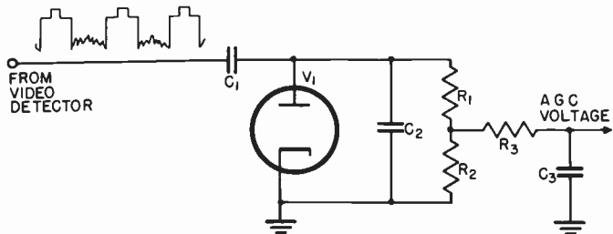
Figure 75. Simplified diagram of a.g.c. circuit.
