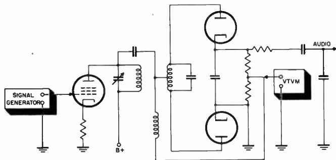
Figure 62. Connections used when checking limiter performance.
