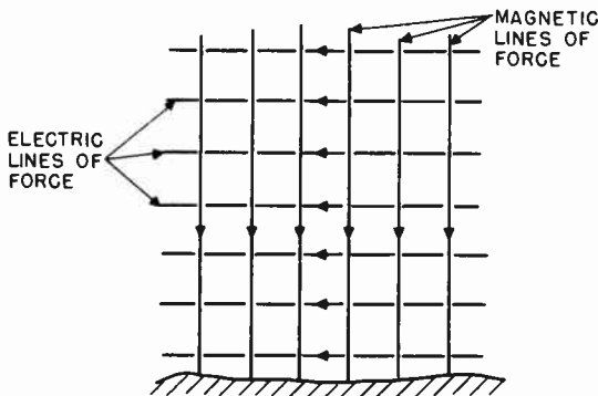
Figure 1. Representation of the magnetic and electric fields of horizontally polarized wave.
