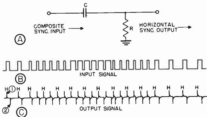
Figure 88. A, differentiating circuit. B, input and output waveforms of circuit in A.
