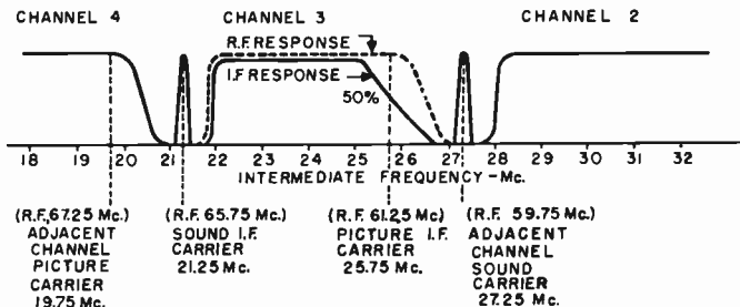
Figure 35. The relationship between the response of a television receiver, the television signal, and signals in adjacent channels.
