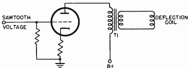
Figure 116. Sweep amplifier for magnetic deflection.
