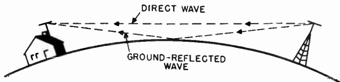
Figure 11. Cancellation of direct wave by ground-reflected wave.
