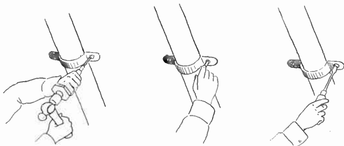
Figure 32. Drilling and mounting to masonry.
