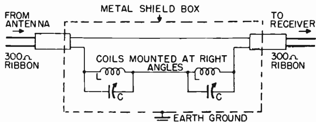
Figure 40. Circuit for wave trap.
