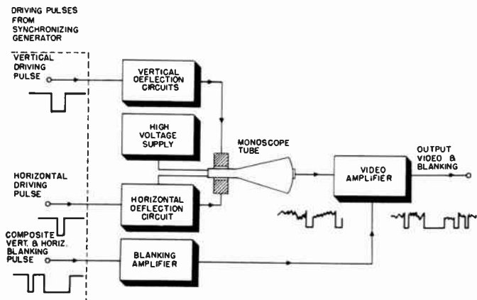
Figure 100. Block diagram of monoscope camera circuit.
