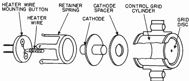
Figure 6. The cathode-grid assembly.
