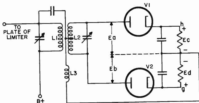
Figure 173. Foster-Seeley discriminator.
