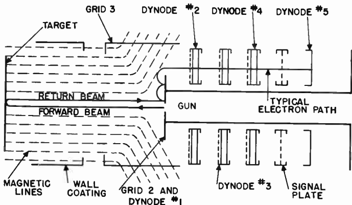
Figure 10. Electron Multiplier Section of the image orthicon.
