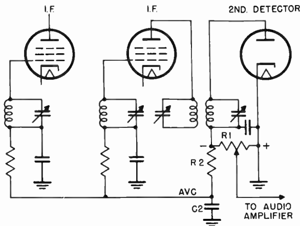
Figure 74. Simplified schematic of a.v.c. circuit of a-m receiver.
