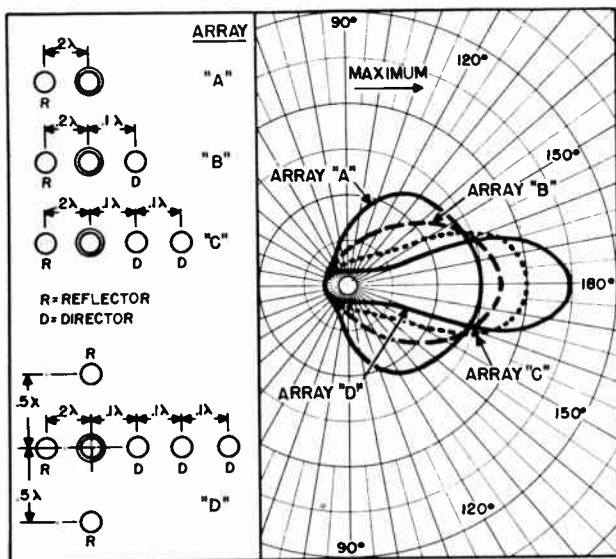
Figure 56. Field patterns of four parasitic arrays.
