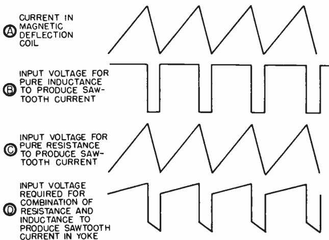
Figure 114. Waveforms of current and voltage in magnetic deflection systems.
