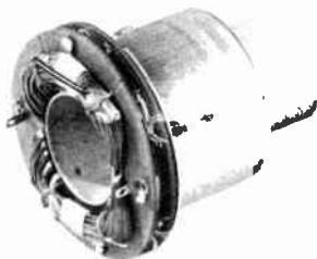
Figure 35. A commercial yoke.
