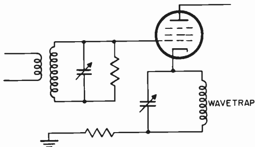
Figure 48. Simplified circuit of i-f amplifier with cathode wave-trap.
