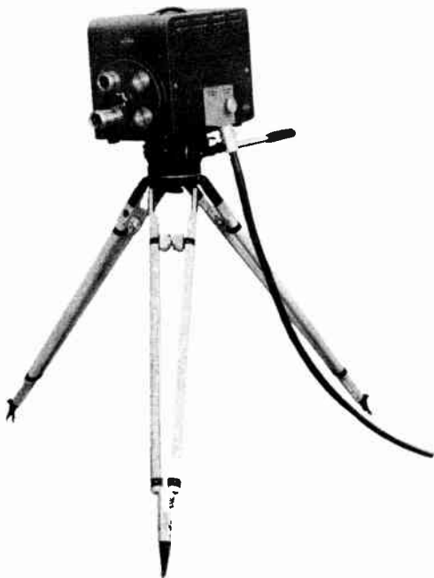
Figure 72. Pickup head mounted on tripod for remote pickup use. (courtesy Raytheon)
