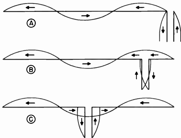
Figure 72. Long-wire antenna, showing current distribution and feed points.
