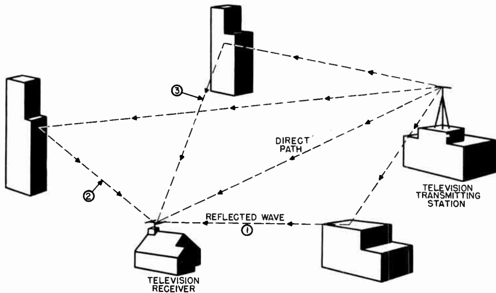
Figure 7. Several reflected waves arriving at antenna along with direct wave.
