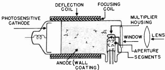
Figure 3. Construction of the image dissector.
