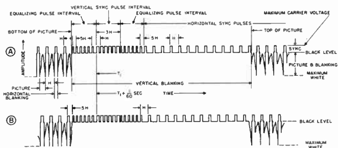
Figure 19. Standard F.C.C. television signal.
