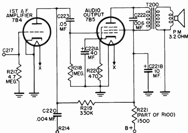
Figure 29. Audio amplifier.
