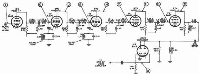
Figure 70. Simplified schematic of wide-band video i-f amplifier, showing points at which instruments are connected when alignment is performed.
