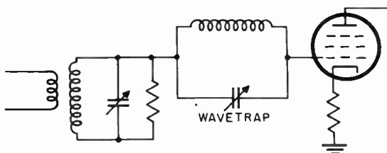
Figure 47. Simplified circuit of i-f amplifier with grid wave-trap.
