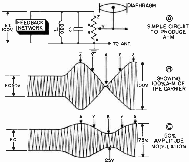
Figure 157. Simple method of amplitude modulation.
