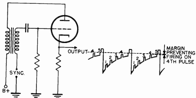
Figure 23. Blocking oscillator frequency divider.
