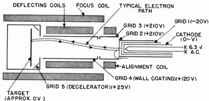
Figure 9. Scanning section of the image orthicon.
