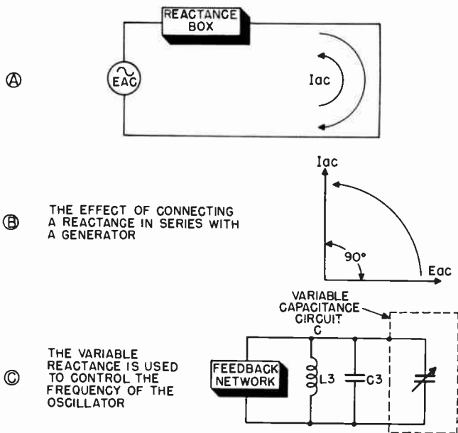
Figure 159. Operation of reactance modulator.
