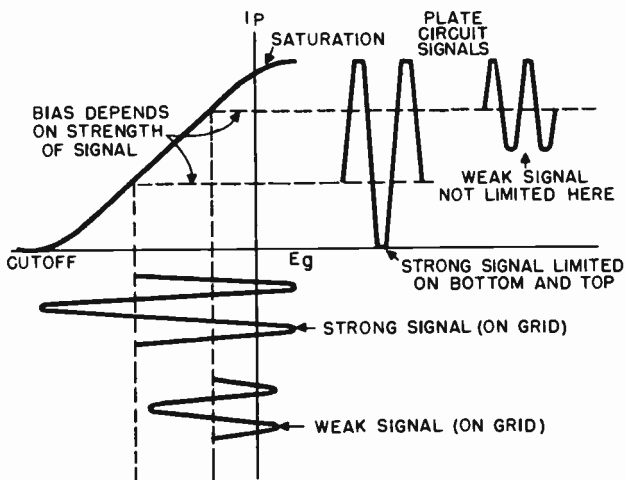
Figure 166. Operation of limiter circuit.
