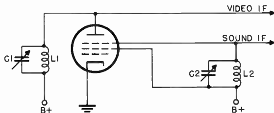
Figure 20. Plate and suppressor-screen tuned circuits for separating video and audio signals.
