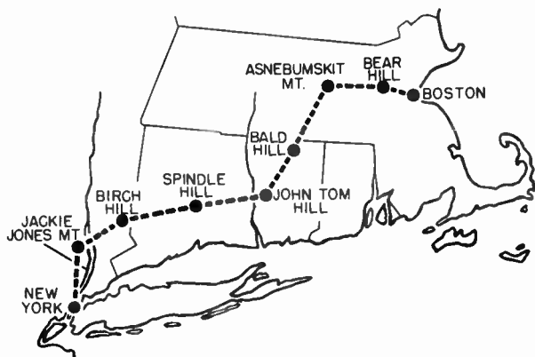
Figure 81. Microwave relay link between New York and Boston.
