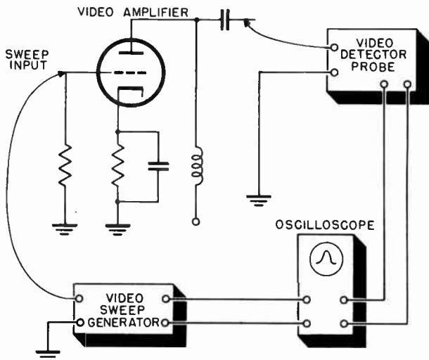
Figure 65. Connections used to adjust video amplifier using sweep generator and oscillograph.
