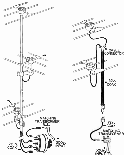
Figure 44. Typical application of coaxial switch.
