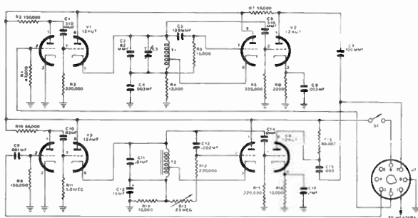
Figure 18. Schematic circuit of Crosshatch Generator
