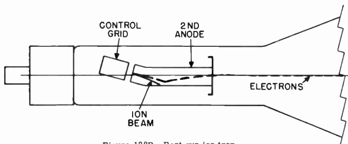
Figure 128B. Bent gun ion trap.
