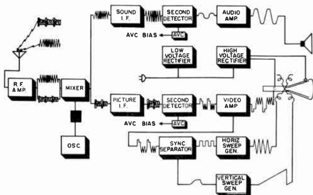
Figure 3. Block diagram of a television receiver with waveforms at input and output of stages.
