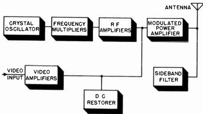
Figure 42. Block diagram of high level modulated transmitter.
