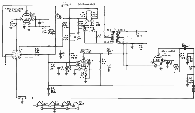
Figure 49B. Sync stabilizer schematic.
