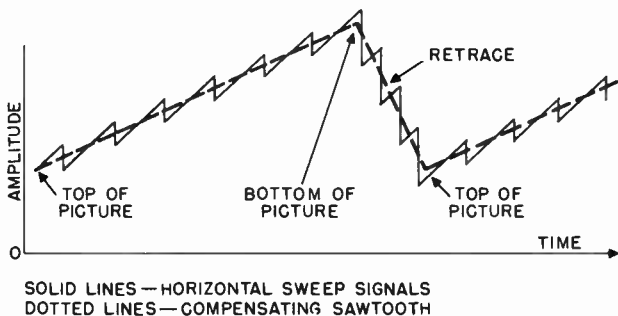
Figure 48. Compensating signal for overcoming keystoneing.
