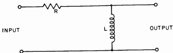
Figure 177. Pre-emphasis filter.
