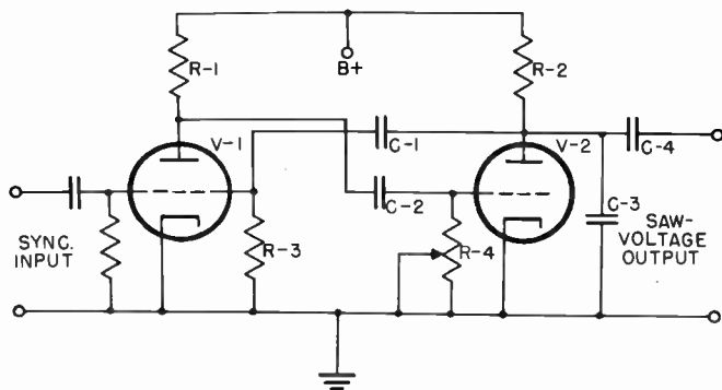
Figure 96. Multivibration circuit.
