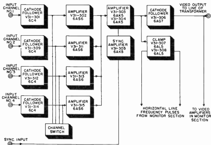
Figure 77. Block diagram of mixer amplifier.
