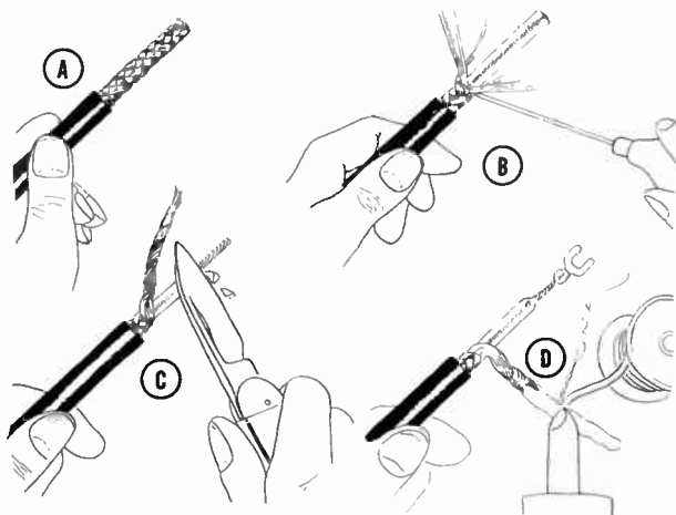
Figure 11. Step-by-step method of preparing coaxial cable by unbraiding and tinning braid. A, cut back rubber insulation. B, score braid. C, twist scored braid and cut back insulation to expose center conductor. D, tin braid and add lug.
