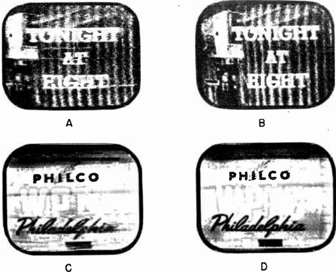
Figure 102. Improvement brought about by incorporating fly-wheel sync in receiver.
