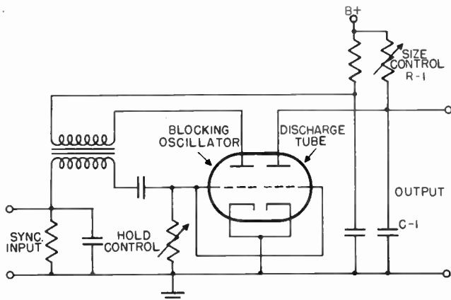
Figure 110. Blocking oscillator discharge circuit using dual triode.
