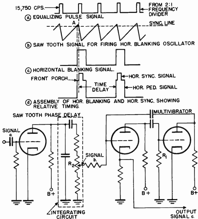
Figure 27. Generation of horizontal blanking pulses.
