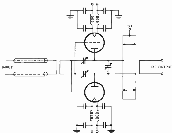
Figure 50. Wideband r-f amplifier circuit.
