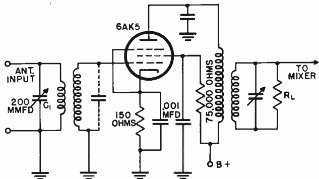
Figure 5. Pentode r-f amplifier.
