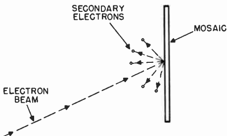
Figure 44. Secondary electrons emitted by a globule on the mosaic.
