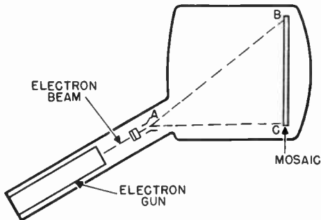
Figure 46. Keystoneing occurs in the iconoscope because the electron beam travels unequal paths from the gun to the mosaic.
