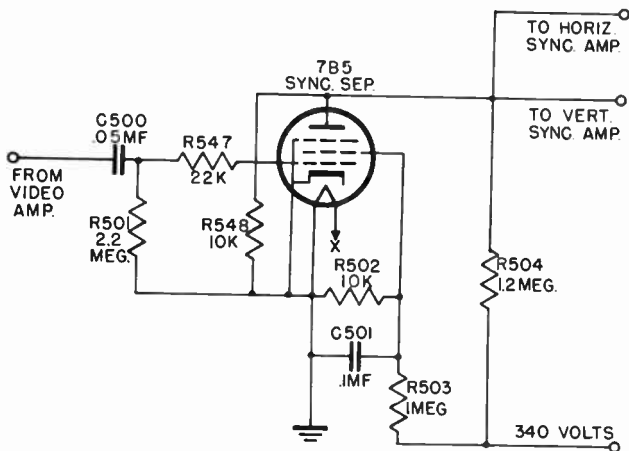
Figure 24. Sync separator.
