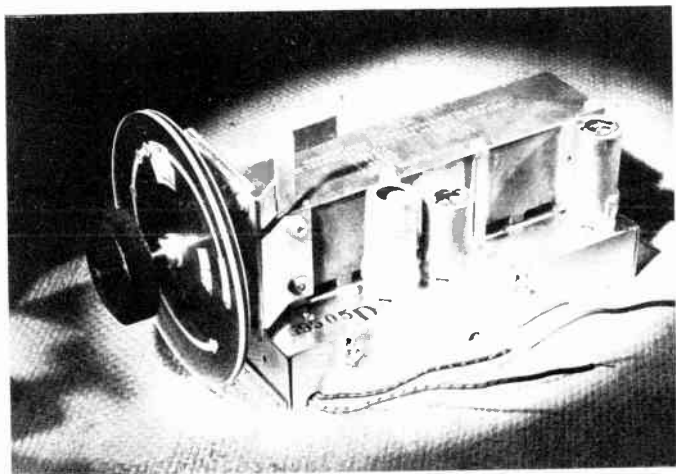
Figure 13. Complete Input tuner assembly for continuous 44-216 Mc coverage, showing manual drive dial. (courtesy DuMont)
