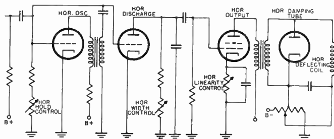
Figure 119. Simplified schematic of horizontal sweep circuit with damping tube.
