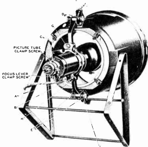
Figure 139. The optical barrel of the Philco projection system.
