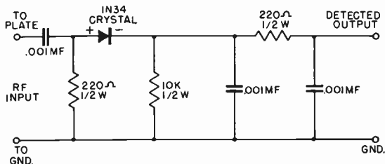
Figure 16. Probe detector.
