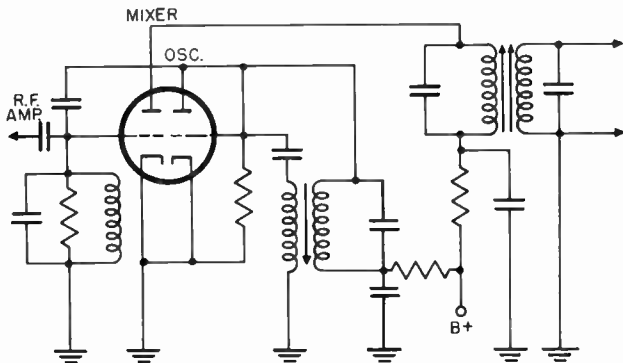
Figure 17. Dual triode mixer-oscillator using grid injection.
