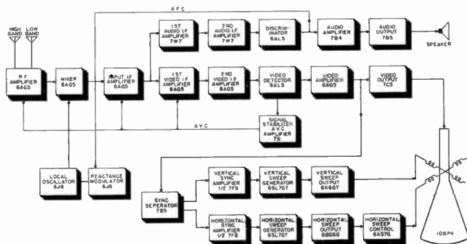
Figure 21. Block diagram of Philco Model 48-1000.
