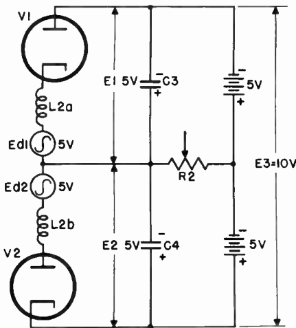
Figure 176. Equivalent circuit of ratio detector.
