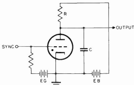
Figure 5. Gas triode sawtooth generator.
