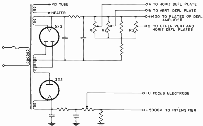
Figure 122. Power supply and positioning controls for electrostatic cathode-ray tube.
