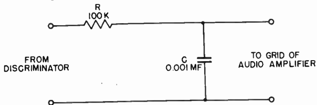
Figure 179. De-emphasis filter.
