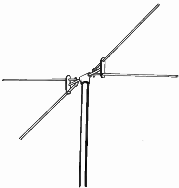
Figure 42. Double-V antenna.
