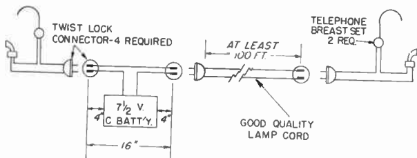
Figure 7. Battery-operated phone system.
