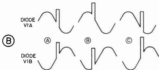
Figure 100. Automatic frequency control circuit which eliminates need for manual hold control.
