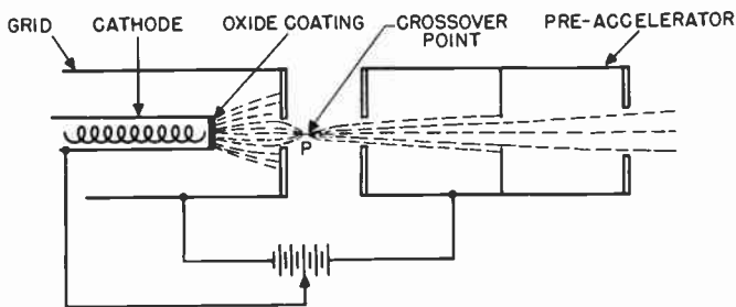
Figure 14. The "crossover" point of the electron beam is between the grid and the pre-accelerator electrode.
