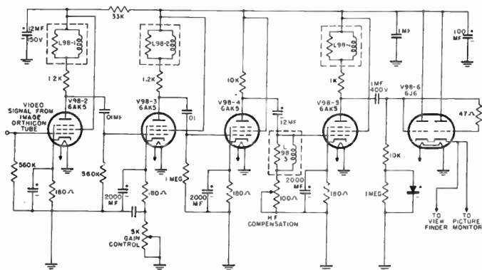
Figure 15. Circuit of video amplifier used in image orthicon camera.
