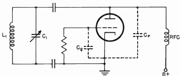
Figure 13. Ultraudion oscillator.
