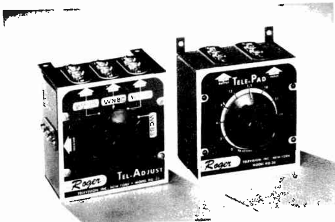
Figure 37. The Tel-Adjust and the Tele-Pad, used to reduce too strong a signal. (courtesy Roger Television)
