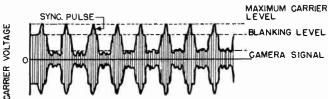
Figure 57. Modulated television carrier.
