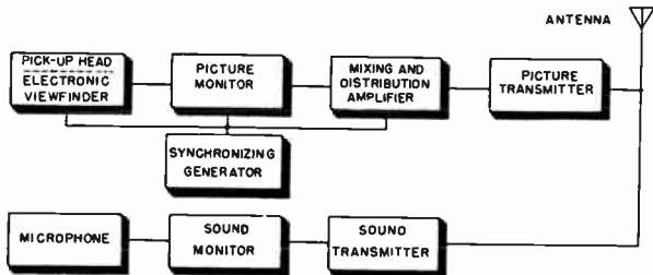
Figure 1. Block diagram of simple television transmitter.
