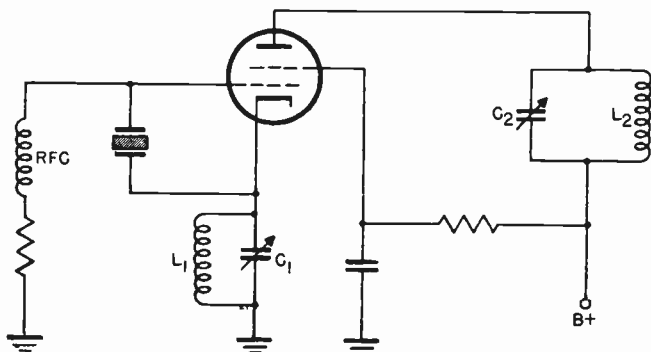
Figure 44. Tri-tet oscillator.
