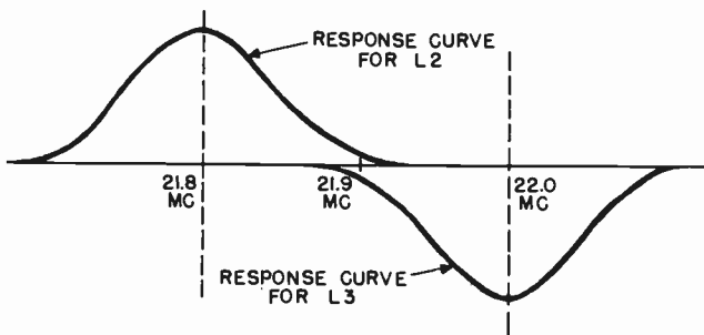
Figure 171. Response curve of tuned circuits of discriminator.
