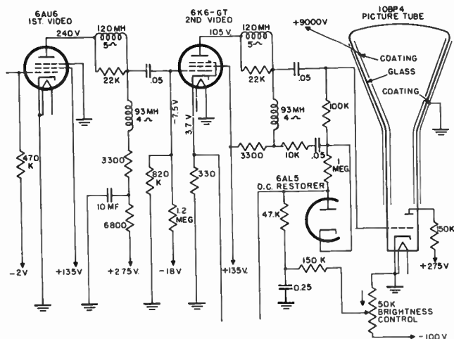
Figure 65. Two stage video amplifier using shunt and series peaking.
