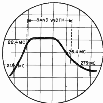
Figure 46. Videoi-f response curve using tuned circuits only.
