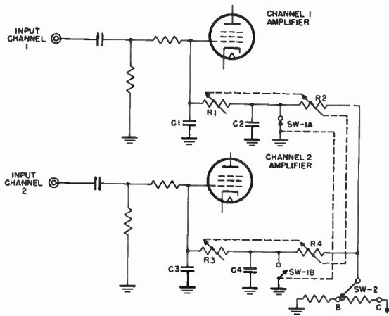
Figure 79. Simplified schematic of input switching circuits.
