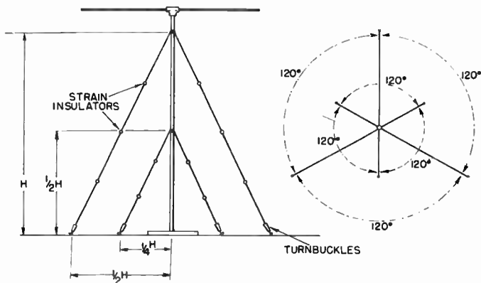
Figure 27. Guy-wire spacing.
