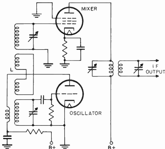
Figure 15. Inductively-coupled mixer-oscillator.
