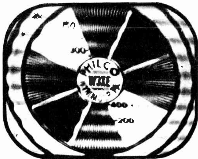
Figure 34. Test pattern showing effects of sound in the picture channel.
