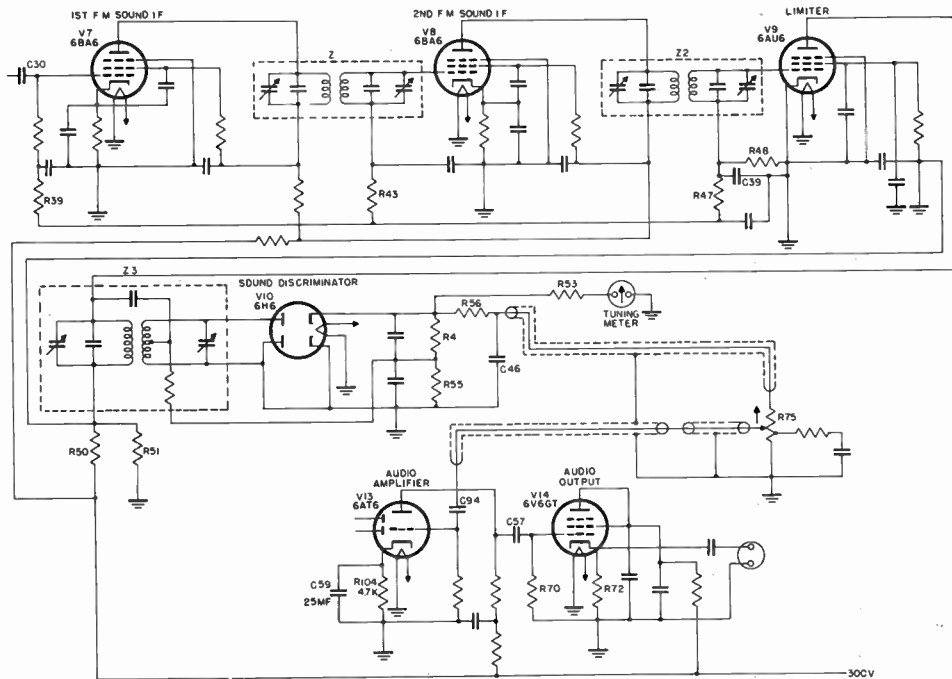
Figure 37. Sound channel.
