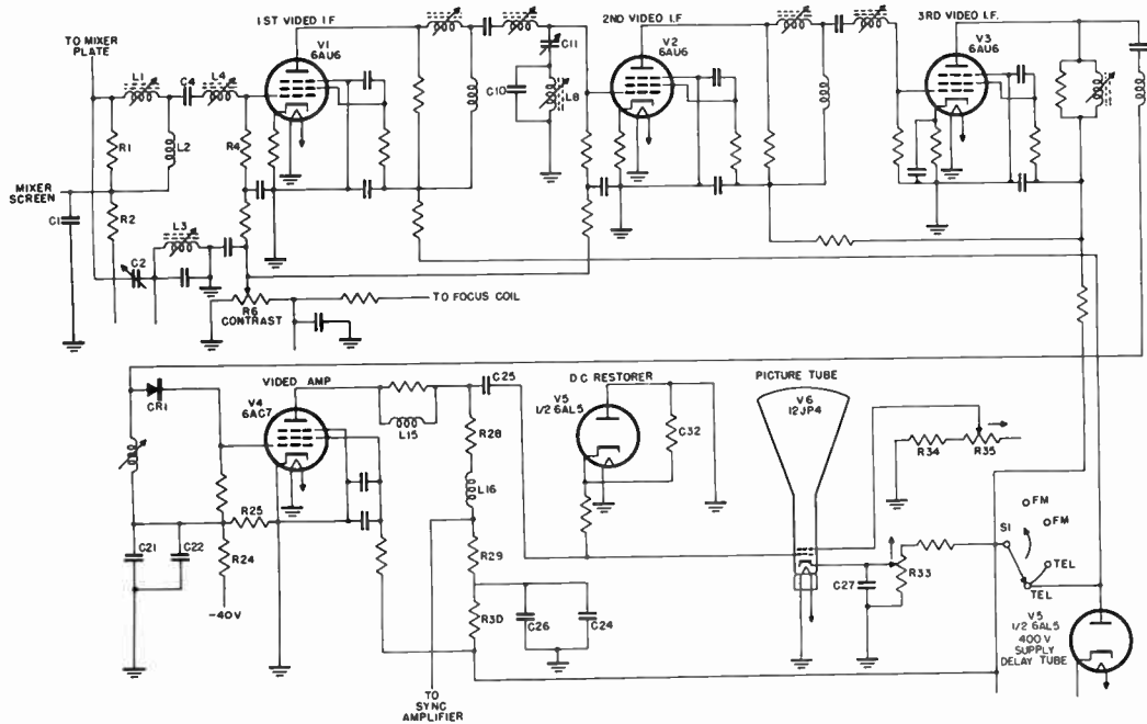
Figure 33. Video circuits.
