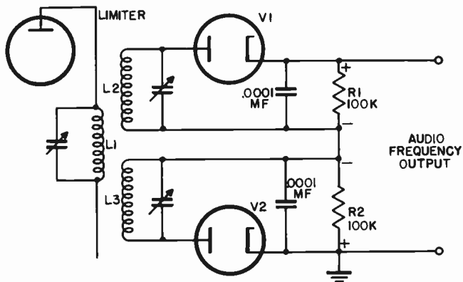
Figure 170. Simple discriminator circuit.
