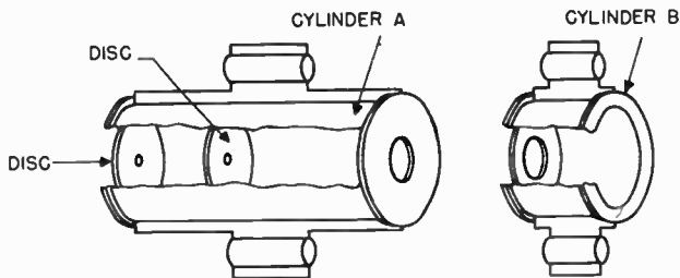
Figure 7. The pre-accelerator electrode assembly.
