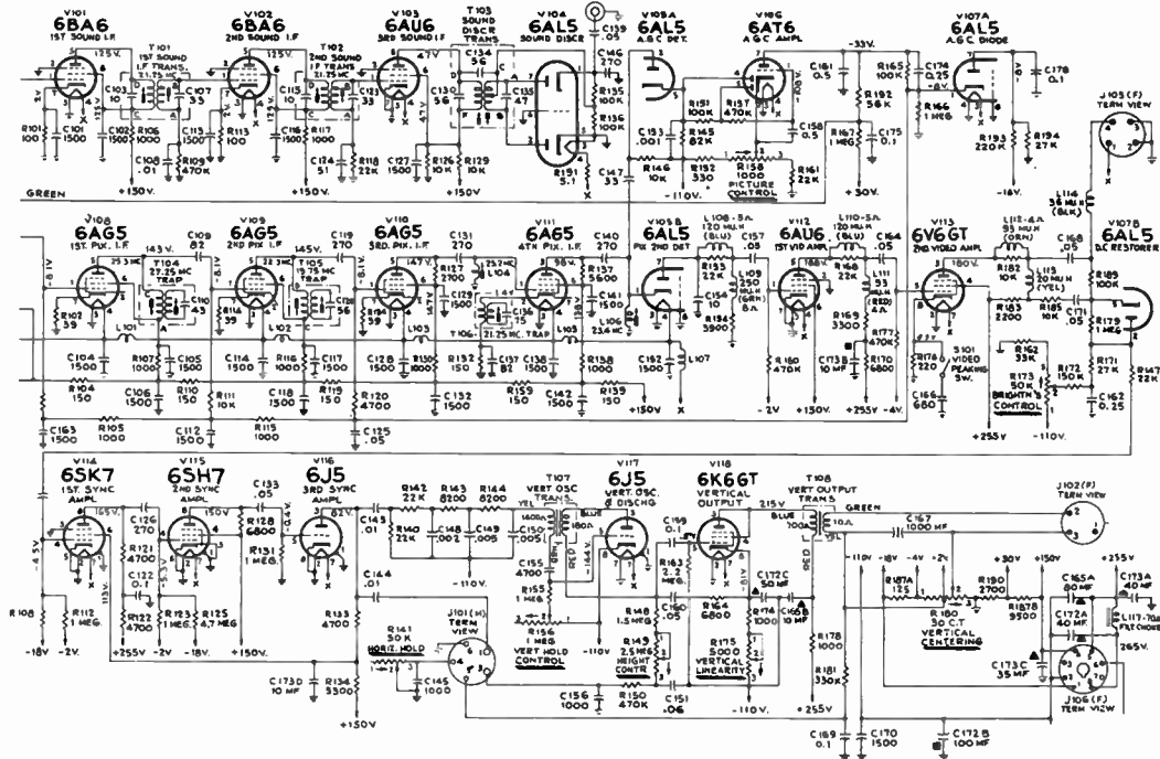
Figure 53. Video, sound, and vertical sweep circuits.
