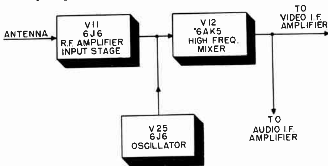
Figure 11. Block diagram of DuMont Inputuner.
