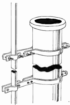
Figure 20. Bracket for mounting on vent pipe.
