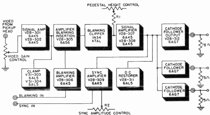
Figure 37. Block diagram of mixing and distribution amplifier.
