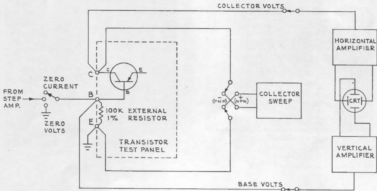
Fig. 14. System for measuring low values of I_{cbo} or I_{cao} .
