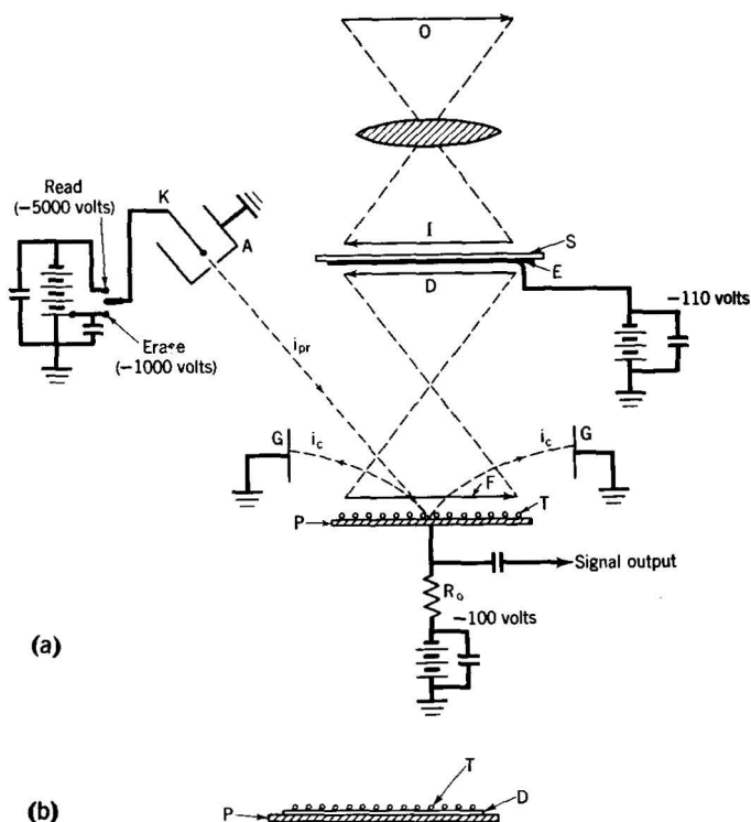
Fig. 34. Television-camera storage tube (Knoll and Randmer).
