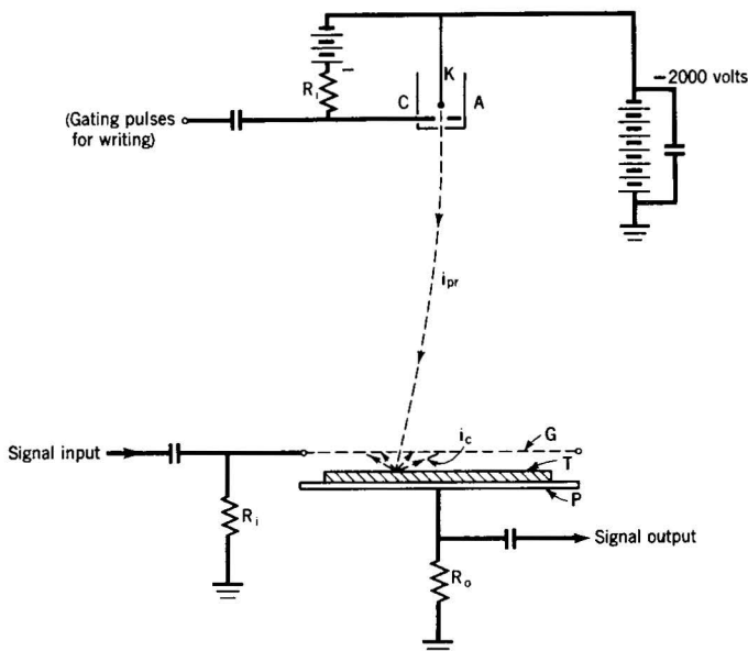
Fig. 25. Computer storage tube (Forrester).
