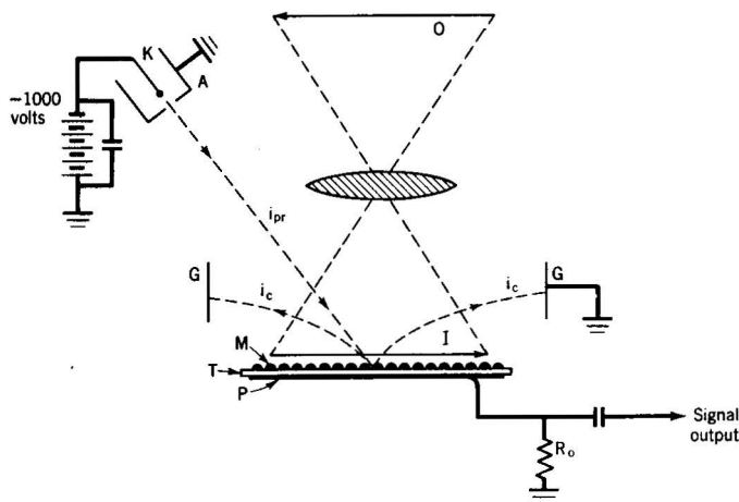
Fig. 28. Television-camera storage tube (Iconoscope).
