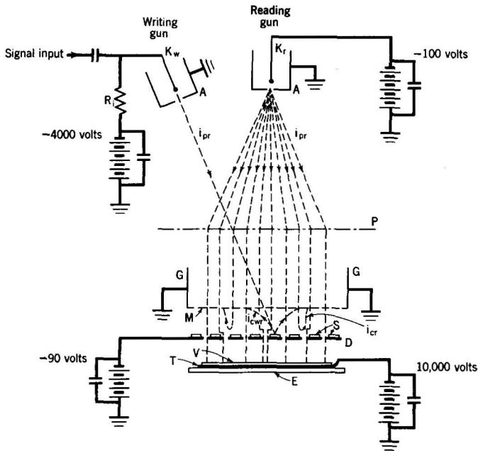
Fig. 22. Viewing storage tube with electron lens raster (Knoll).
