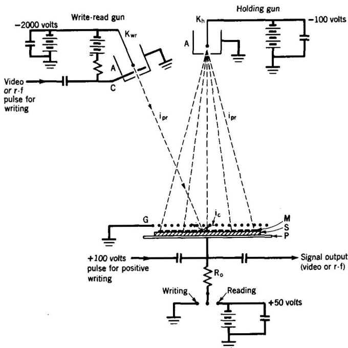
Fig. 27. Computer storage tube (Dodd, Klemperer, and Youtz).
