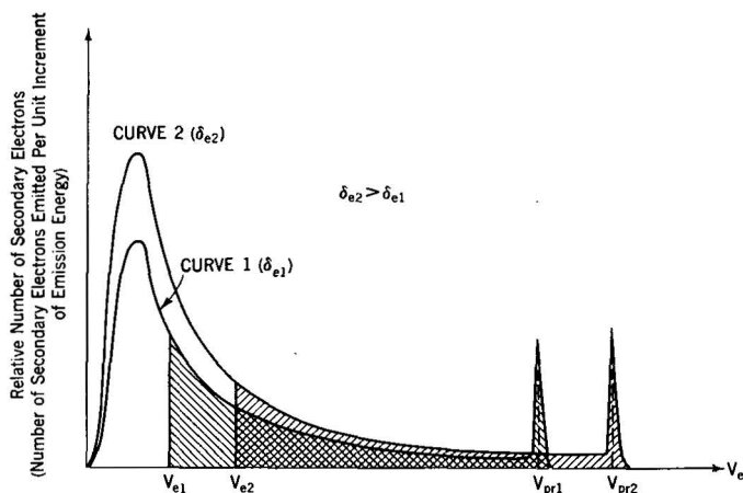
Fig. 5. Velocity distribution curves of secondary electrons for a given material showing minimum energy of secondary electrons which can reach the collector for different primary energies. V_e , emission energy of secondary electrons in volts.
