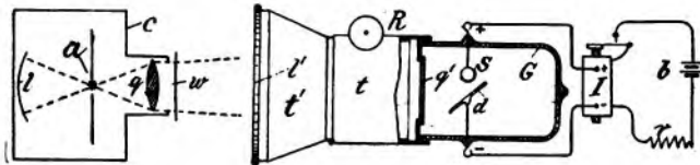
FIG. 99. ZICKLER TRANSMITTER.
