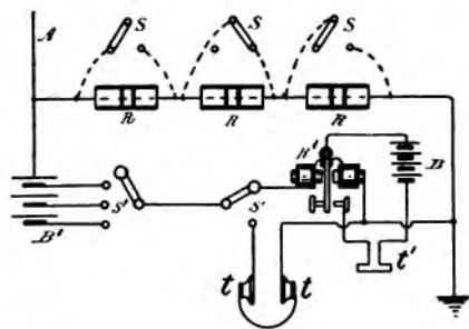
FIG. 82. CALLING RELAY.
