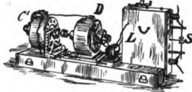
FIG. 80. MOTOR-GENERATOR.
