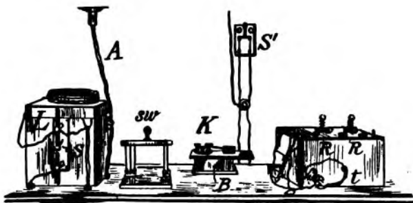
FIG. 86. SHIPBOARD OUTFIT.
