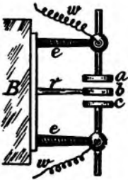
FIG. 79. DISK SPARK-GAP.
