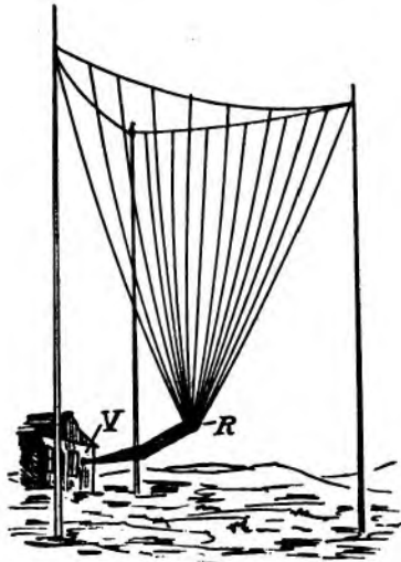
FIG. 71. BRANLY-POPP AERIAL WIRES.
