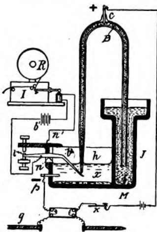
FIG. 106. ARMORL WIRELESS SYSTEM.
