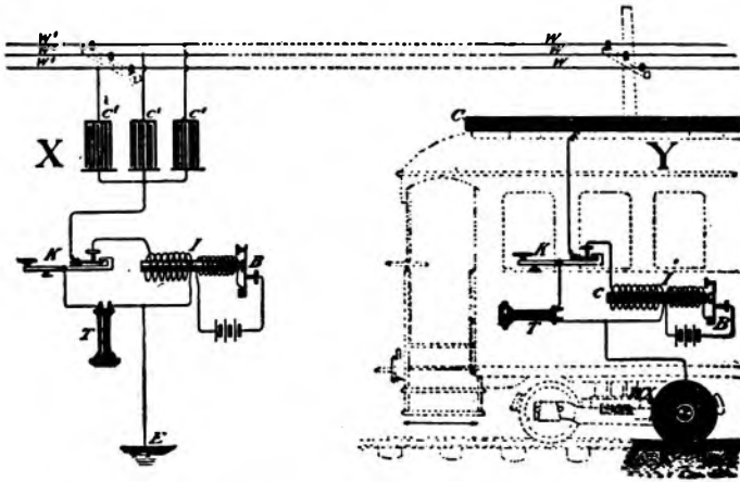
FIG. 7. EDISON INDUCTION TELEGRAPHY.
