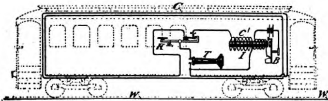
FIG. 6. PHELPS INDUCTION TELEGRAPH
