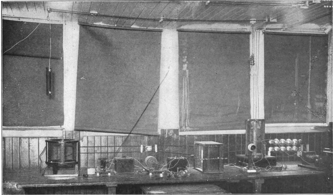
THE WIRELESS-TELEPHONE APPARATUS OF THE BANCROFT FOOTE BOYS' CLUB, Y. M. C. A., NEW HAVEN, CONNECTICUT
