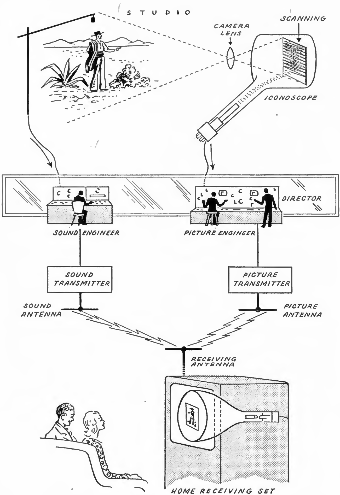
BLACK AND WHITE TELEVISION SYSTEM FROM STUDIO TO RECEIVER
