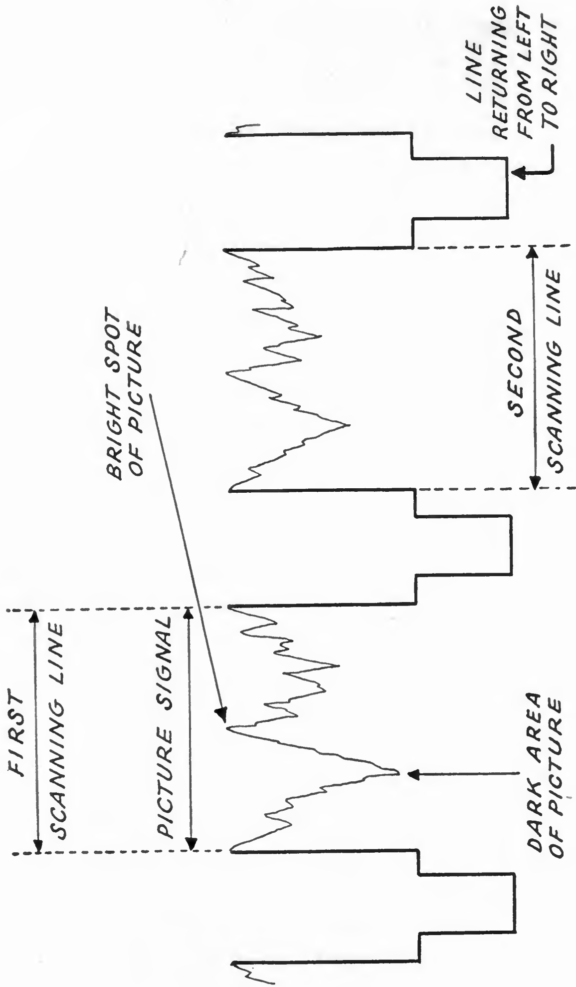
ELECTRONIC SIGNAL PRODUCED BY TELEVISION CAMERA
