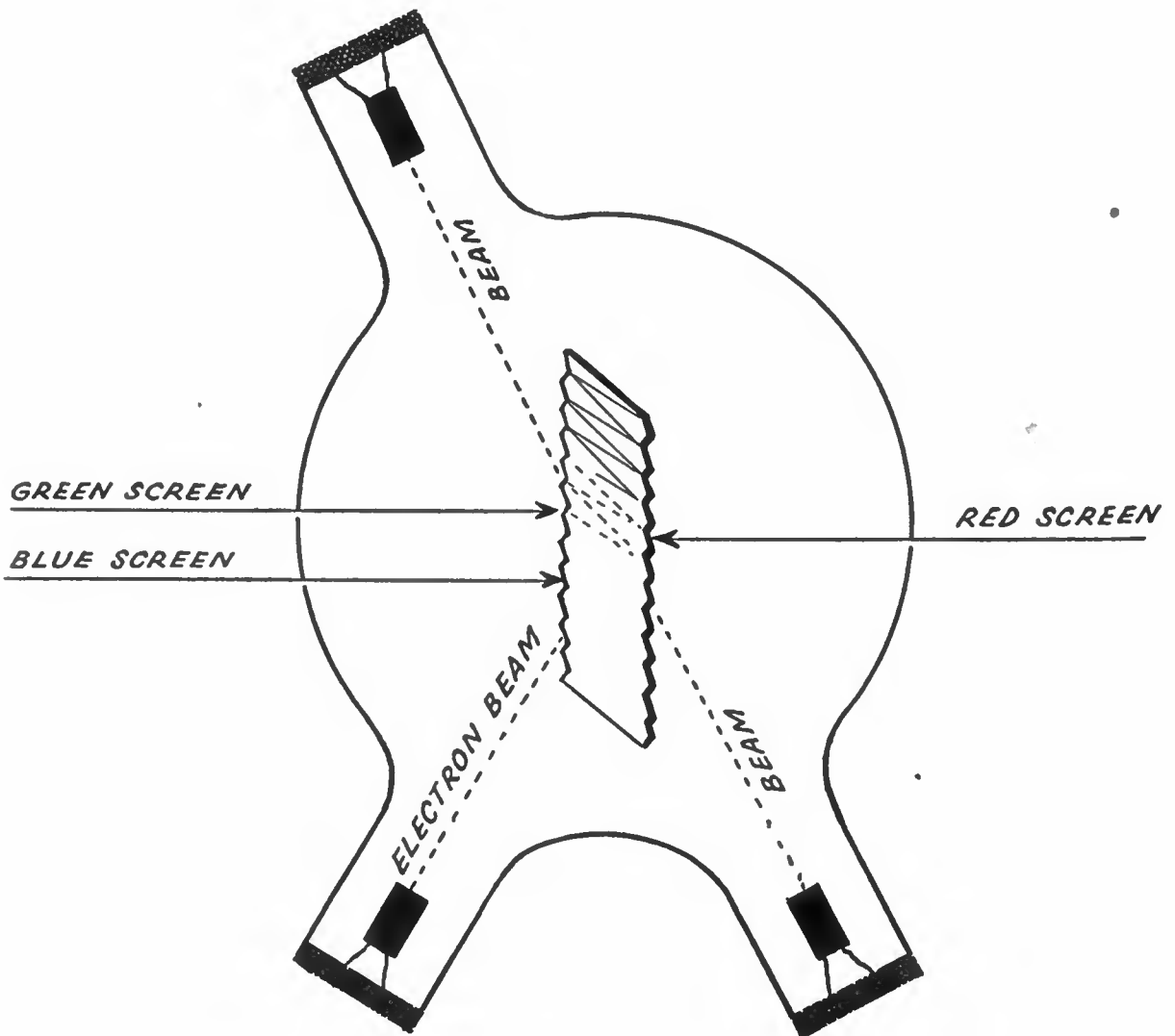
COLOR CAMERA TUBE FOR THREE-COLOR BAIRD SYSTEM
