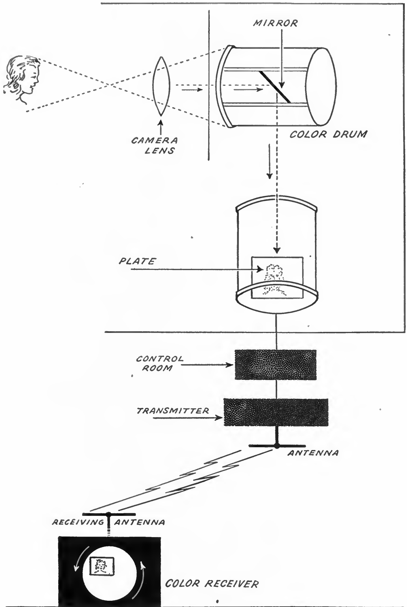
TELEVISION COLOR TRANSMISSION FROM CAMERA TO RECEIVER
