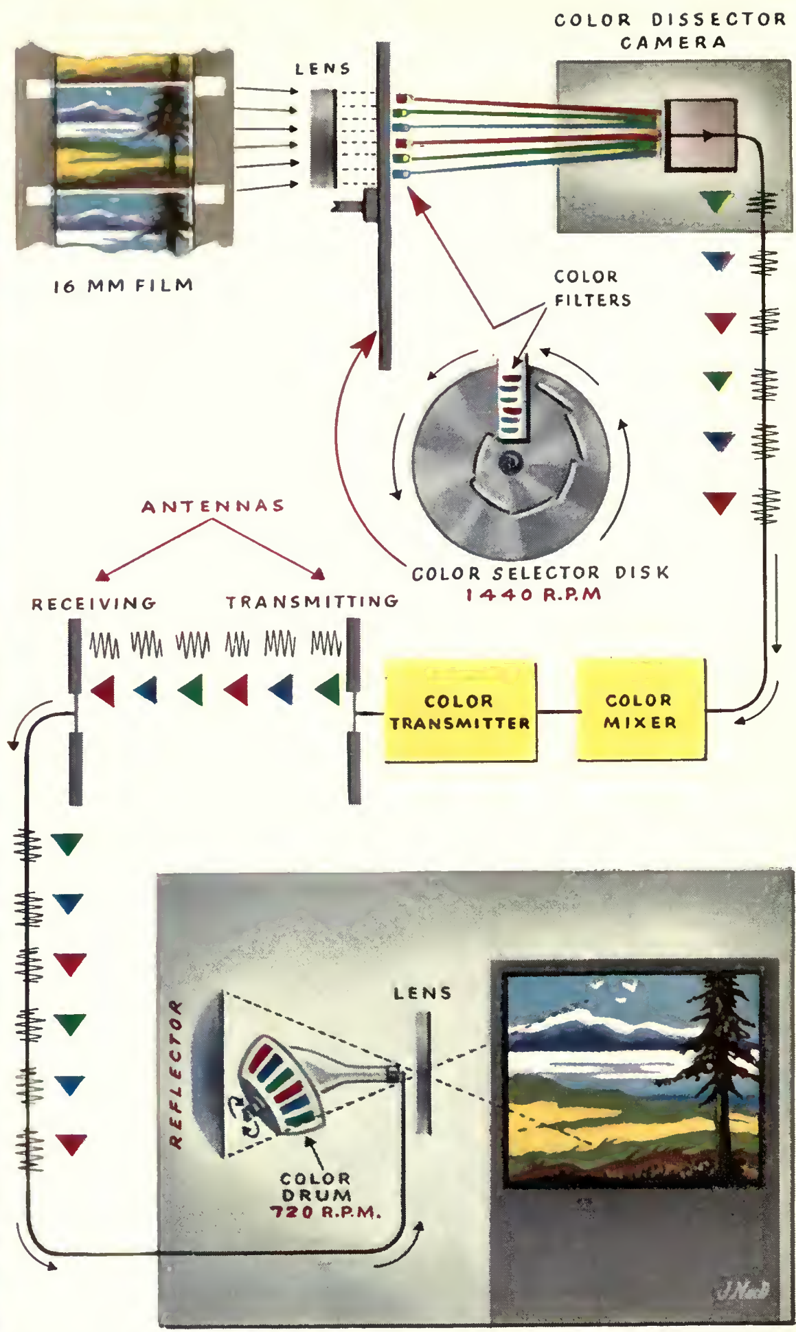
C.B.S. COLOR SYSTEM FOR FILM
