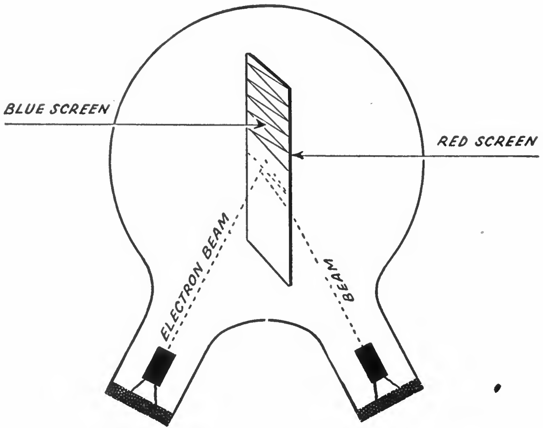
COLOR CAMERA TUBE FOR TWO-COLOR BAIRD SYSTEM
