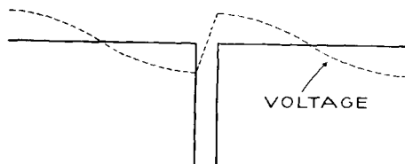
Figure 5 The "Voltage-Fed" Zepp. (Compare Figure 6).
