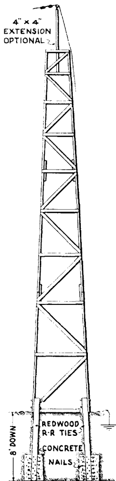
Figure 3 The foundation used for a guyless tower (four redwood posts or railroad ties sticking out of the ground a ways) to which the base of the tower is anchored.
