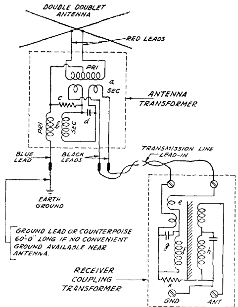
Figure 17 "Double Doublet" system giving good broadcast-band response
