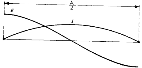
Figure 2 Showing Voltage (E) and Current (I) Distribution on a Half-wave Antenna
