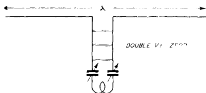
Figure 8 The "Double Zepp." See Figure 7.
