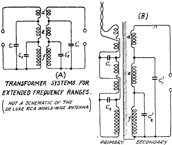
Figure 16 Two coupling systems giving extended frequency ranges
