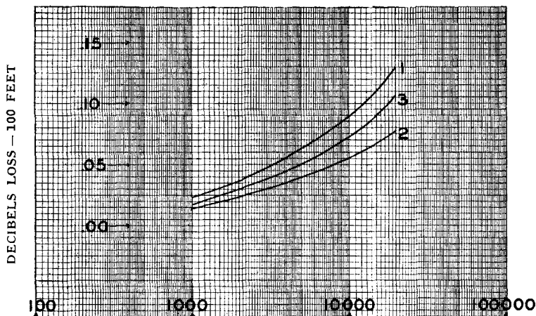
FREQUENCY — KILOCYCLES PER SECOND LOSS VERSUS FREQUENCY (COMPUTED LOSS PLUS 50%)
