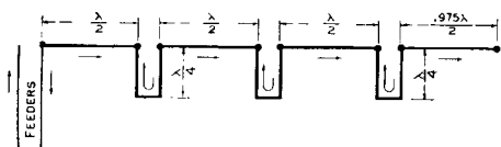
Figure 21 Four Half Waves in Phase to Increase Broad- side Directivity; Zepp. Fed.
