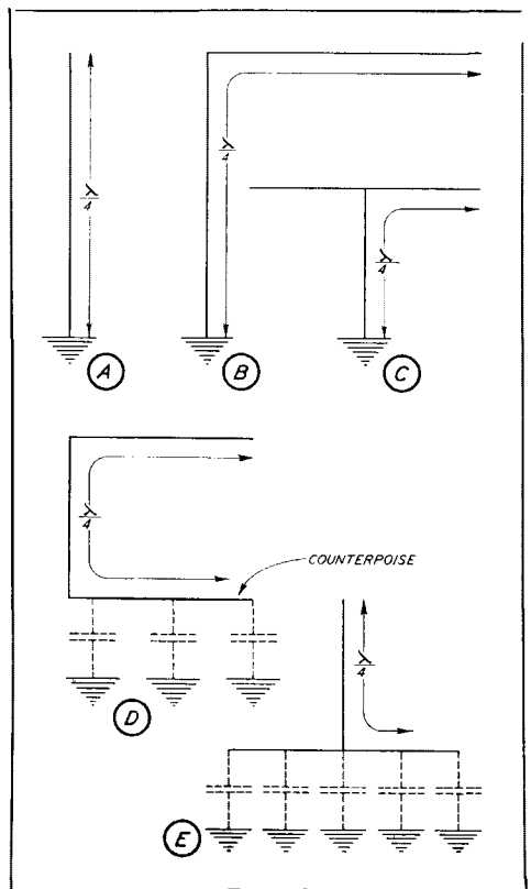
Figure 3 Variations of the Marconi Type Antenna (Grounded and Capacity Grounded)
