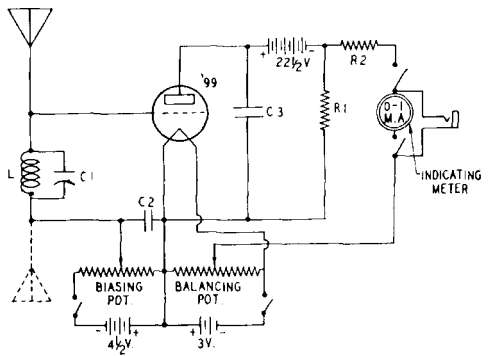
Figure 8 A Simple Field Strength Meter L—18 d.c.c. on 1\frac{1}{4} " diam. form to hit band C 1 —100 μfd. midget variable condenser C 2 and C 3 —0.001 μfd. Biasing potentiometer—2000 ohms Balancing potentiometer—200 ohms R 1 —5000 ohms R 2 —1000 ohms
