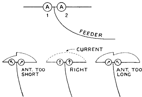
Figure 33 Checking the Single-Wire-Fed Antenna.
