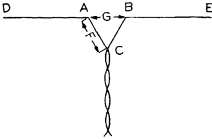
Figure 20 Reference Schematic of the Doublet of Figure 18.
