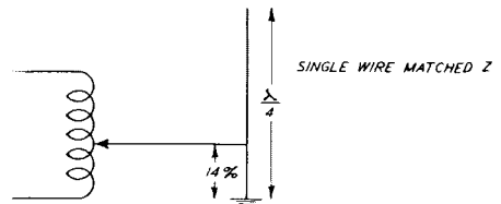
Figure 34 Marconi with Single Wire Feed.
