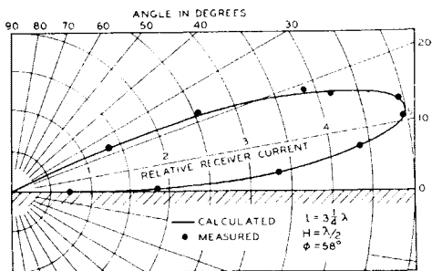
Figure 13 Vertical directivity of the \frac{3}{4} wavelength rhombic antenna described in the text. The receiver current ratio of 5/1 at the tip of the lobe represents a power gain of 25 times, or 14 db.
