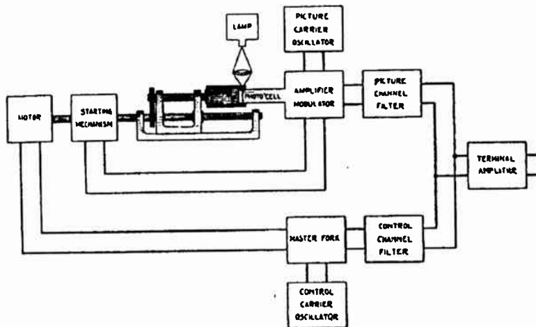
FIG. 21.—Schematic Diagram of Sending End of Apparatus.
