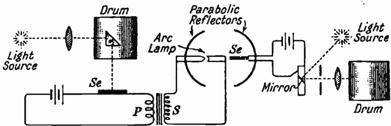
FIG. 16.—Bernouchi's Method.
