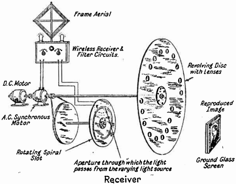
FIG. 30.—Mr. Baird's original Receiving Apparatus.
