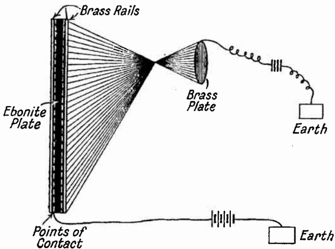
FIG. 14.—Senlecq's Apparatus.
