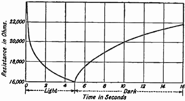
FIG. 35.—General Curve showing Inertia or Lag of a Selenium Cell.
