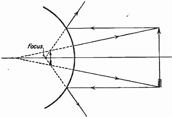
FIG. 75.—Image formed by Convex Mirror.
