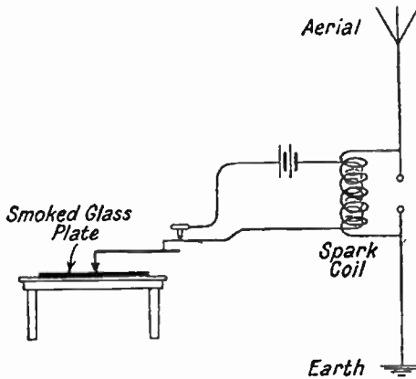
FIG. 24.—Knudsen's Transmitter Circuit.
