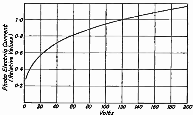
FIG. 45.—Curve of Current-voltage Variation (General Electric Co.'s Vacuum Cell).
