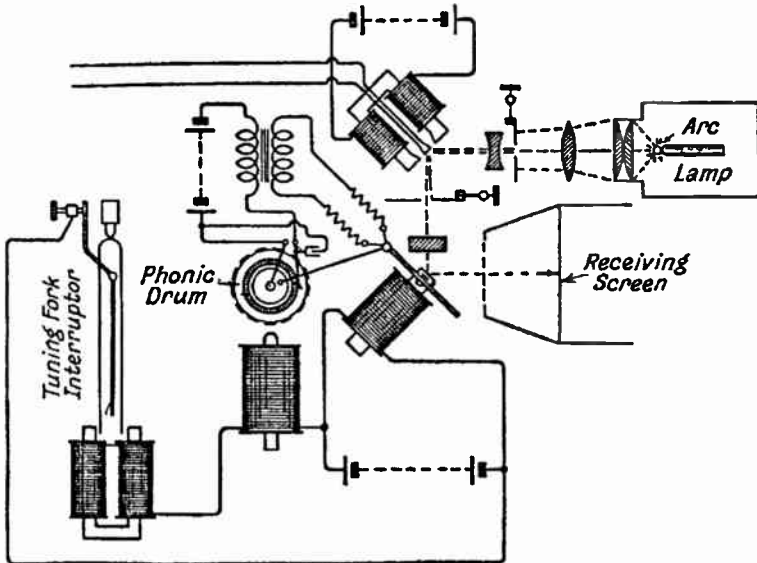
FIG. 55.—The "Telehor" Receiving Circuit.
