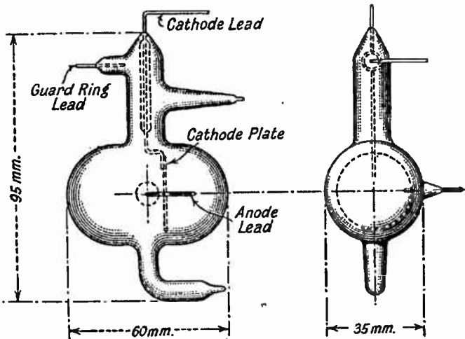
FIG. 43.—The General Electric Co.'s new type of Photo-electric Cell.
