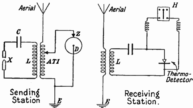
FIG. 17.—Diagram of Korn's Circuit.
