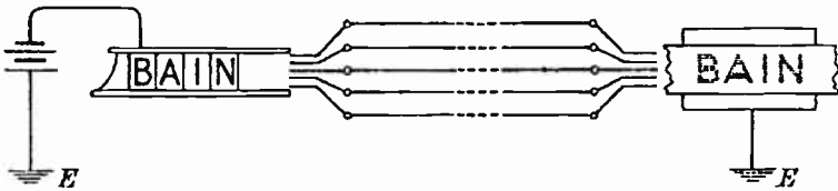
FIG. 9.—Bain's Chemical Recorder.
