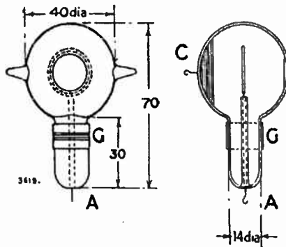
FIG. 41.—The Cambridge Inst. Co.'s Photo-electric Cell. (Internal Construction.)
