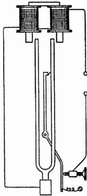
FIG. 56.—The Tuning-fork Interrupter.
