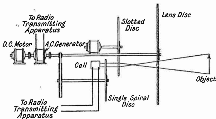
FIG. 79.—Diagrammatic Sketch of Transmitting Arrangements.
