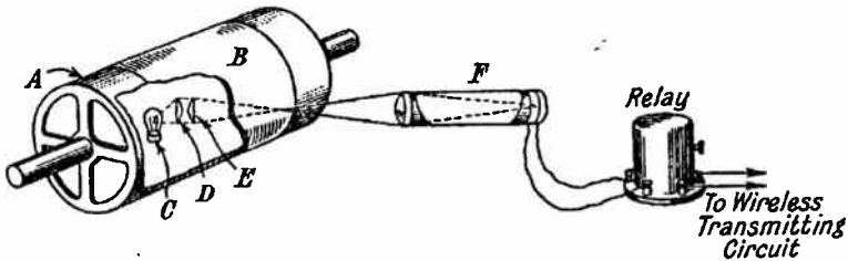
FIG. 25.—Diagrammatic Sketch of Ranger's Transmitting Cylinder.
