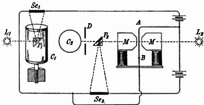
FIG. 18.—Arrangement of Korn's Apparatus.
