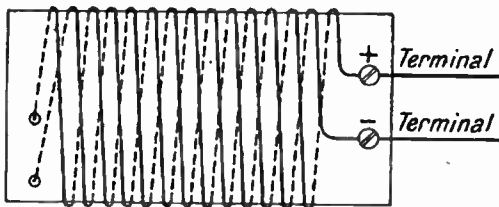
FIG. 32.—Early form of Selenium Cell.
