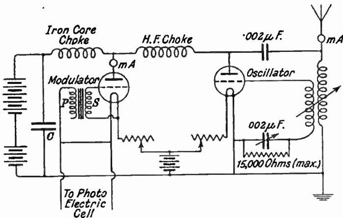
FIG. 93.—Transmitting Radio-circuit.
