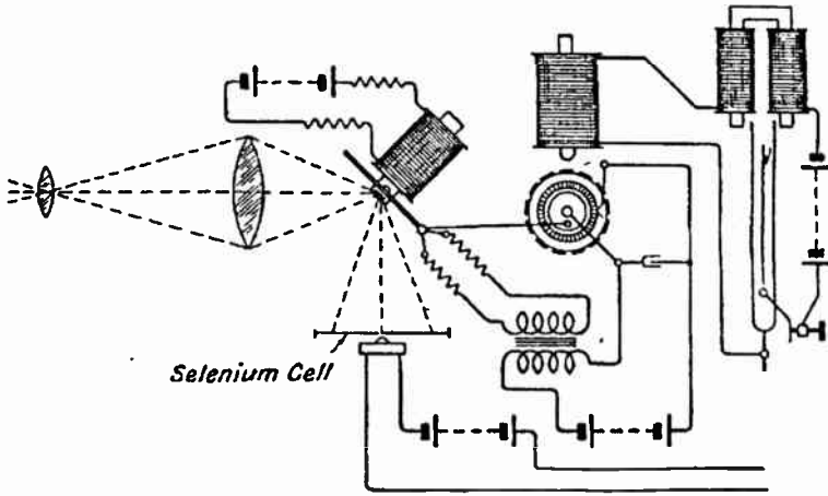
FIG. 54.—The "Telehor" Transmitter Circuit.
