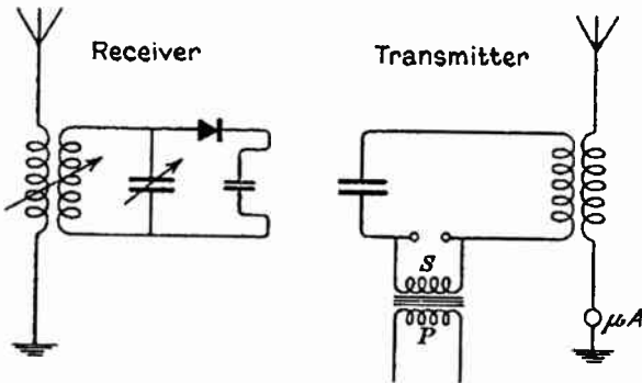
FIG. 90.—Syntonic Wireless Circuit with Carborundum Detector.
