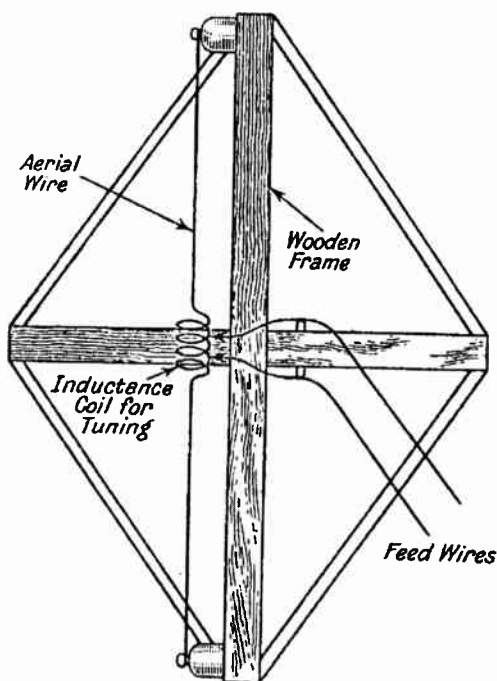
FIG. 92.—Short Wave Transmitting Aerial.
