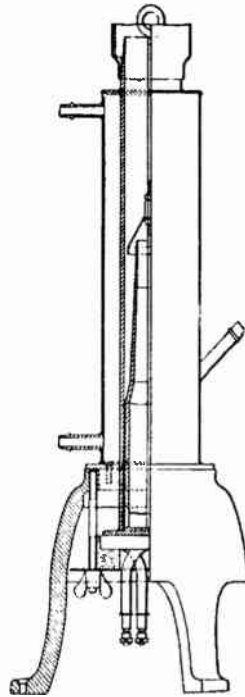
FIG. 39.—Diagram showing Internal Construction of the Langmuir Pump.
