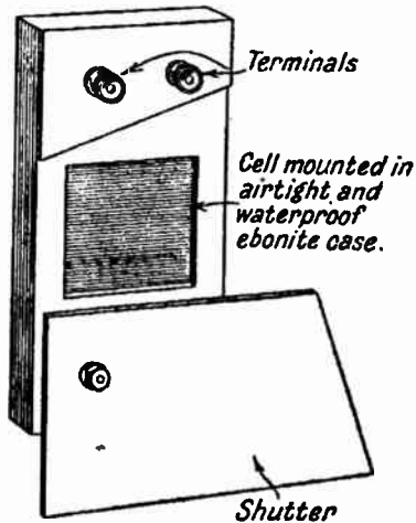
FIG. 34.—Modern form of Selenium Cell (mounted).
