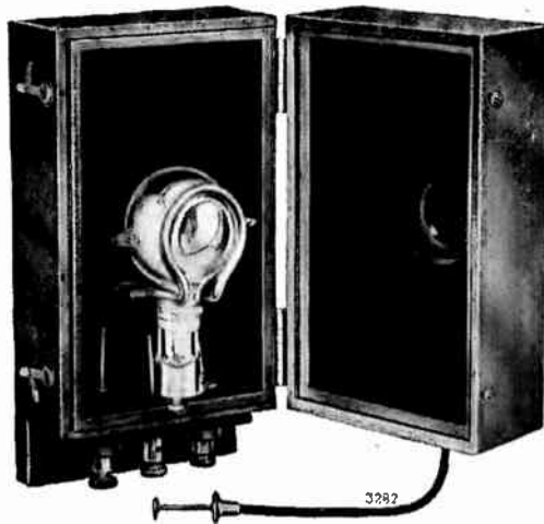
FIG. 40.—The Cambridge Inst. Co.'s Photo-electric Cell.
