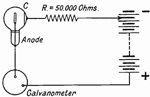
FIG. 48.—Connections for measuring Photoelectric Current.
