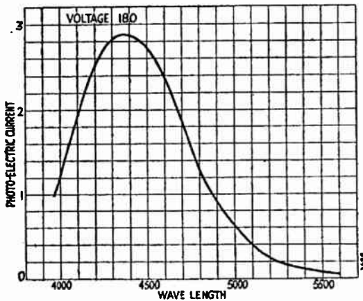
FIG. 47.—Current Wave-length Curve for an Average Cell.
