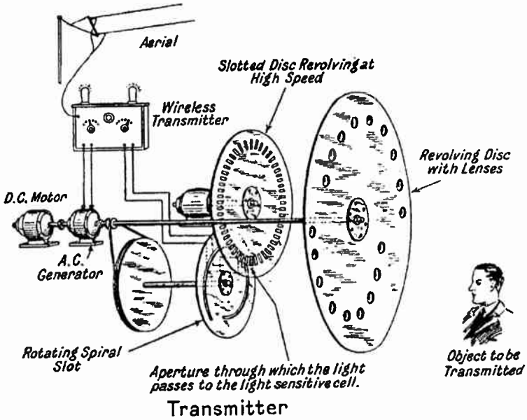
FIG. 29.—Mr. Baird's original Transmitting Apparatus.
