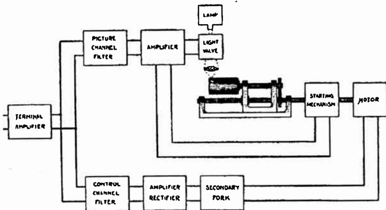
FIG. 22.—Schematic Diagram of Receiving End of Apparatus.
