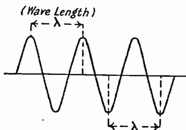
FIG. 69.—Wave-length.
