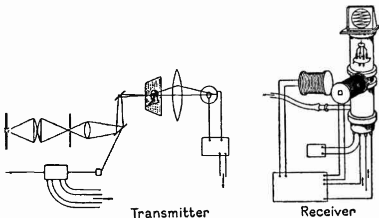
FIG. 52.—Apparatus of MM. Belin and Holweck.
