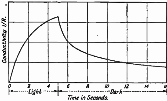
FIG. 36.—General Curve for behaviour of a Selenium Cell.
