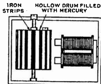
FIG. 57.—La Cour's Phonic Drum
