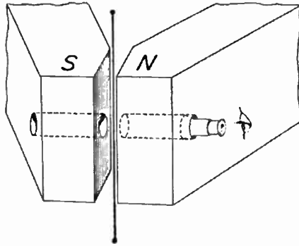
FIG. 19.—Diagrammatic Illustration of the Einthoven String Galvanometer.
