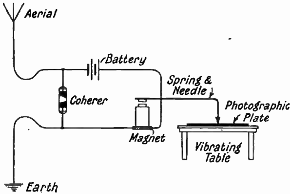
FIG. 23.—Knudsen's original Receiving Circuit for Radio Photography.
