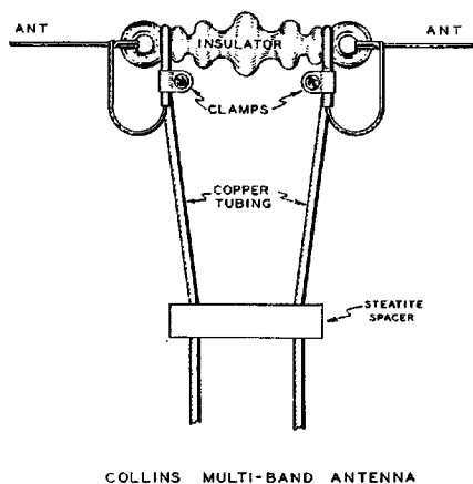
COLLINS MULTI-BAND ANTENNA
