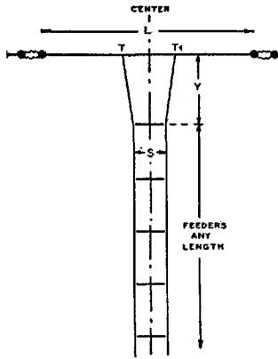
Fig. 31 Two Wire Matched Impedance Antenna System.
