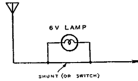
Fig. 15 Lamp Indicator or R-F Meter for Denoting Comparative Output.
