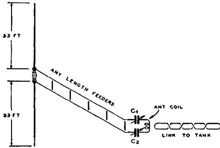
Fig. 30-A 20 and 40 Meter Vertical Antenna with Zepp Feeders. C1-C2 Are .00025 mfd. Condensers.
