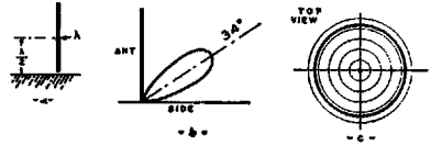
Full Wave Antenna Gives Maximum Radiation Upward at an Angle of 34 Degrees from the Horizon.
