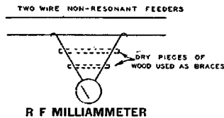
Fig. 32 Method for Locating Standing Waves on Two Wire Non-Resonant Feeder.
