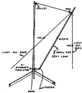
TWO BAND (10-20 METER) TILT ANTENNA — VERTICAL FOR 20 METERS — TILT 54° FROM HORIZON FOR 10 METERS
