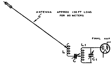
Fig. 33 End Fed Antenna with Series Tuning Circuit.
