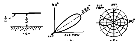
Horizontal Antenna Half Wave Above Ground. This is the best height for horizontal antenna for general use.
