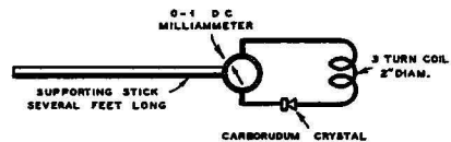
SIMPLE R F FEEDER MEASURING SET
