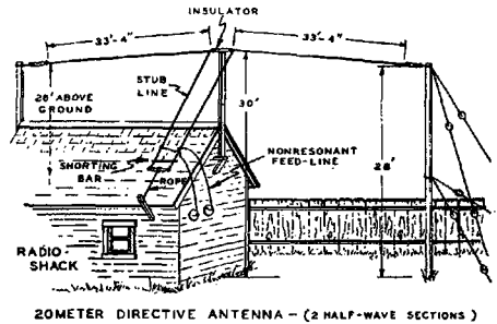
Fig. 23 Pictorial of Fig. 22, Showing Simplicity of 20 Meter Antenna Installation.
