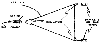
Fig. 122 Triangular Antenna.
