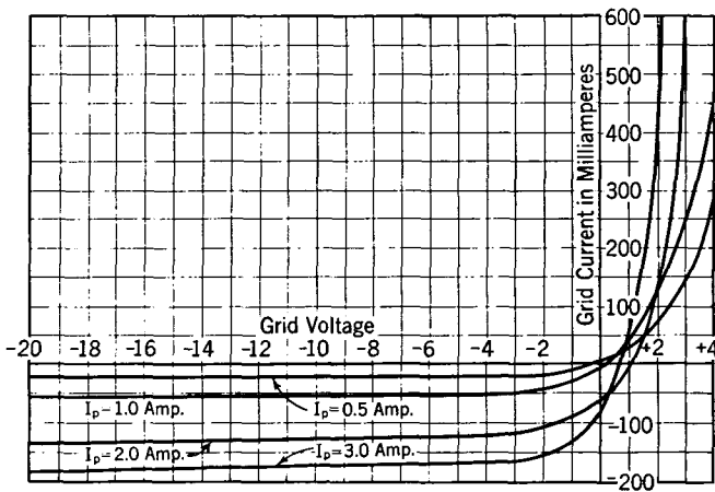
FIG. 62. The grid current after breakdown in a negative-grid, mercury-vapor-filled tube.
