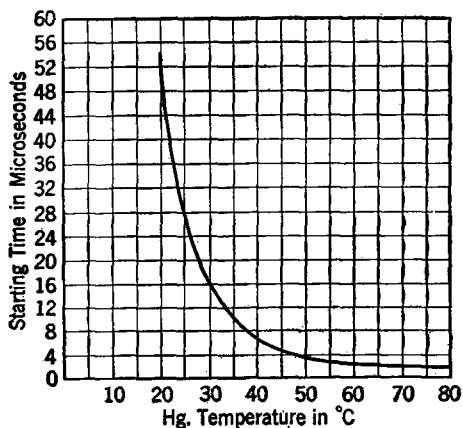
FIG. 54. The time required to establish full conductivity, that is, the "ionization time," and the effect of the mercury-vapor pressure.
