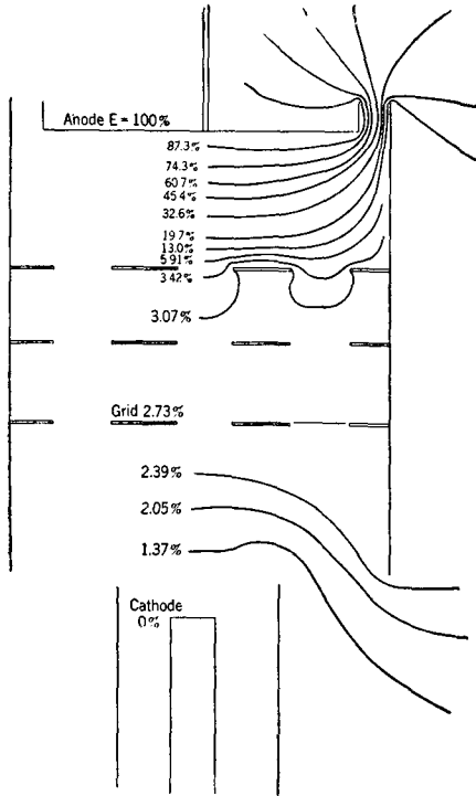
FIG. 57. The potential distribution in a "positive-grid" tube for a combination of electrode voltages which would just cause breakdown.
