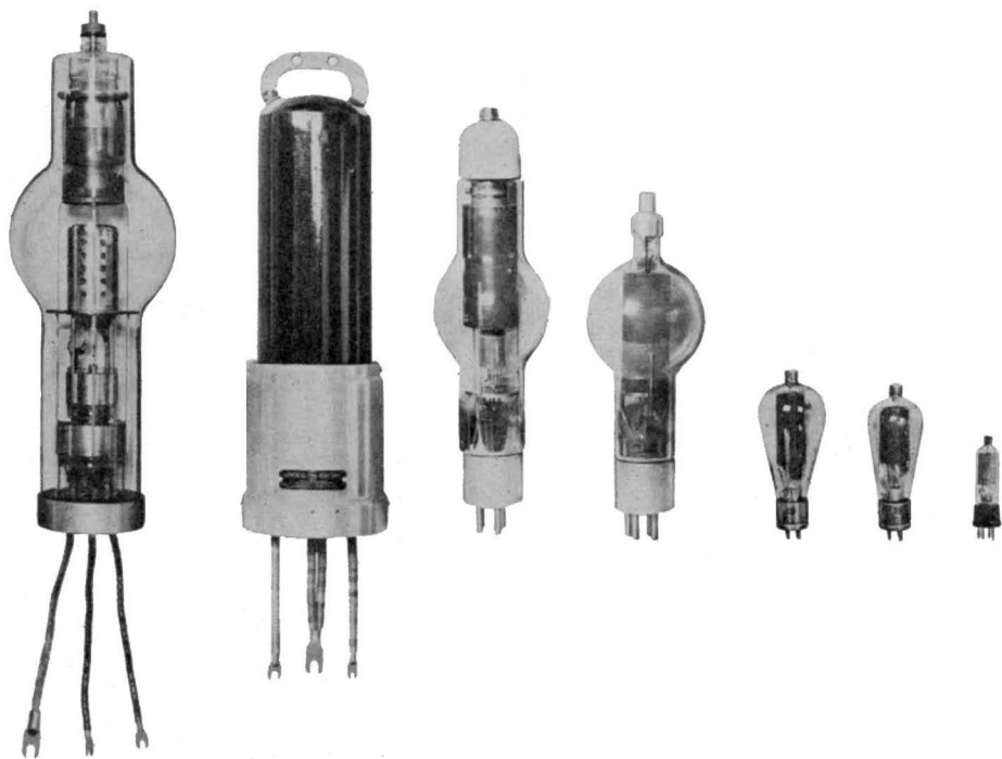
FIG. 6. A group of three-electrode, mercury-vapor-filled tubes. The ratings of these tubes range from 15,000 volts and 75 amperes down to 1,000 volts and 0.125 ampere.
