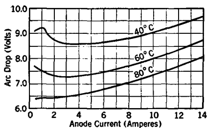
FIG. 49. The effect of load current and mercury temperature on the arc drop.
