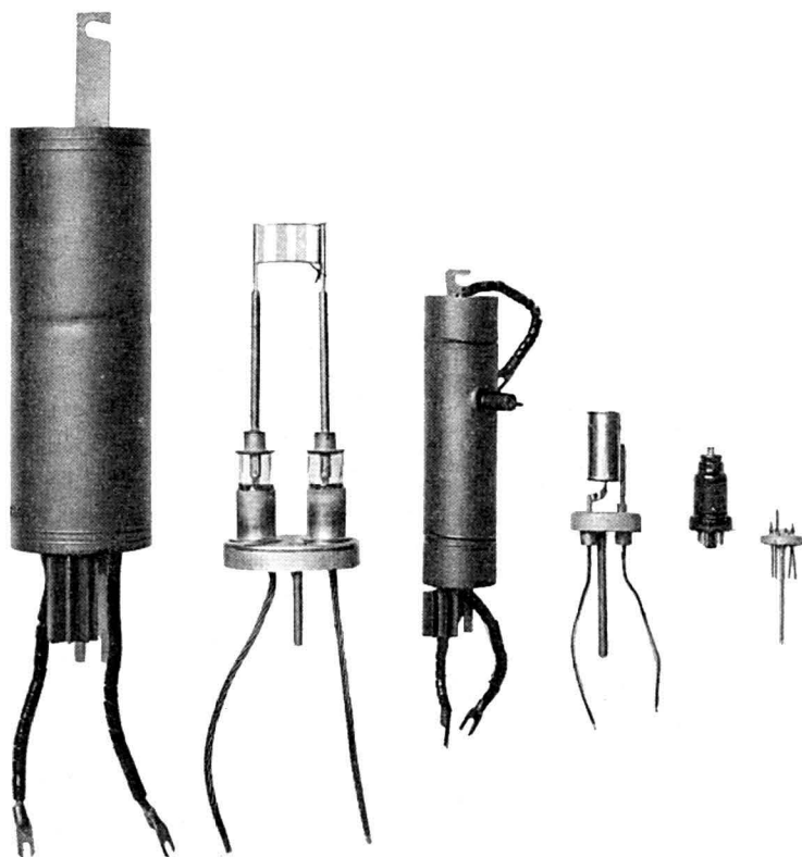
FIG. 86. A group of metal tubes showing the internal structure. At the left is a two-electrode, mercury-vapor tube and cathode header; next, is a shield-grid, mercury-vapor tube and cathode mount and, at the right, a receiving tube and cathode header.
