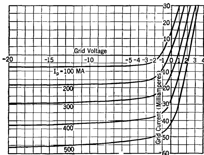
FIG. 64. The grid current after breakdown in a typical argon-filled tube.
