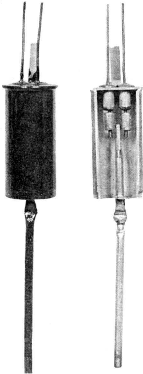
FIG. 83. A single-pole, double-throw vacuum switch.
