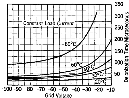
FIG. 53. Relation between grid voltage, mercury temperature, and deionization time for one type of three-electrode tube.
