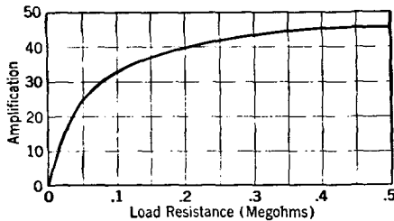
FIG. 44. The calculated gain in a high-vacuum tube amplifier for various load resistors. The tube for which this curve was calculated has a \mu of 50 and a plate resistance of 50,000 ohms.
