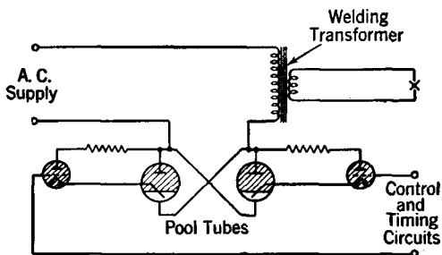
FIG. 81. The use of pool tubes for controlling the flow of alternating current to a welder. The pool tube igniters are energized by grid-controlled, hot-cathode tubes.
