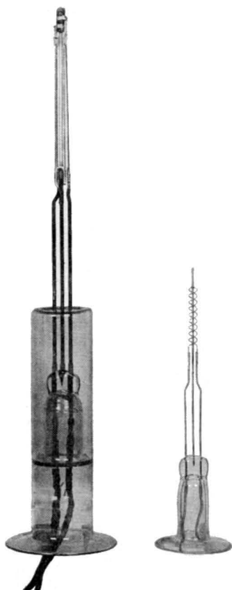
FIG. 3. Typical cathode mounts; pure tungsten filament on the left and a thoriated-tungsten filament on the right.
