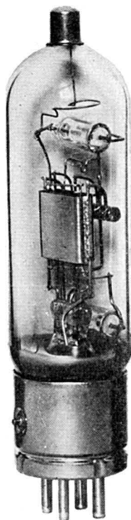
FIG. 38. A low-grid-current, high-vacuum tube.
