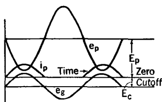
FIG. 40. The current and voltage relations in a high vacuum tube Class B amplifier.
