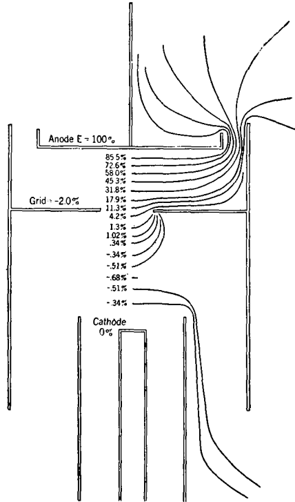
FIG. 58. Potential distribution in a "negative-grid" tube at breakdown.
