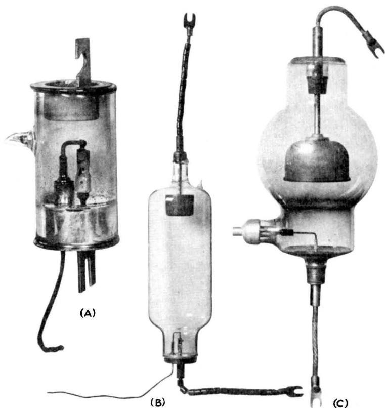
FIG. 70. A group of mercury-pool tubes equipped with immersed ignitors.
