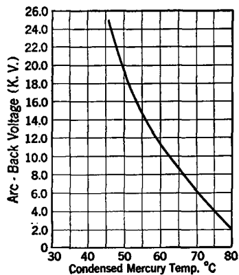
Fig. 51. Curve illustrating the effect of mercury-vapor pressure on arcbreak voltage.
