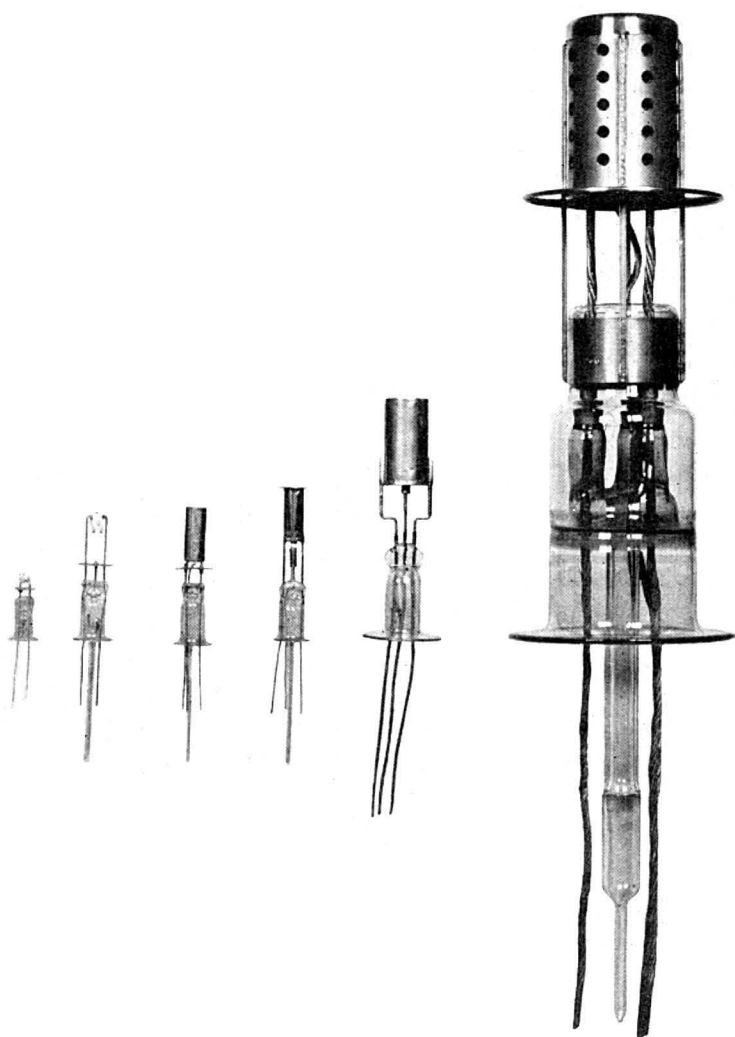
FIG. 4. A group of barium-coated cathodes. The two at the left are coated filaments. The others are indirectly heated, heat-shielded cathodes. The small filament can supply about 2.0 amperes of electron emission. The cathode at the extreme right can supply an electron emission of about 600 amperes.
