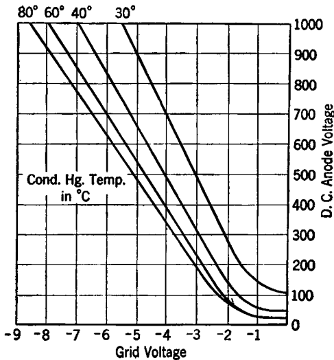
FIG. 56. The critical grid voltage or break-down characteristic of a typical negative-grid, mercury-vapor filled tube. Grid voltages to the left of each curve prevent arc formation whereas those to the right permit full conduction.
