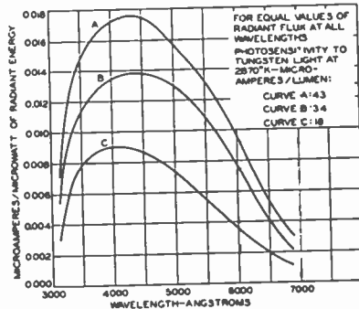
Fig. 3—Spectral sensitivity characteristic of three different 5820's.
