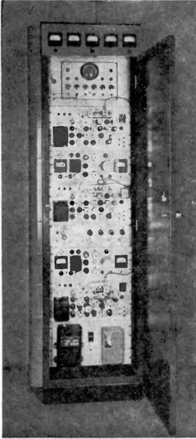
Fig. 5—Television carrier synchronization equipment, receiving station rack.
