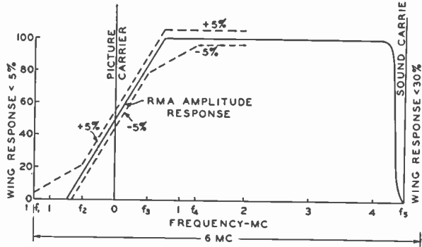
Fig. 12 — Standardization of amplitude characteristic of monitor.
