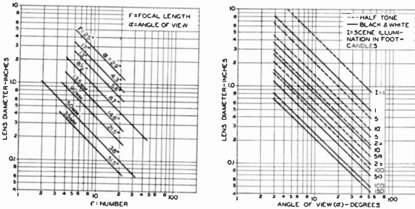
Fig. 5—Illumination requirements for various lens diameters, f : numbers, and angles of view.
