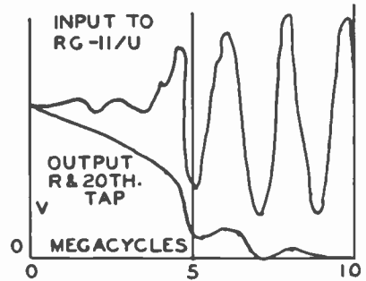
Fig. 9—Same coils as in Figures 7 and 8, but half of the 20 sections bridged, making 10 sections of T -bridged and 10 sections of T .
