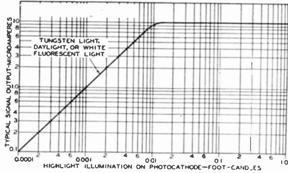
Fig. 4—Typical signal output of type 5820.
