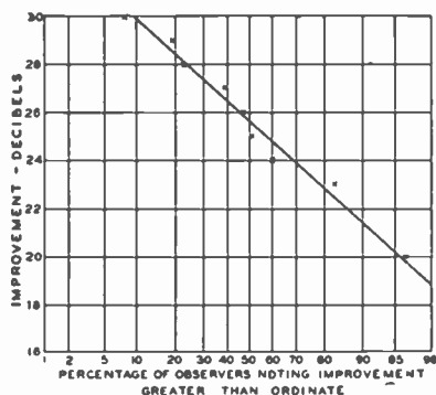
Fig. 7.—Improvement in reception of a television signal in the presence of a cochannel interfering signal. (The improvement factor is that obtained with carriers offset by one-half line frequency, 7875 cycles, with nonsynchronous operation used as a reference standard.)
