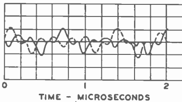
Fig. 9(g) — Cross talk voltage on blue kinescope grid
