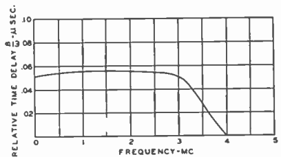
Fig. 15 — Delay characteristic of network for compensation of phase distortion associated with cut-off in receiver.
