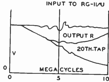
Fig. 6—Same as in Figure 5 except the half-section coils pushed together.
