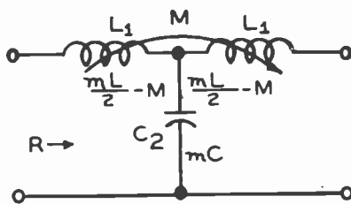
Fig. 1—Constants of the T .
