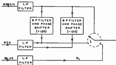
Fig. 21 — Circuit modifications at the transmitter to eliminate cross talk between the red and green channels.
