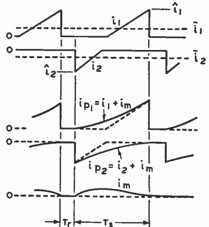
Fig. 5b—Current components in circuit of Figure 5a.
