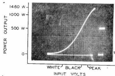
Fig. 20—Modulation characteristics.
