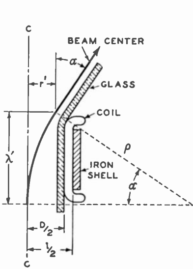
Fig. 2—Geometric relation of kinescope and deflection-coil dimensions to the beam-deflection angle \alpha .
