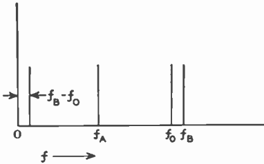
Fig. 2—Frequency relationships in the dot-sequential color television system.
