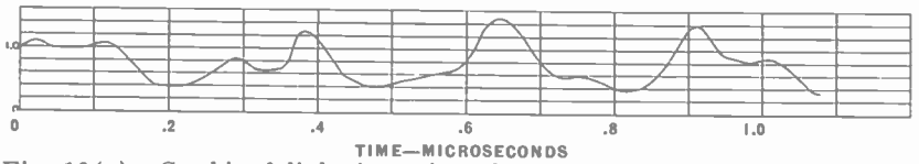
Fig. 10(c)—Combined light intensity of two successive scans of the same line on the green kinescope of a color television receiver.
