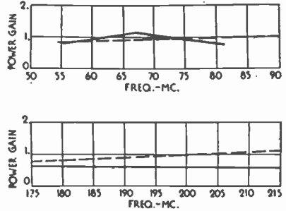
Fig. 9—Power-gain measurements of modified dipole.
