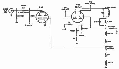
Fig. 7a—Revised video output circuit of Channel 4 receivers.
