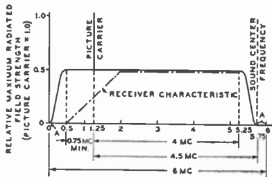
Fig. 1—RMA idealized amplitude characteristics of transmitter and receiver.
