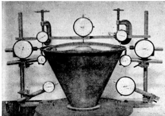
Fig. 3—Pressure deformation test equipment.
