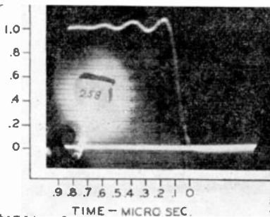
Fig. 19—Square wave response.
