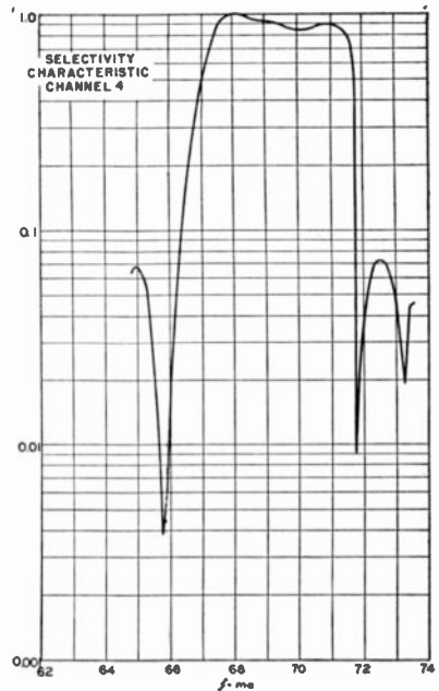
Fig. 22—Frequency characteristic of receiver on Channel 4.
