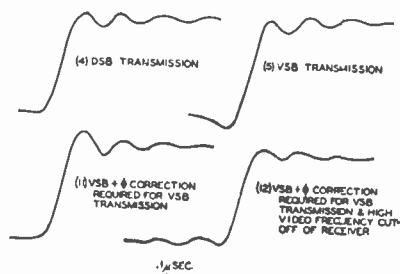
Fig. 7—Television receiver square-wave response.
