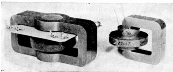
Fig. 14—Autotransformer (right) has higher efficiency and smaller size than transformer with separate secondary winding (left). Both transformers have powdered-iron cores.
