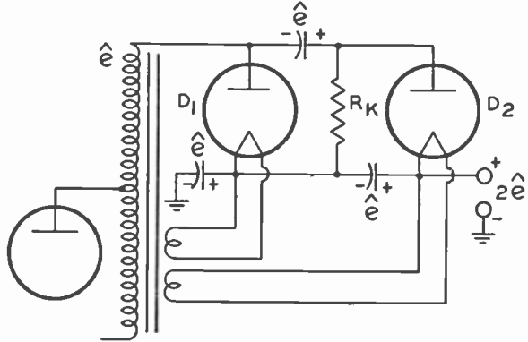
Fig. 11—Voltage-doubling circuit with coupling resistor.
