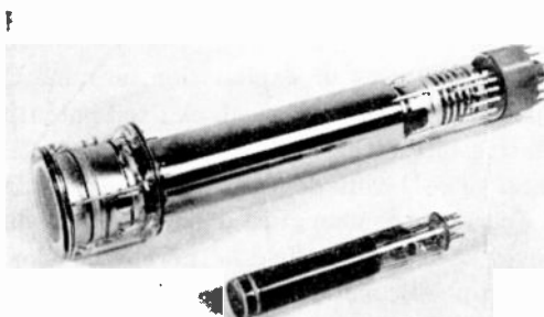
Experimental one-inch-diameter vidicon, with the standard commercial image orthicon in the background.
