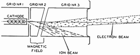
Fig. 5—Single-magnet ion-trap system.
