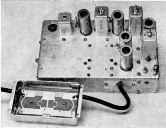
Fig. 4—Photograph of tuner, showing high-pass filter.
