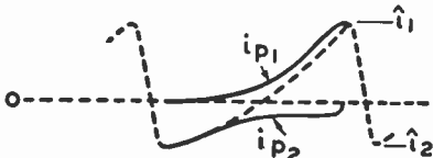
Fig. 5c—Waveform distortion in increasing the average value of i_2 .
