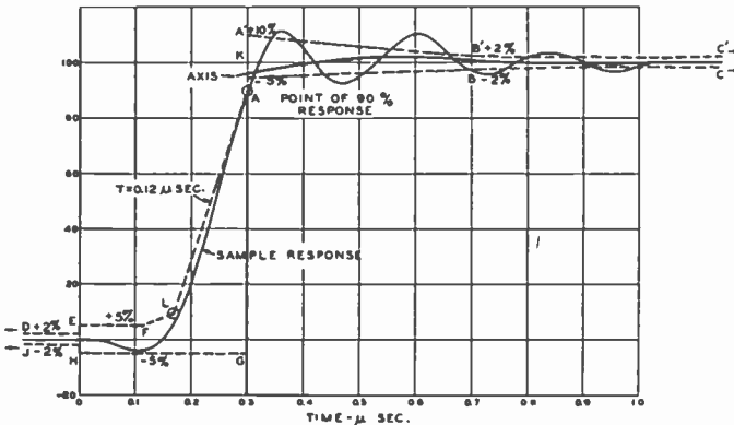
Fig. 13—Standardization of square-wave response of monitor.
