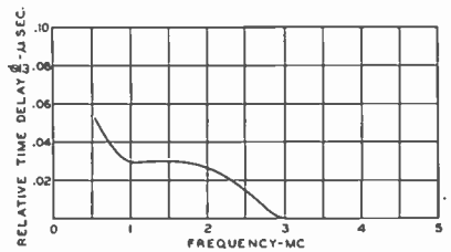
Fig. 5—Delay distortion introduced by VSB transmission.
