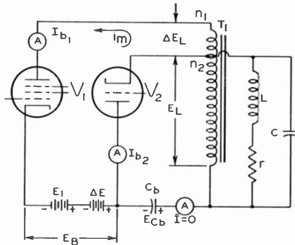
Fig. 6—Power feedback circuit with autotransformer.
