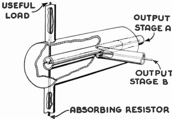
Fig. 11 — A slotted diplexer or bridge which is particularly useful at ultra-high frequencies.
