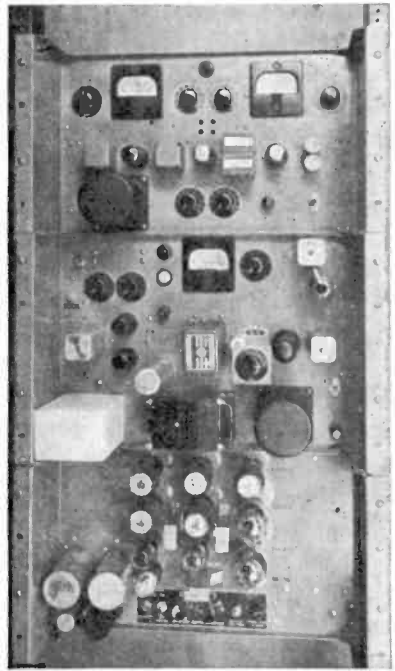
Fig. 6—Television carrier synchronization equipment, transmitter control units.
