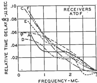
Fig. 8—Delay distortion introduced by VSB transmission.
