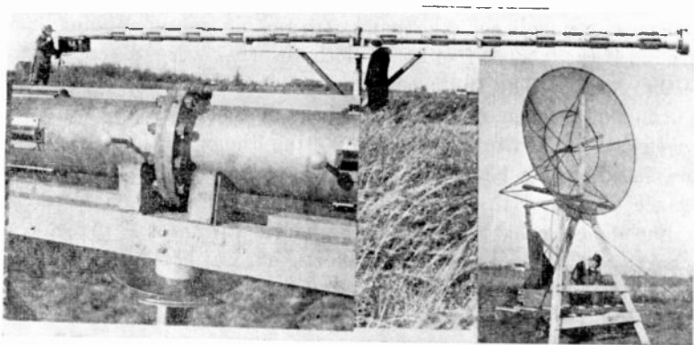
Fig. 7—Vertical pattern test setup for the antenna.
