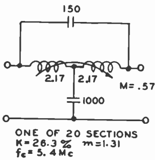
Fig. 6—Same as in Figure 5 except the half-section coils pushed together.
