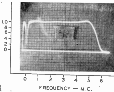
Fig. 17—Modulator video response.
