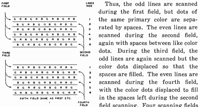
Fig. 6—Scanning and interlace pattern.
