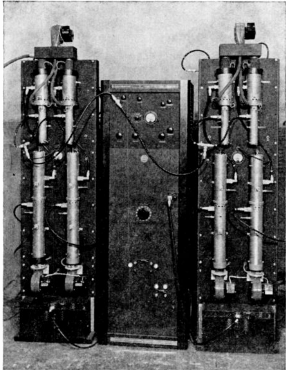
Fig. 13—The experimental 850-mega-cycle television transmitter.
