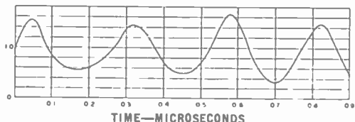
(f) Combined light intensity of two successive scans of the same line, obtained by adding light intensities of the green and red tubes. The sampling frequency is 2.4 megacycles.
