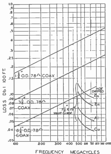
Fig. 17—Curve showing loss of various 7\frac{1}{2} \times 15 -inch wave guides and standard size coaxial lines.
