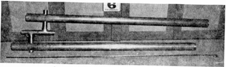
Fig. 26—Notch diplexer photograph.
