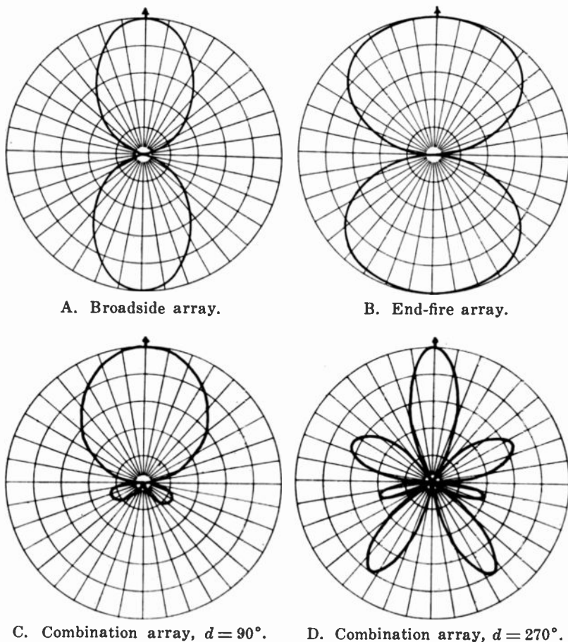
Fig. 2—Relative elevation field patterns.
