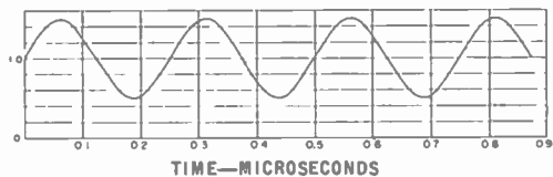
Fig. 30—(a) Signal out of green camera tube; f = 4.0 megacycles, G + g \cdot \sin(\omega t) = 1 + \frac{1}{2} \sin(\omega t) .
