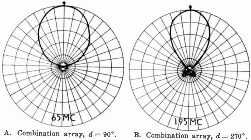
Fig. 3—Relative azimuth field patterns.
