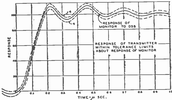
Fig. 14 — Standardization of square-wave response of transmitters.
