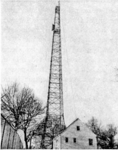
Fig. 6—Transmitter building (side view) and antenna tower. The Channel 4 parabolic receiving antenna can be seen at the 160 foot level of the tower.
