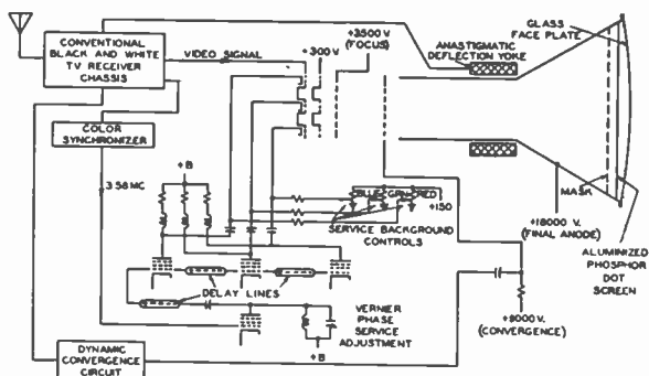
Fig. 1—Block diagram of receiver circuit principles for the three-gun tri-color kinescope.
