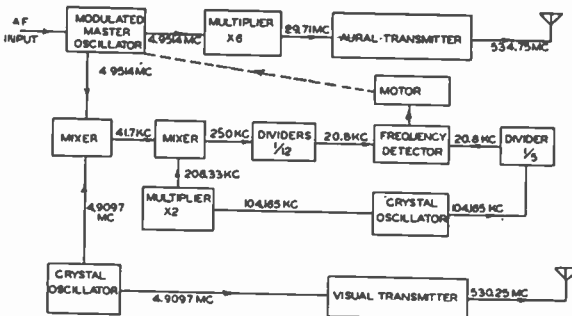
Fig. 14 — Block diagram of frequency control system.
