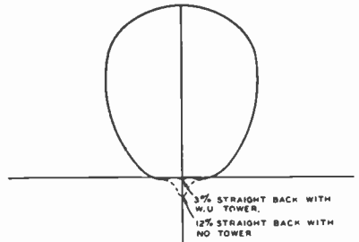
Fig. 4—The relative field patterns in the horizontal plane of the Brandywine receiving antennas.
