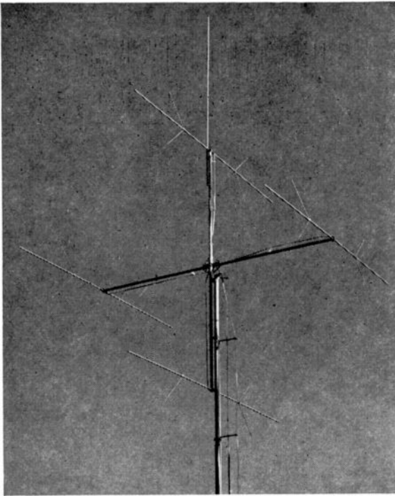
Fig. 11—Reversible-beam array.
