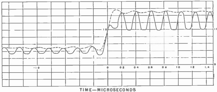
GREEN RESPONSE TO BAND LIMITED STEP FUNCTION SUMS OF SCANS f_o = 2.4 Mc., f_B = 4.1 Mc., f_A = 2.0 Mc.
