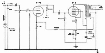
Fig. 7b—Revised audio amplifier circuit of Channel 4 receivers.
