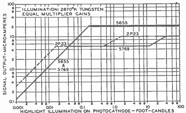
Fig. 8 — Simplified signal output characteristics for image orthicon types 2P23, 5655, and 5769.
