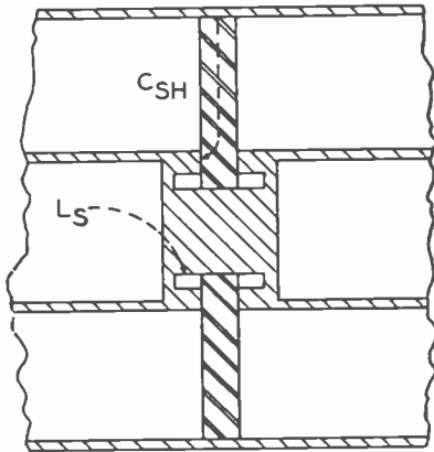
Fig. 11—Section of compensated undercut insulator for 3\frac{1}{2} -inch diameter coaxial line.
