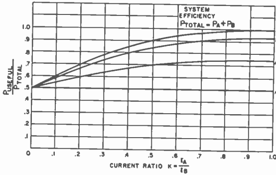
Fig. 3—Power in the useful load in terms of the total power as a function of the ratio of the currents produced by the two generators.
