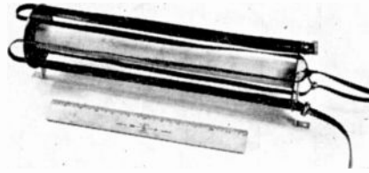
Fig. 12—Diplexer assembly.
