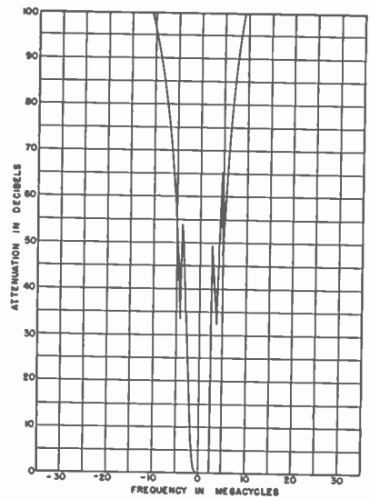
Fig. 10—Overall tuner selectivity curves.
