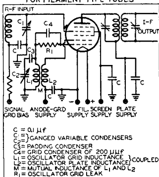
TYPICAL PENTAGRID CONVERTER CIRCUIT FOR FILAMENT-TYPE TUBES
