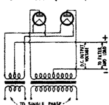
SINGLE PHASE FULL-WAVE RECTIFIER CIRCUIT (TWO TUBES)
