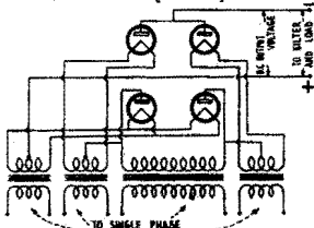
SINGLE PHASE FULL-WAVE RECTIFIER CIRCUIT (FOUR TUBES)
