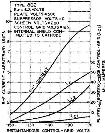
CONTROL-GRID MODULATION CHARACTERISTICS
