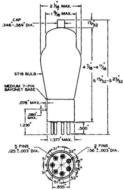
BOTTOM VIEW OF BASE
