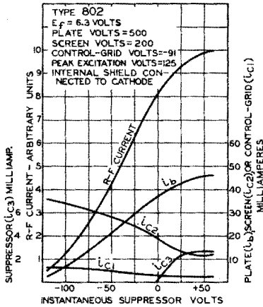
SUPPRESSOR MODULATION CHARACTERISTICS
