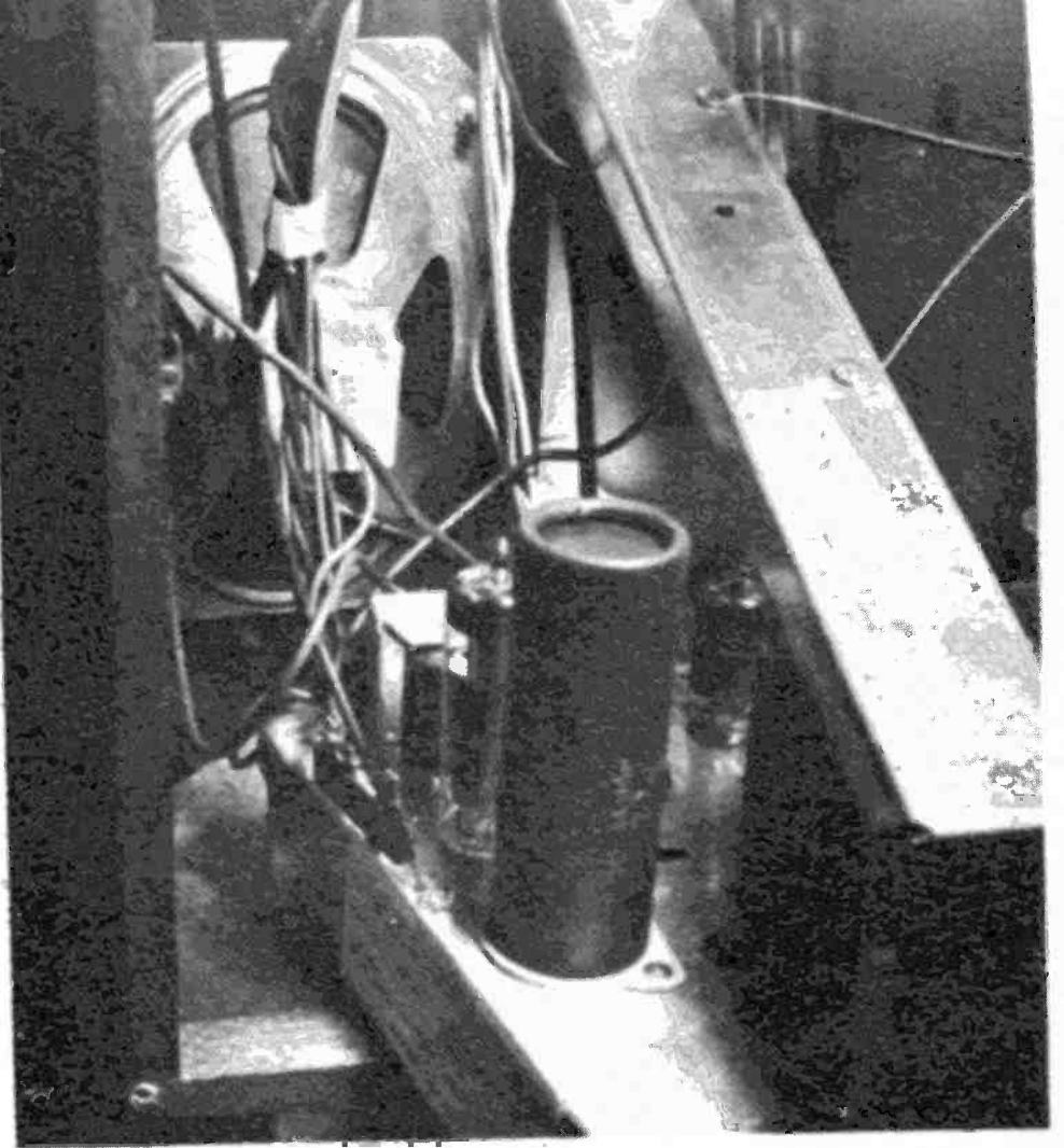
After wires leave the audio output transformer they travel to the speaker mounted in cabinet.
