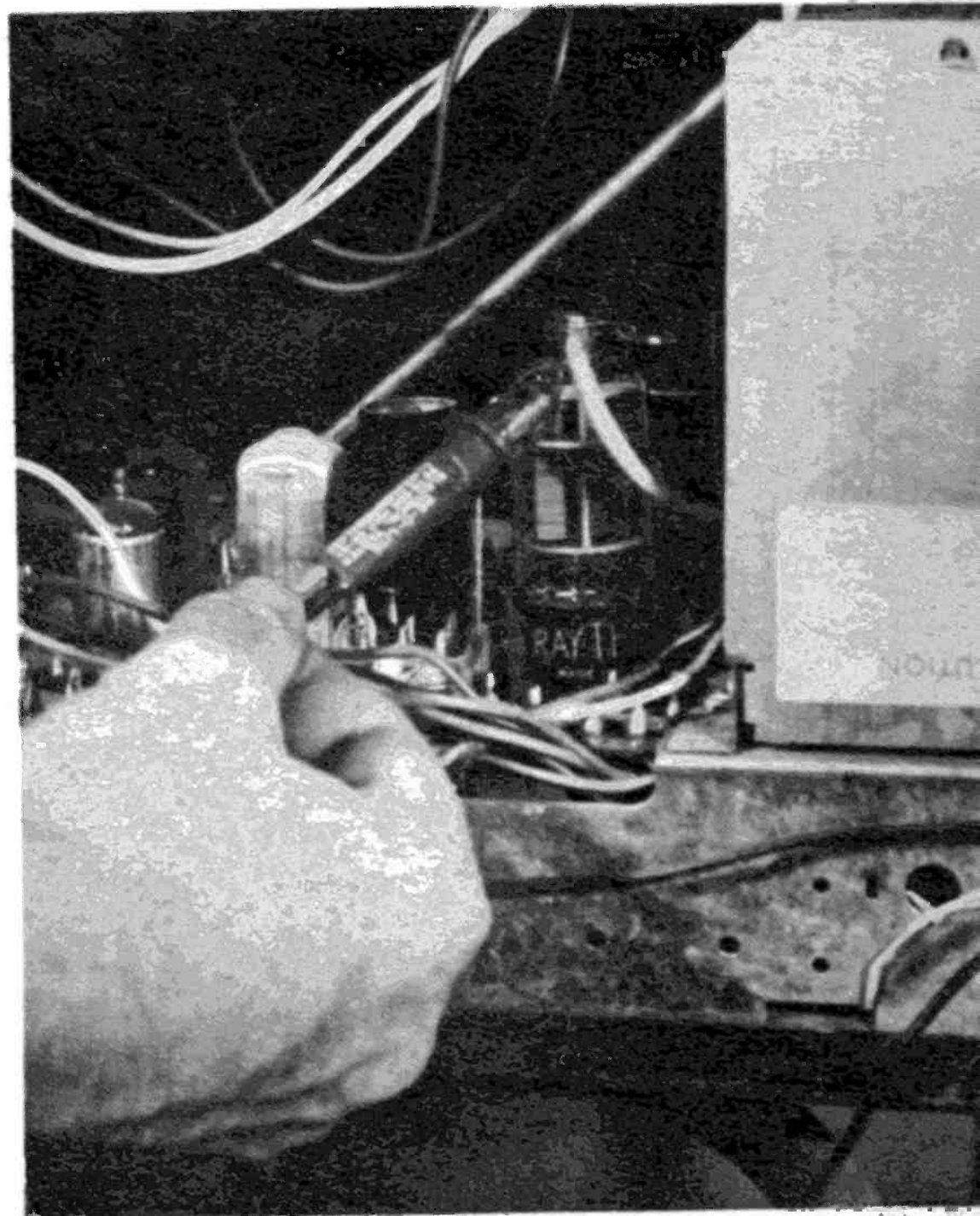
A safe and easy way to test for the presence of high voltage is to place a neon tester in here.
