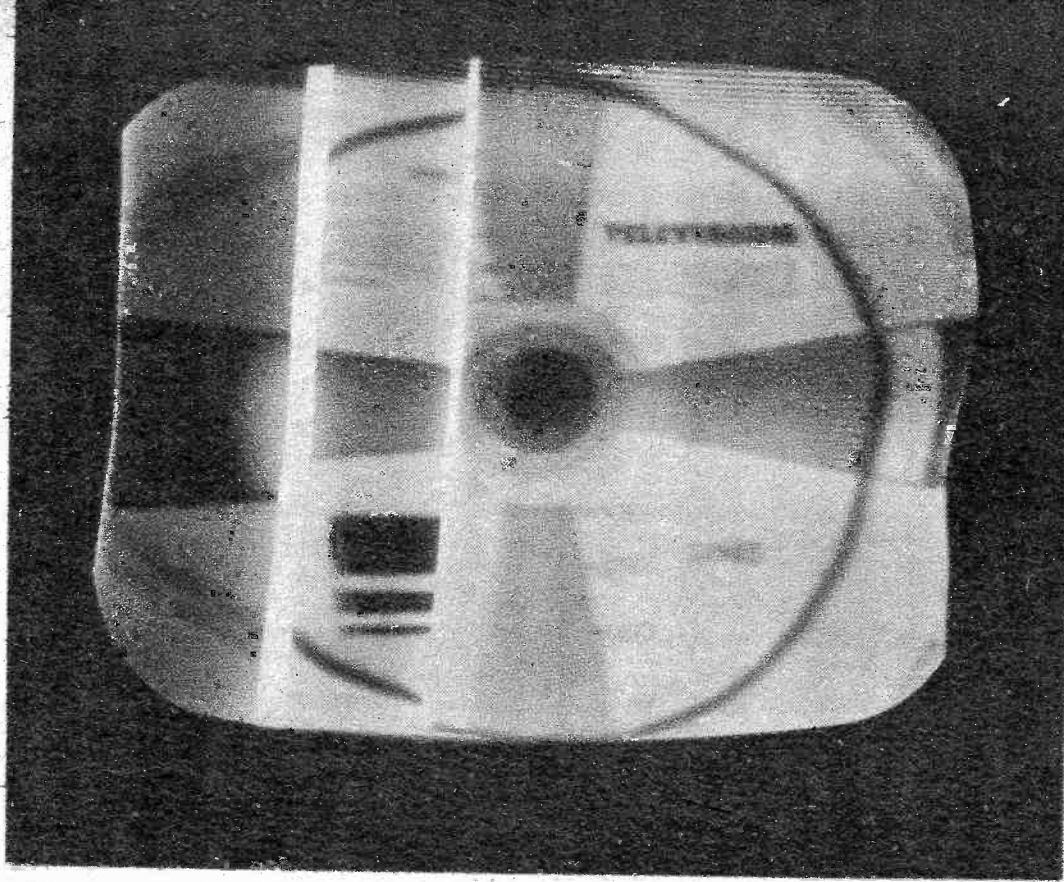
POOR HORIZONTAL LINEARITY: The main reason for this condition is a weak DAMPER tube. Also check HORIZONTAL OUTPUT , HORIZONTAL DRIVE CONTROL , HORIZONTAL LINEARITY CONTROL or WIDTH CONTROL . Lastly, try the HORIZONTAL OSCILLATOR and HORIZONTAL PHASE DETECTOR (see Chapter 8).
