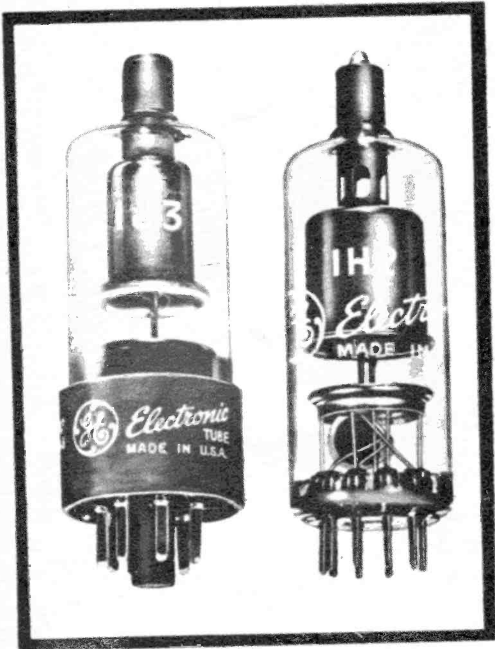
Typical high voltage rectifier tubes have heavy duty caps on tube top to pass the high voltage.
