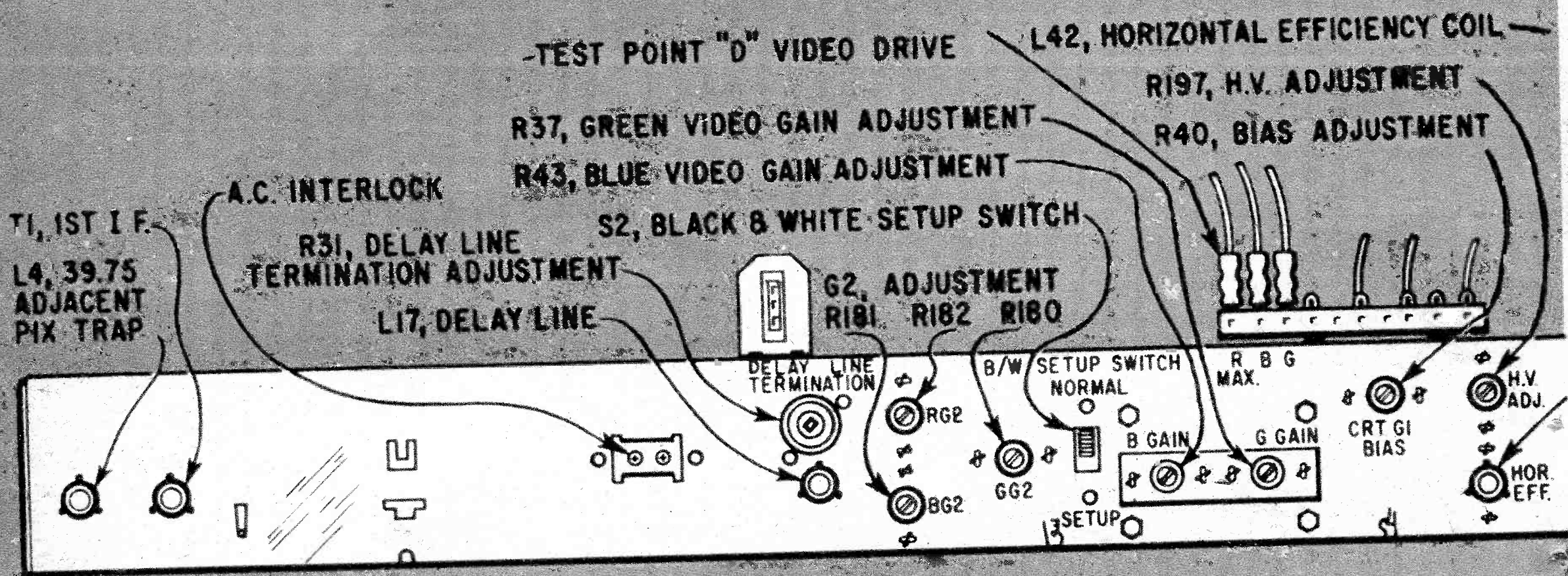
A diagram with information for adjustments is a valuable adjunct to round out a tube location guide.
