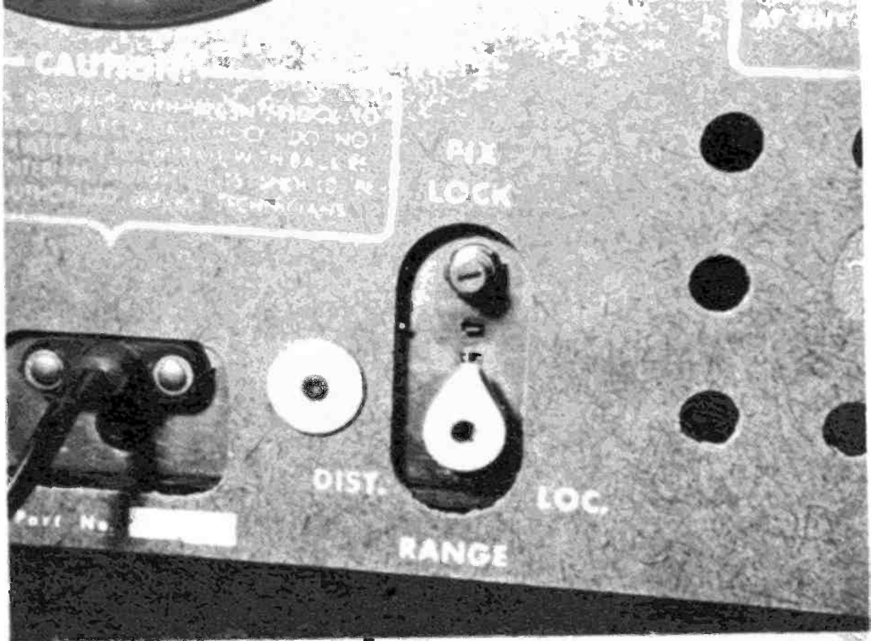
The local-distance switch is a variation of an AGC control. It turns the RF amplifier on full.
