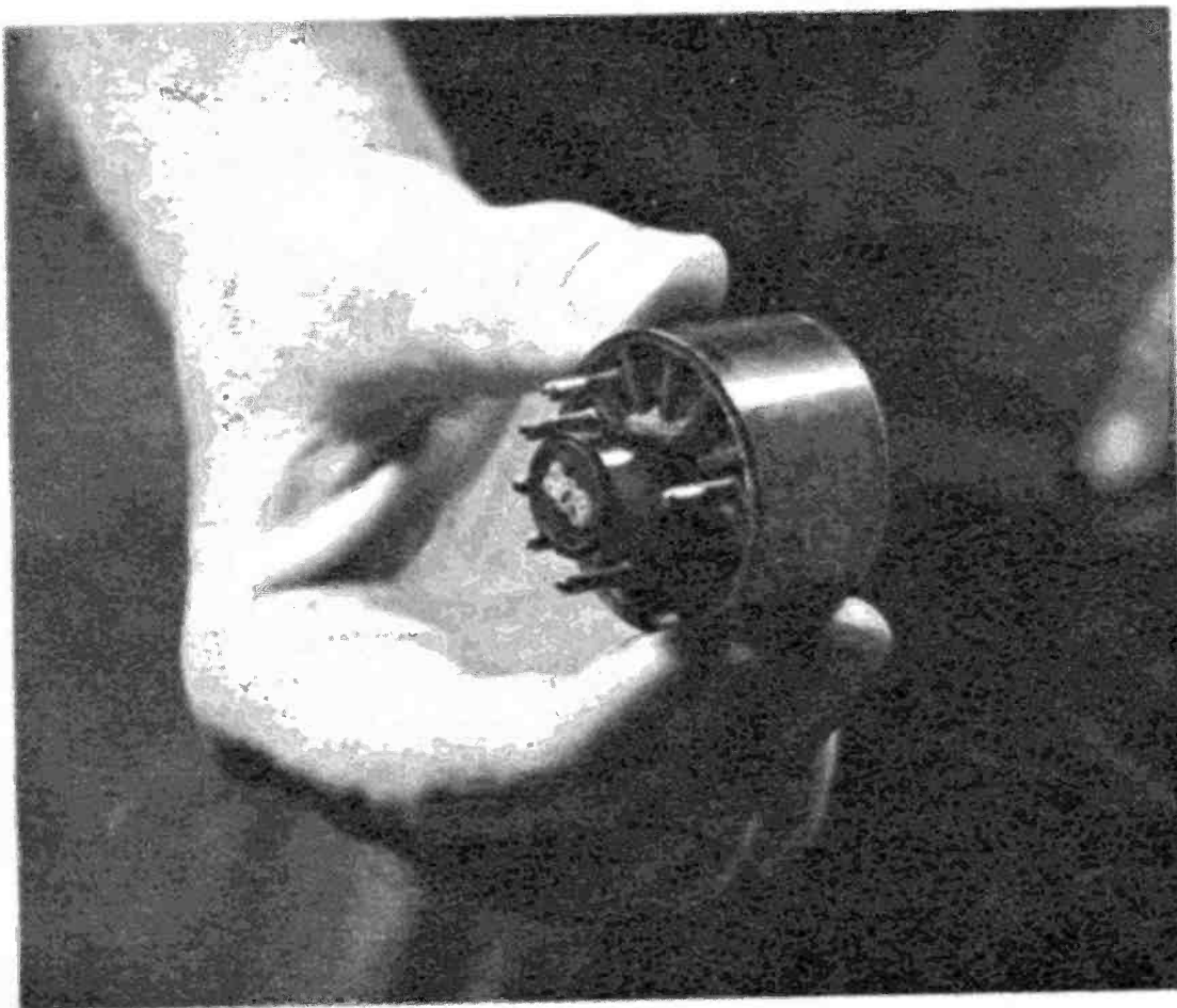
When the plastic socket comes off the neck of the tube you can rethread and solder it back on.
