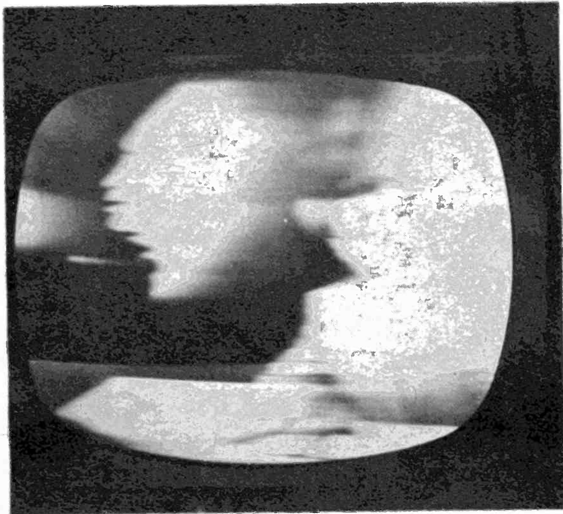
A bad peaking coil stops the video amplifier from passing the full 4.5 MC range, and causes smear.
