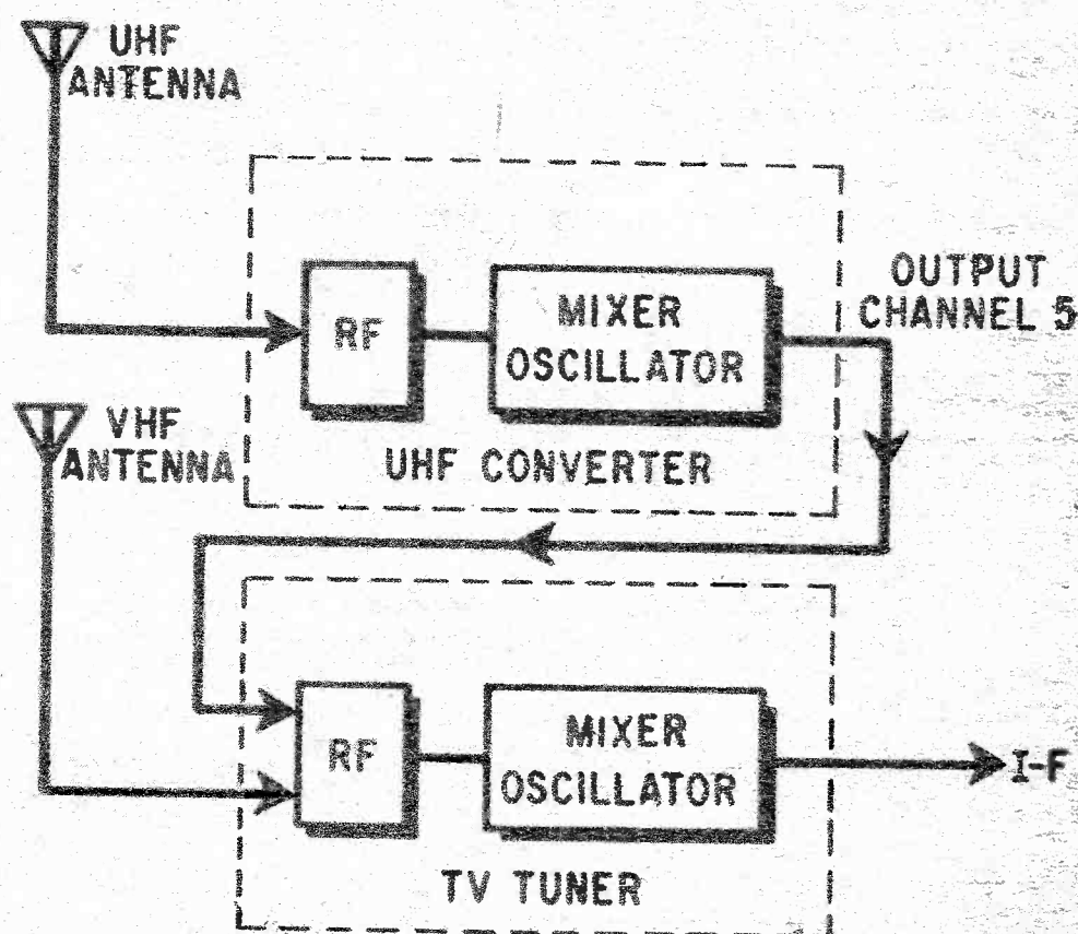
HOME INSTALLED UHF CONVERTER
