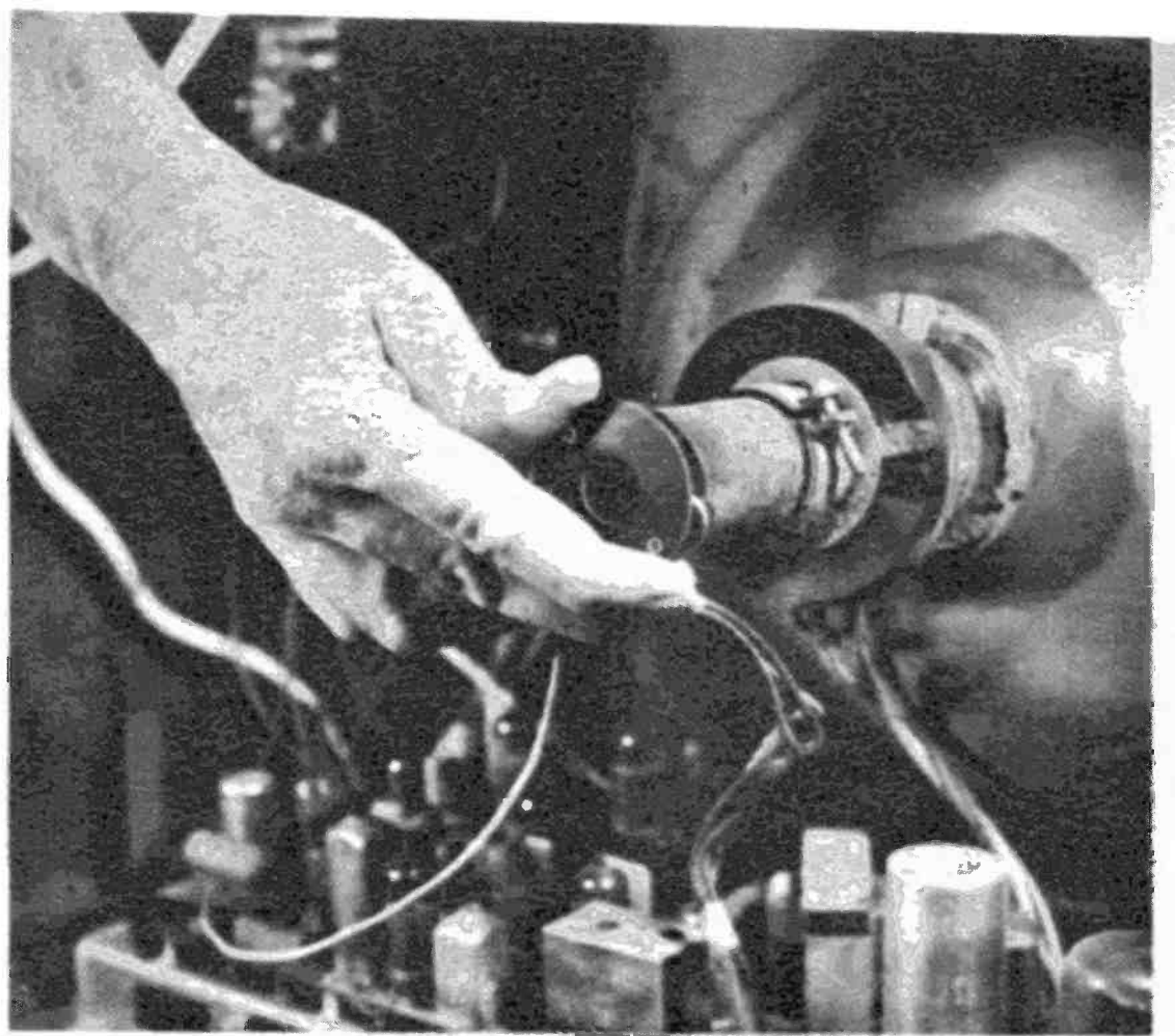
A visual check of the way the heaters are lighting will sometimes reveal valuable service clue.
