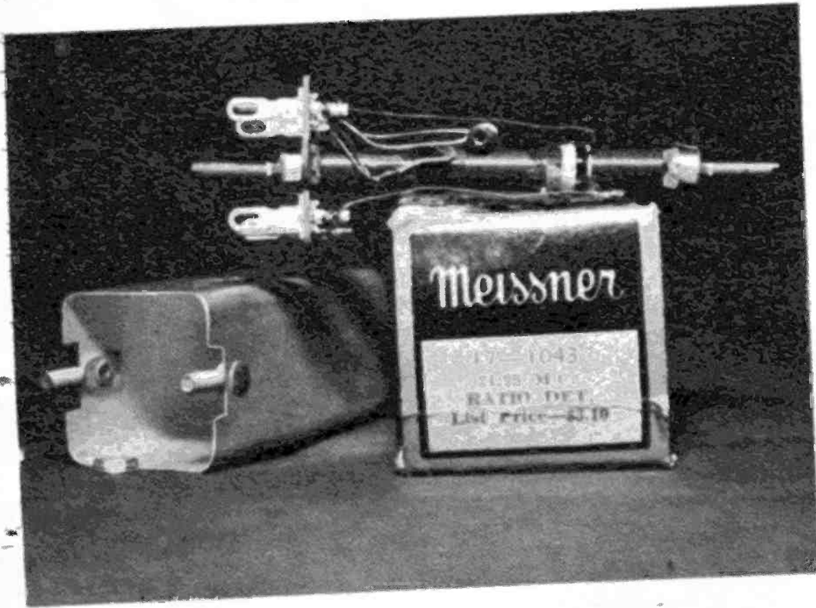
A detector can has adjustment spots on the top and the bottom. They can easily be tuned by ear.
