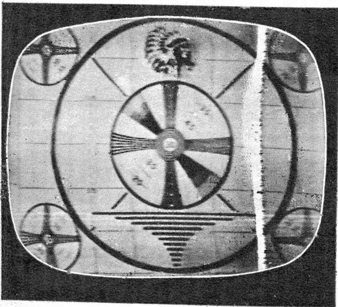
POOR HORIZONTAL LINEARITY: The main reason for this condition is a weak DAMPER tube. Also check HORIZONTAL OUTPUT , HORIZONTAL DRIVE CONTROL , HORIZONTAL LINEARITY CONTROL or WIDTH CONTROL . Lastly, try the HORIZONTAL OSCILLATOR and HORIZONTAL PHASE DETECTOR (see Chapter 8).
