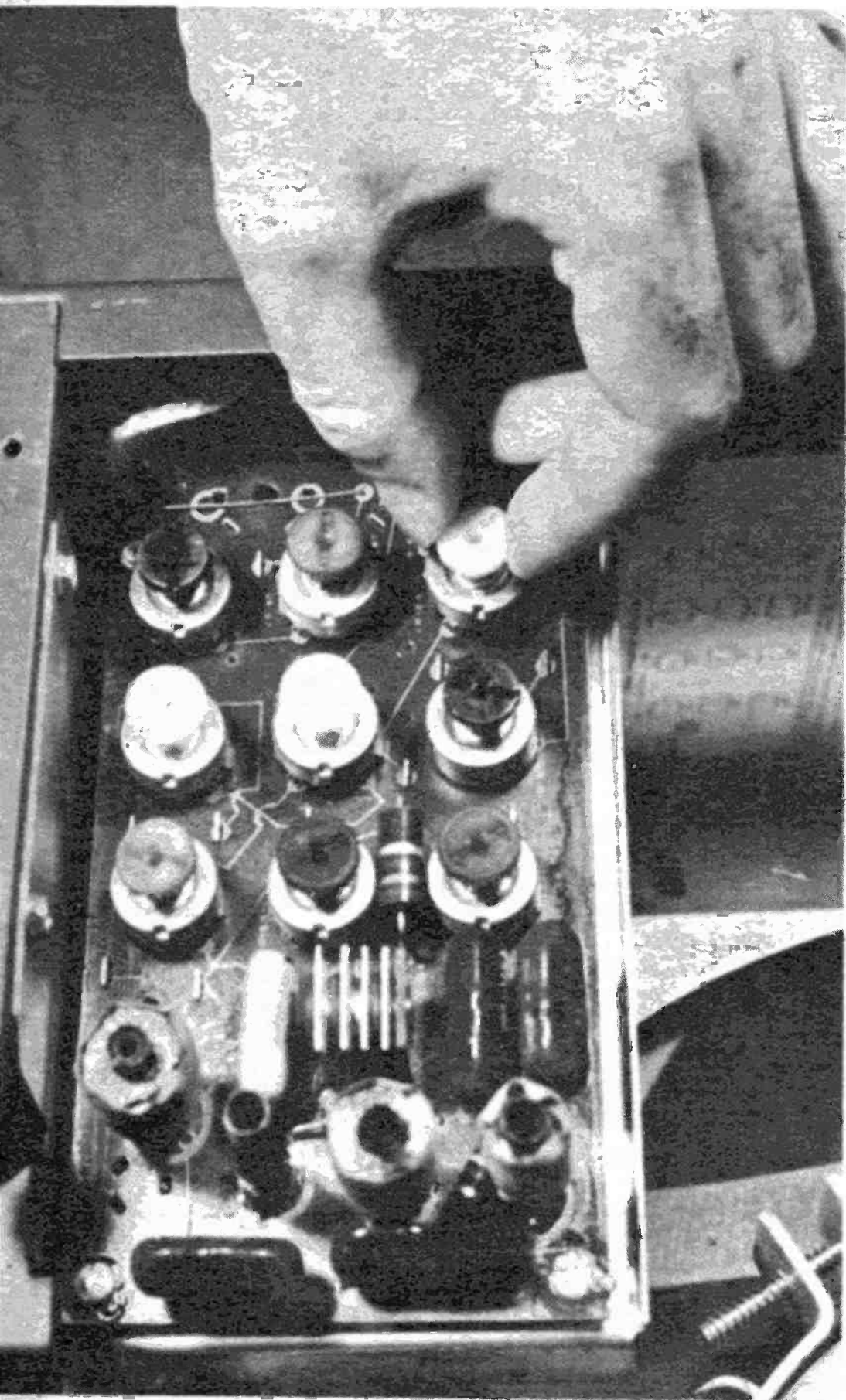
Nine of the convergence adjustments are conducted by hand. All knobs rotate 360 degrees.
