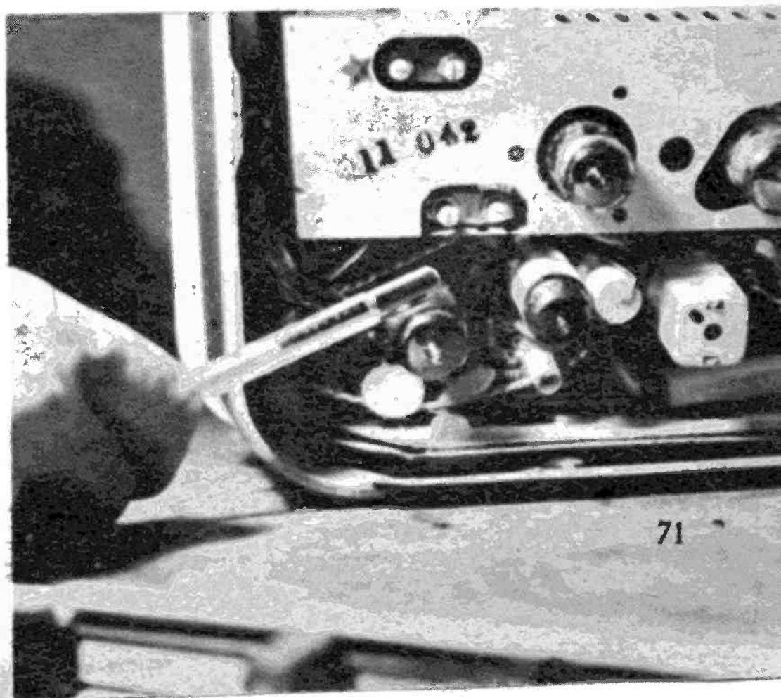
An easy way to test for a bad sound tube is to tap it gently. Bad ones will ping or crackle.
