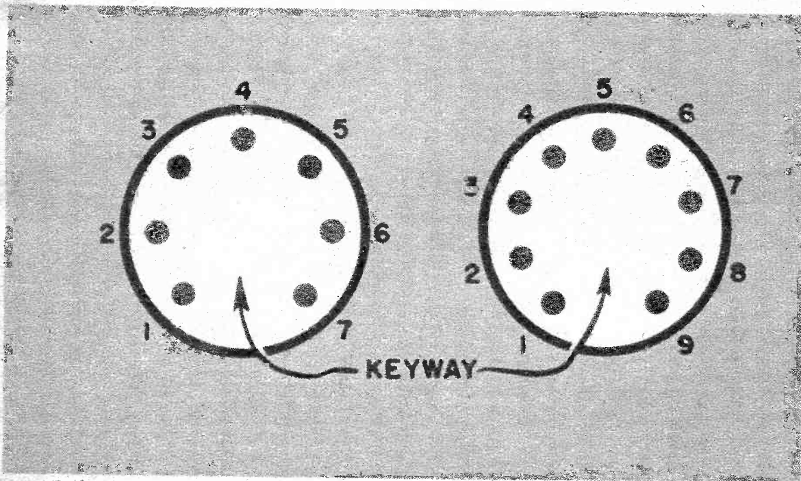
In the miniature type of tubes the keyway takes the form of a space. Count pins from the left.
