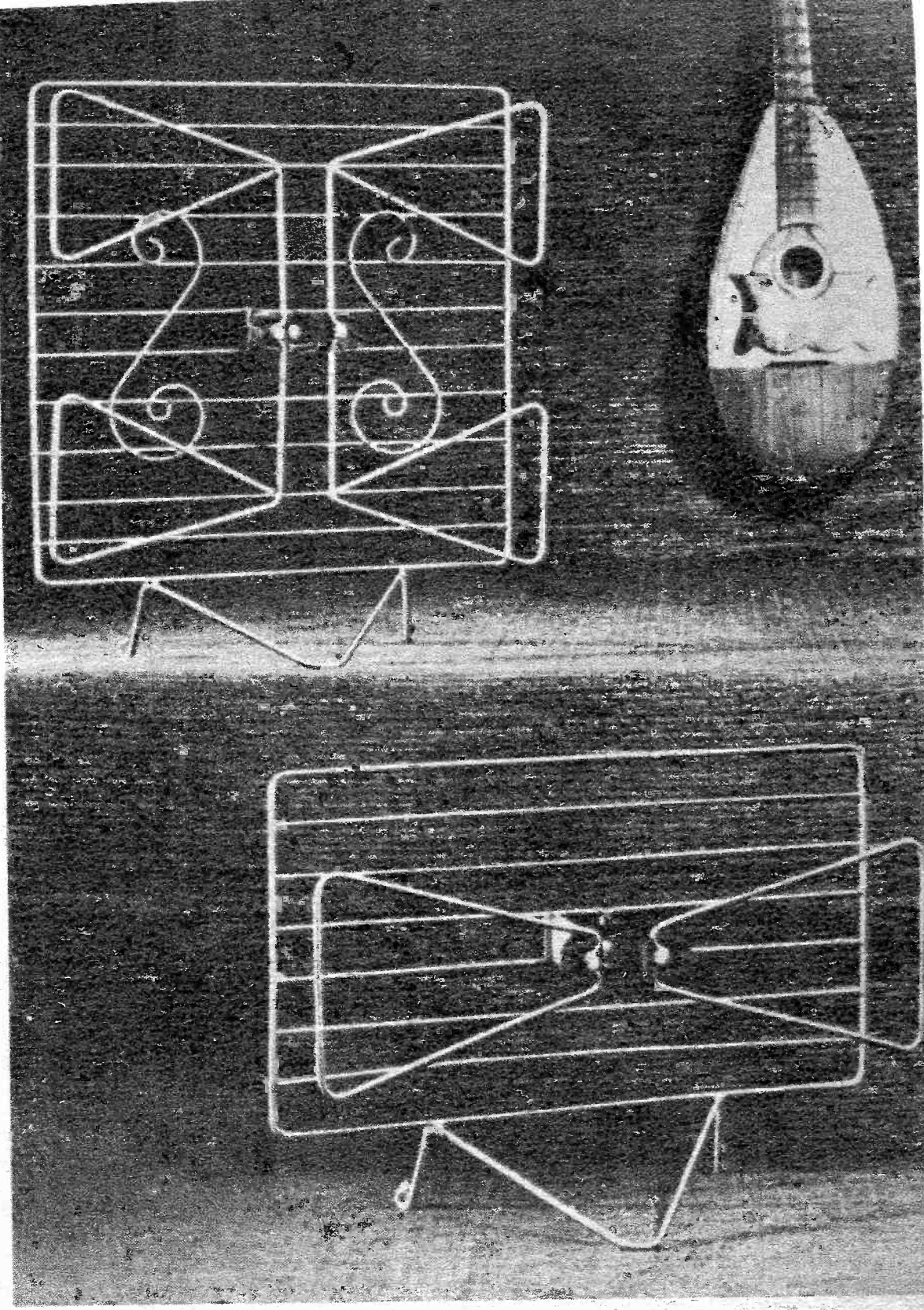
There are many forms of UHF indoor antennas. The decorative shapes, above, are half wave antennas.
