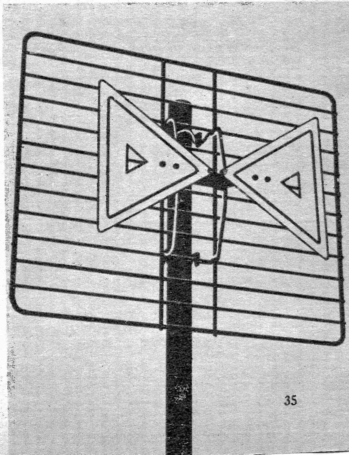
In shape of a bowtie, this is actually a half wave conical antenna, made solid between the elements.
