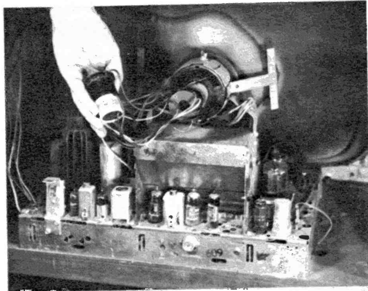
The most common CRT trouble of low brightness can be fixed quite often with a brightener.
