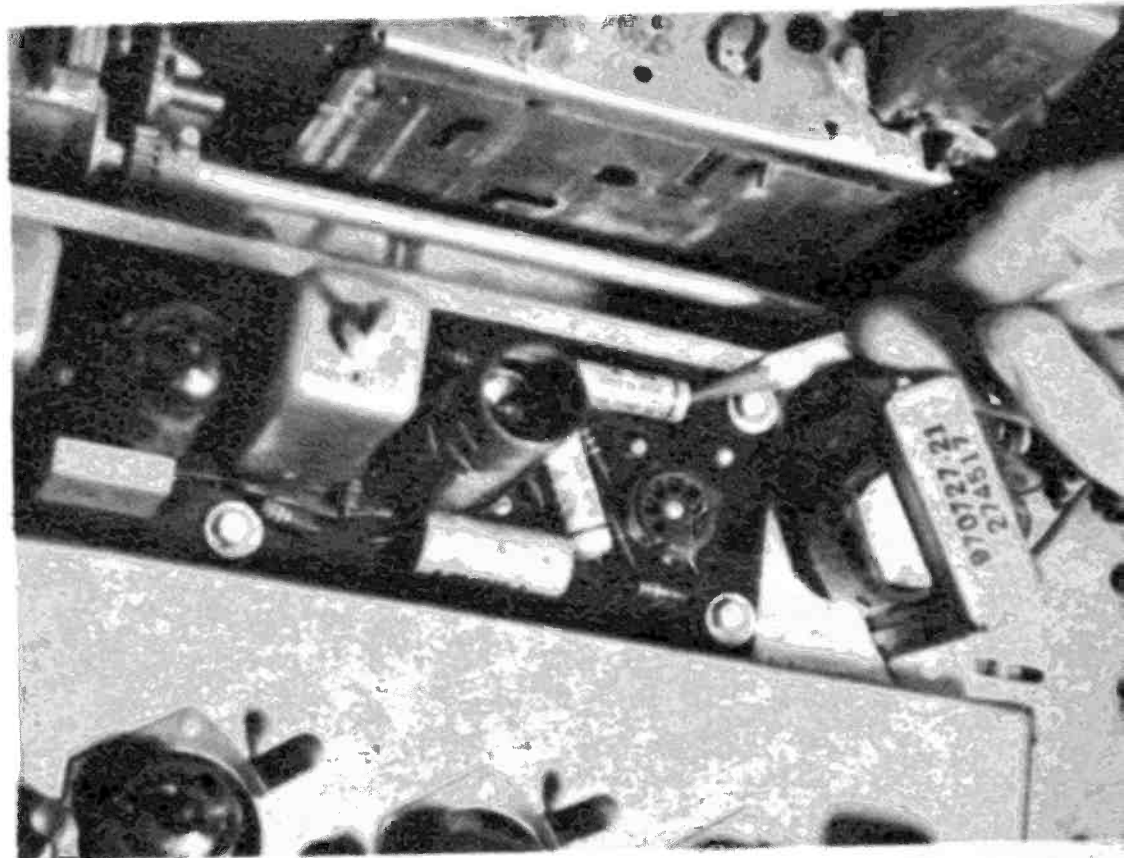
An easy way to test for a bad sound tube is to tap it gently. Bad ones will ping or crackle.
