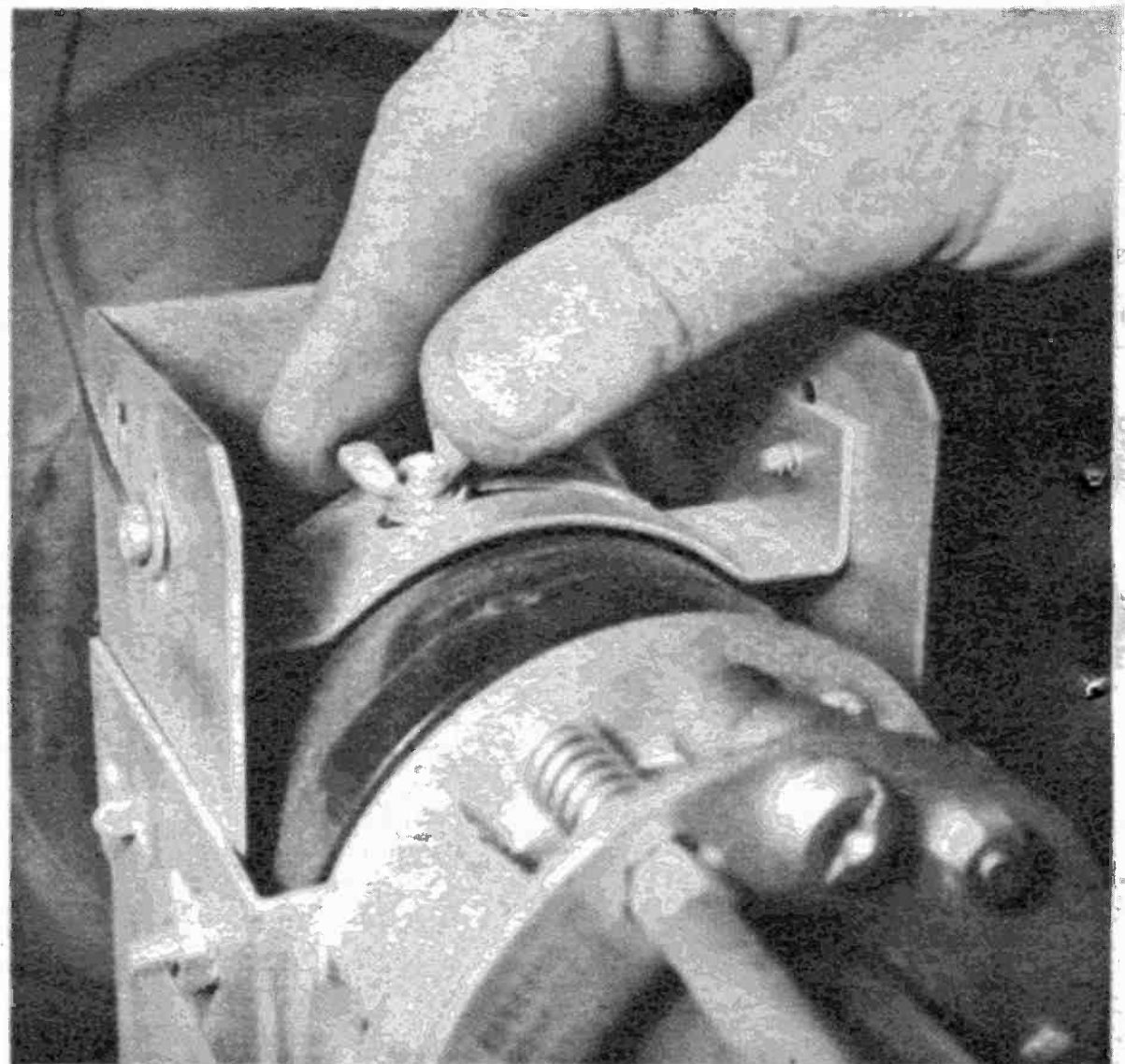
Some yokes have wing nuts on the top of center. Loosen nut and swing yoke for a tilted picture.
