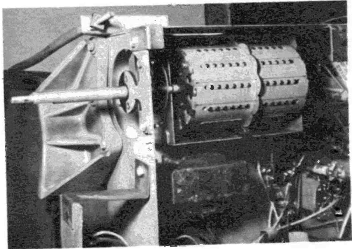
Above is a common type tuner with the channel strips exposed. Springs hold strips in place.
