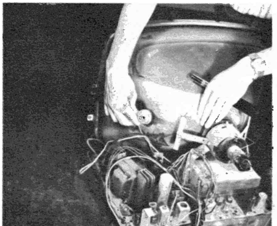
A professional tests for correct value of high voltage at CRT well during picture tube repair.
