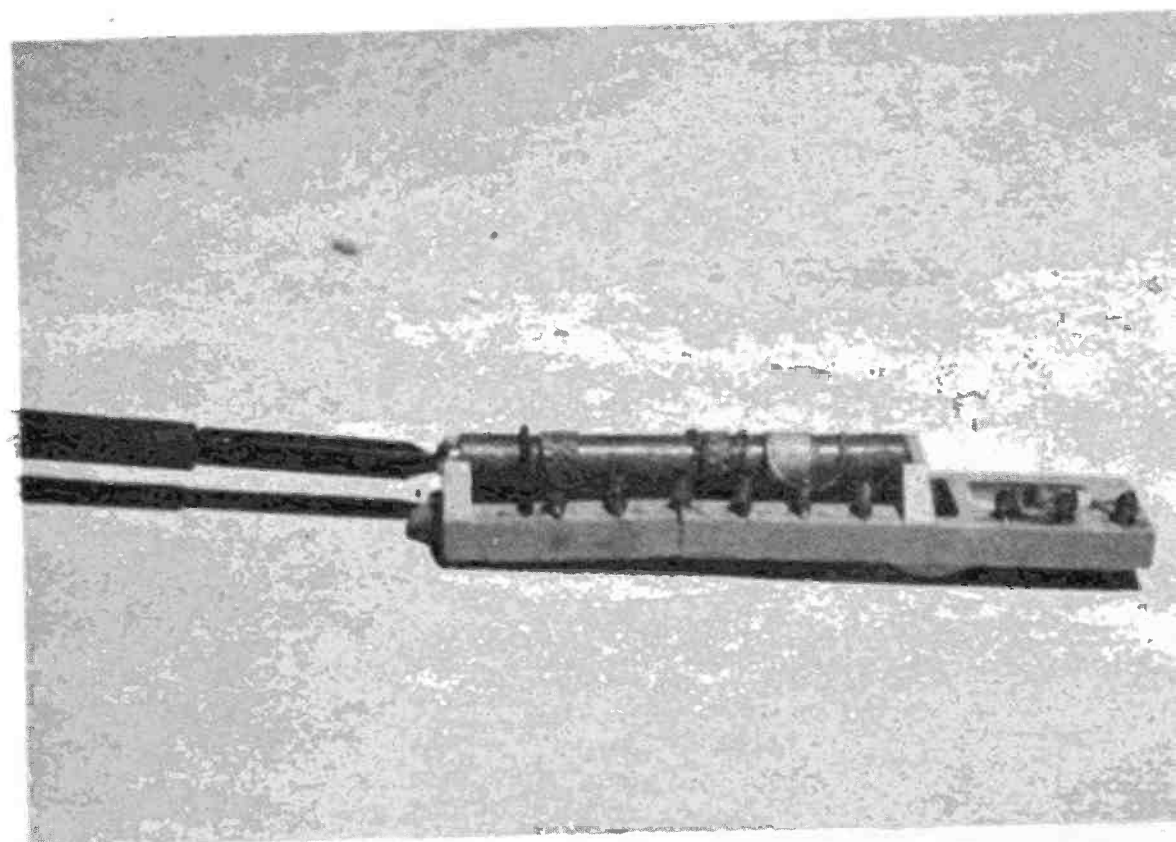
This is what happens inside the tuner when you insert a screwdriver and adjust the oscillator.
