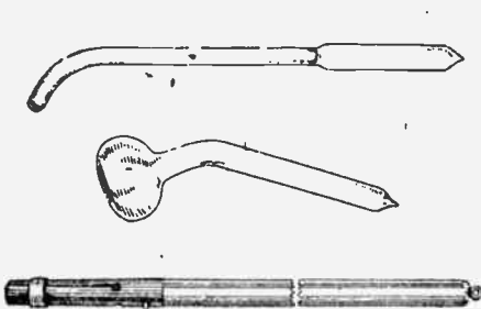
Some Typical High Frequency Electrodes
