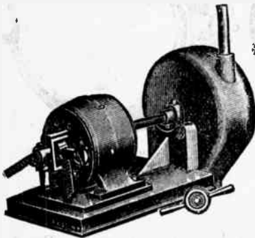
Fig. 11. Water motor direct connected to dynamo.
