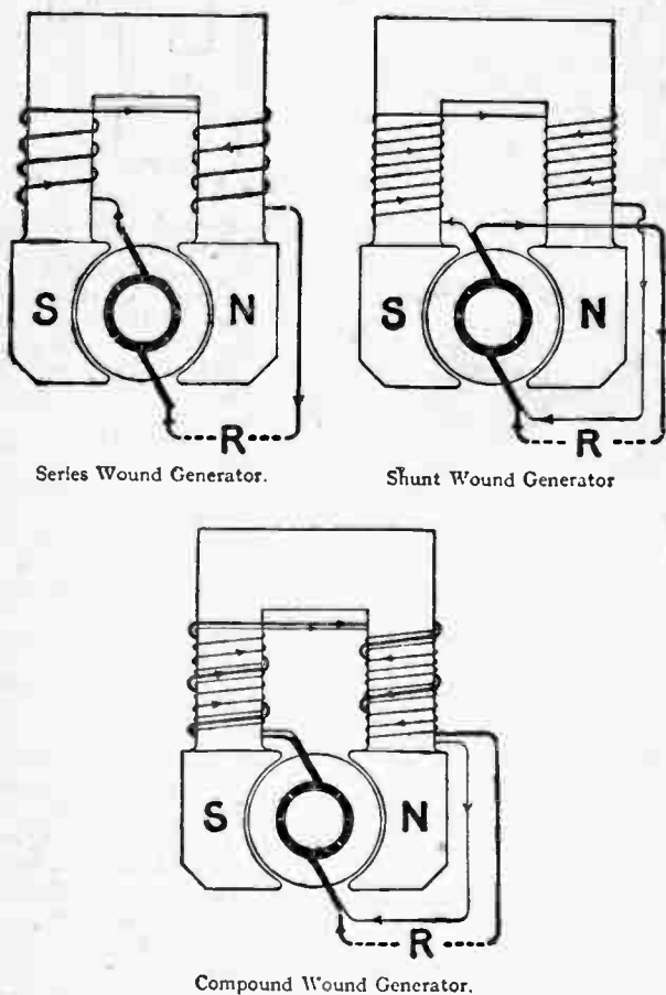
Compound Wound Generator.
