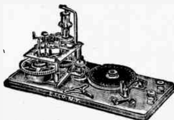
Omnigraph with Spring Motor.
