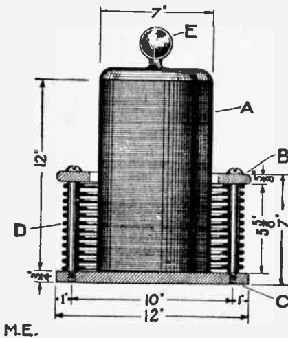
An Oudin Coil.
